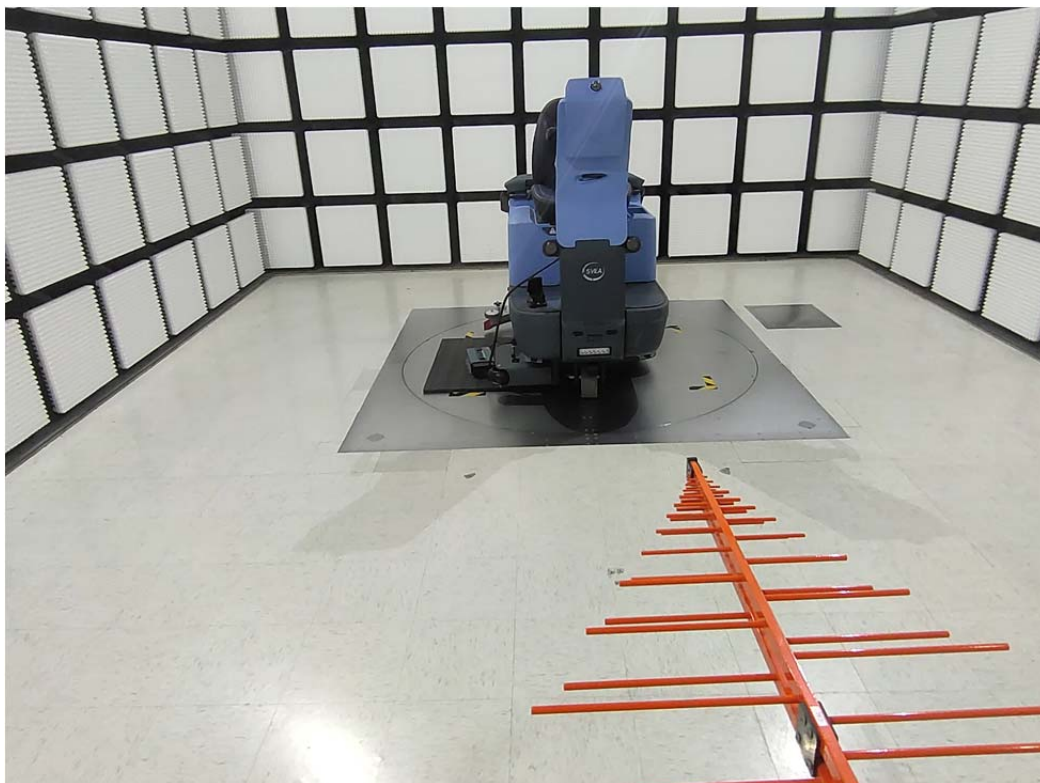
Radiated Emission 30 MHz-1 GHz View
