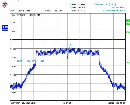
g_2442MHz_Chain 0 -8.59dBm/3kHz
