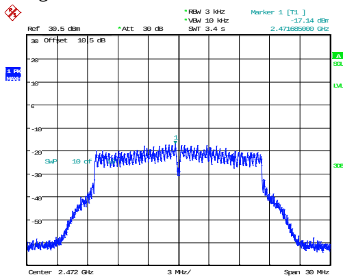
g_2472MHz_Chain 0 -17.14dBm/3kHz
