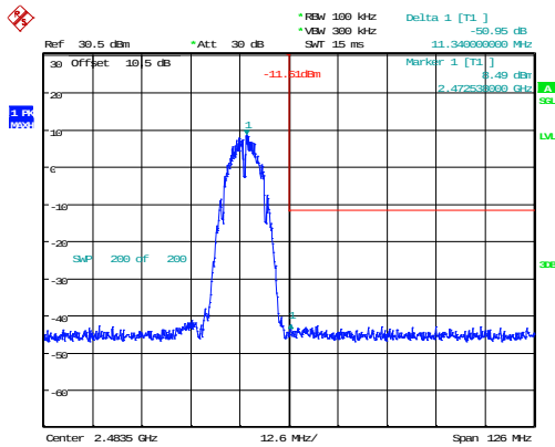
b_2472MHz_Chain 0 50.95dB
