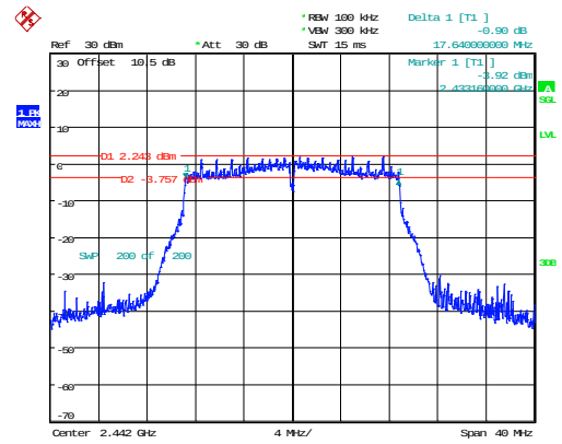
n20_2442MHz_Chain 0 17.640MHz
