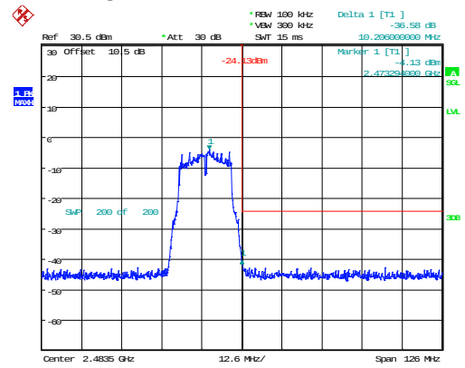
g_2472MHz_Chain 1 36.58dB
