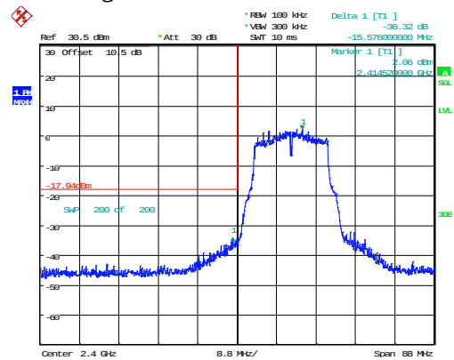
g_2412MHz_Chain 1 36.32dB
