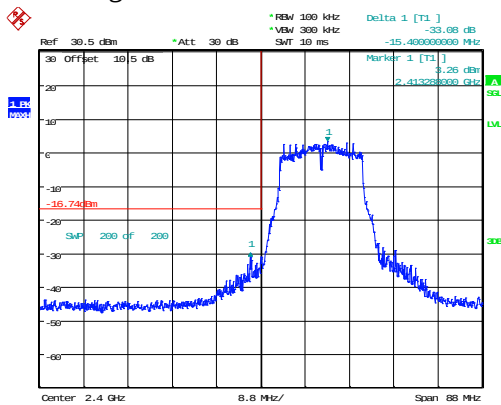
g_2412MHz_Chain 0 33.08dB
