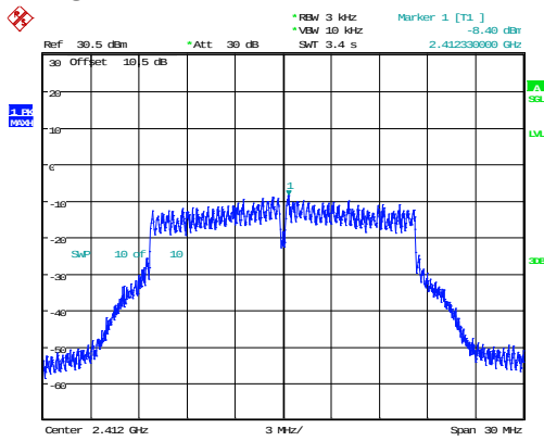
g_2412MHz_Chain 0 -8.40dBm/3kHz
