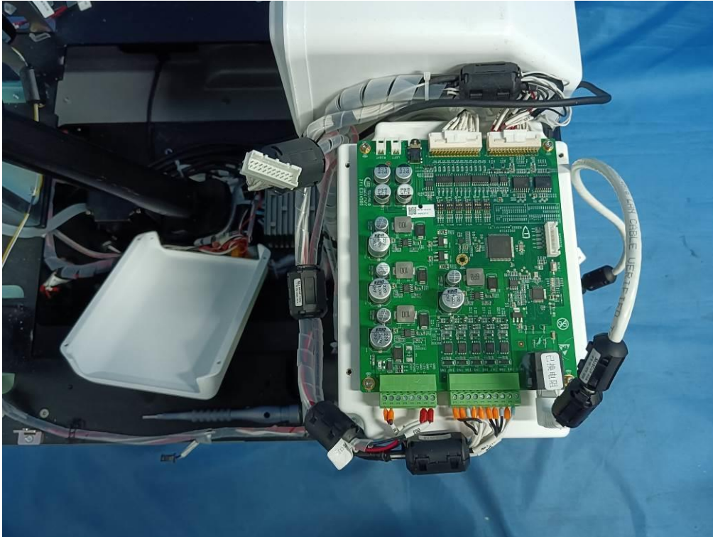
OPEN VIEW-16 OF EUT
