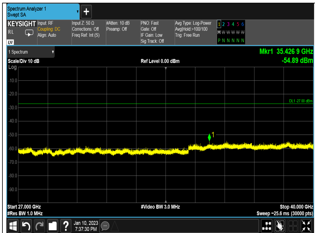
Test_Graph_802.11n40_ANT1_5190_MCS0_Frequency Band 5
