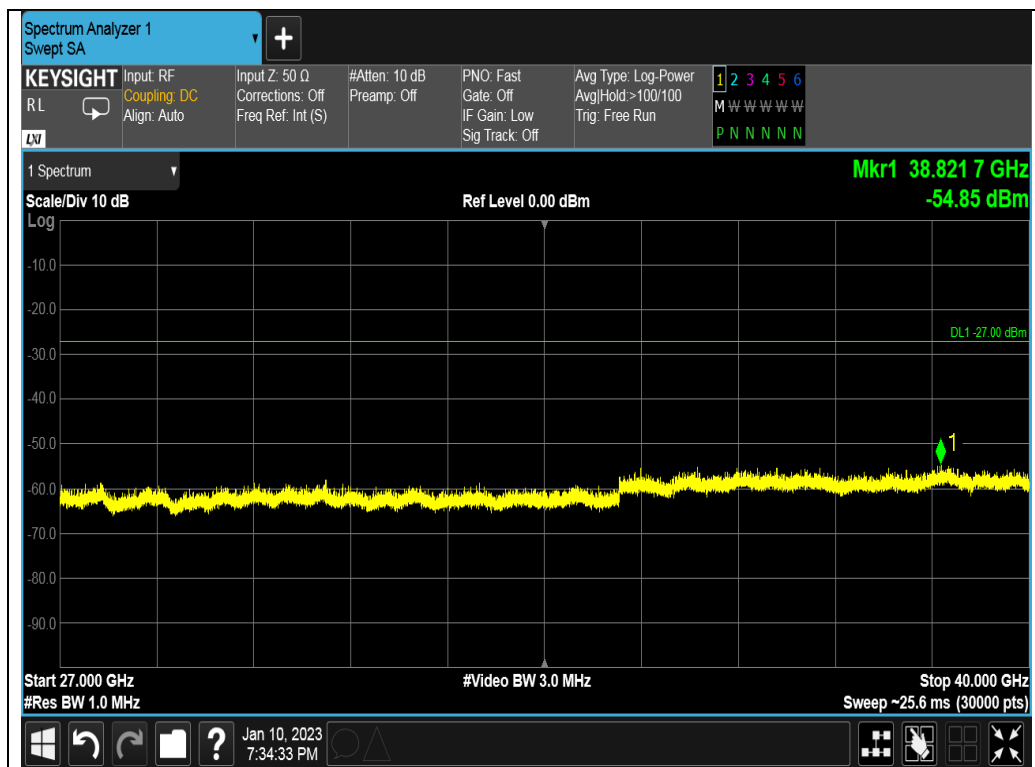
Test_Graph_802.11a_ANT1_5180_6Mbps_Frequency Band 5
