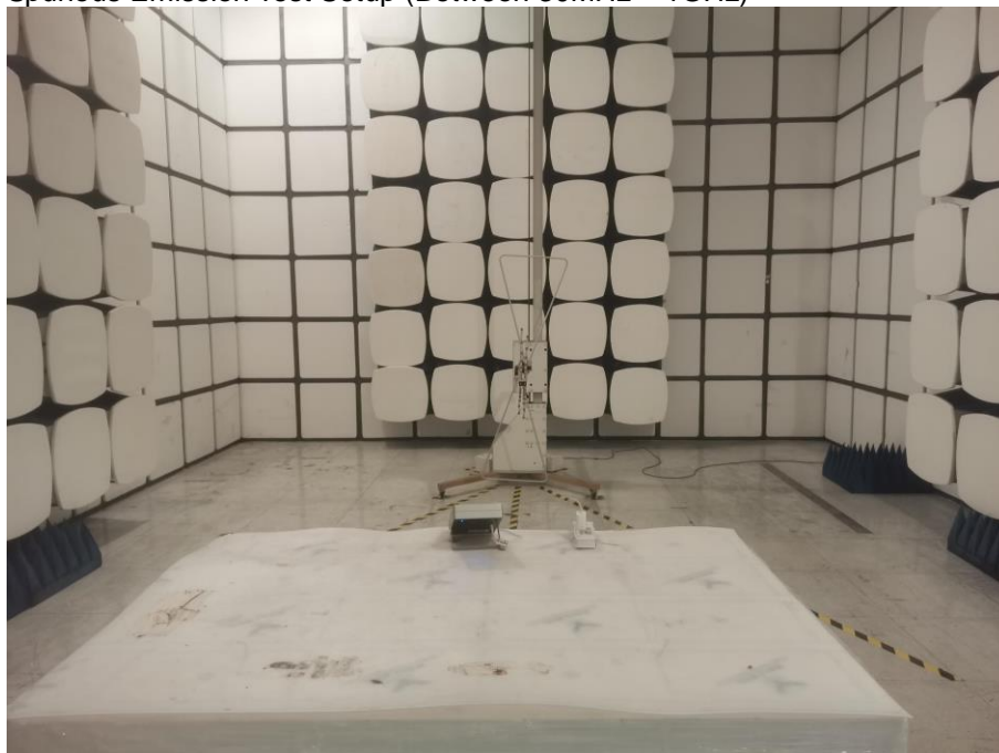
Spurious Emission Test Setup (Between 30MHz – 1GHz)
