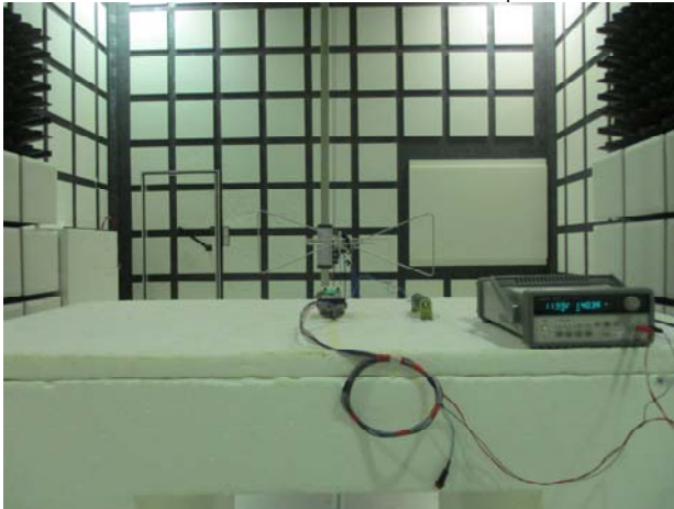
Part_15_209_WPC_Radiated_Setup
