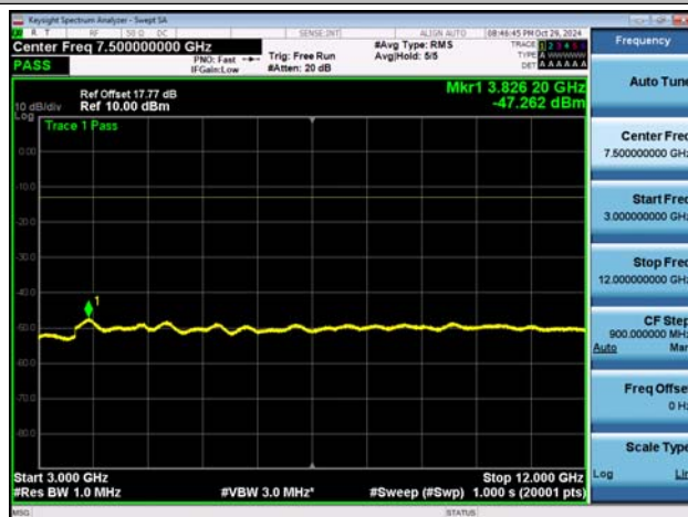
NTNV-n2-PC3-15-40-L-DFT-BPSK-Inner_1RB_Left-3000-12000-PASS
