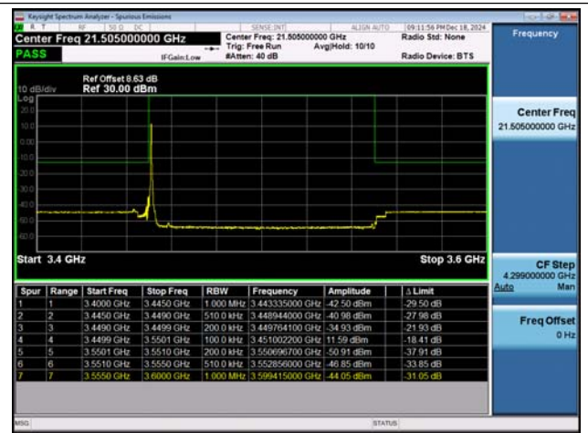
NTNV-n77(3450-3550)-PC3-30-100-M-DFT-BPSK-Edge_1 RB_Left-PASS
