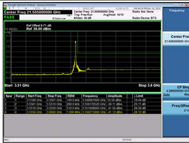
NTNV-n78(3450-3550)-PC2-30-40-H-DFT-BPSK-Edge_1RB_ Right-PASS
