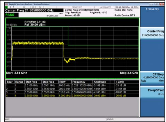
NTNV-n78(3450-3550)-PC2-30-40-H-DFT-BPSK-Outer_ Full-PASS
