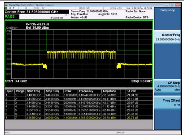
NTNV-n77(3450-3550)-PC3-30-100-M-DFT-BPSK-Out_F ull-PASS
