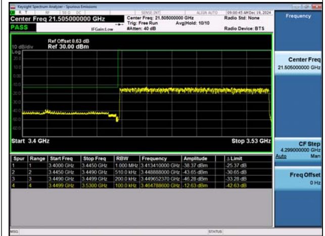
NTNV-n78(3450-3550)-PC2-30-80-L-DFT-BPSK-Outer_ Full-PASS
