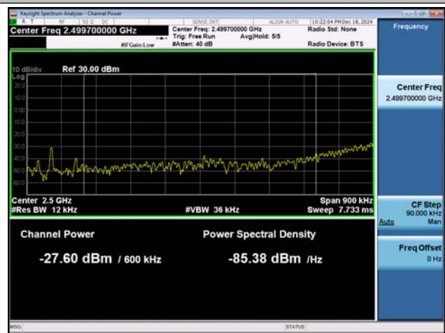
NTNV-n7-PC3-15-30-L-DFT-BPSK-Edge_1RB_Left-PASS_Fin al1
