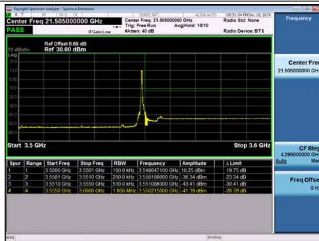
NTNV-n78(3450-3550)-PC2-30-50-H-DFT-BPSK-Edge_1RB_ Right-PASS
