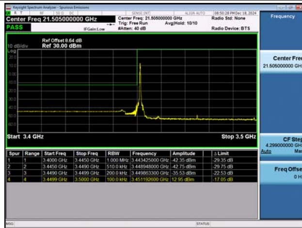
NTNV-n78(3450-3550)-PC2-30-50-L-DFT-BPSK-Edge_1RB_ Left-PASS
