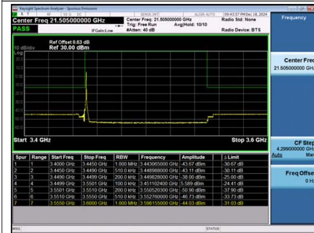
NTNV-n78(3450-3550)-PC2-30-100-M-CP-256QAM-Edge_1RB_Left-PASS
