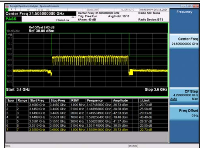
NTNV-n78(3450-3550)-PC2-30-100-M-CP-QPSK-Outer_Ful I-PASS
