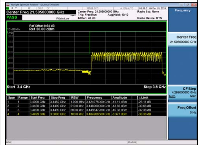
NTNV-n78(3450-3550)-PC2-30-50-L-DFT-BPSK-Outer_ Full-PASS
