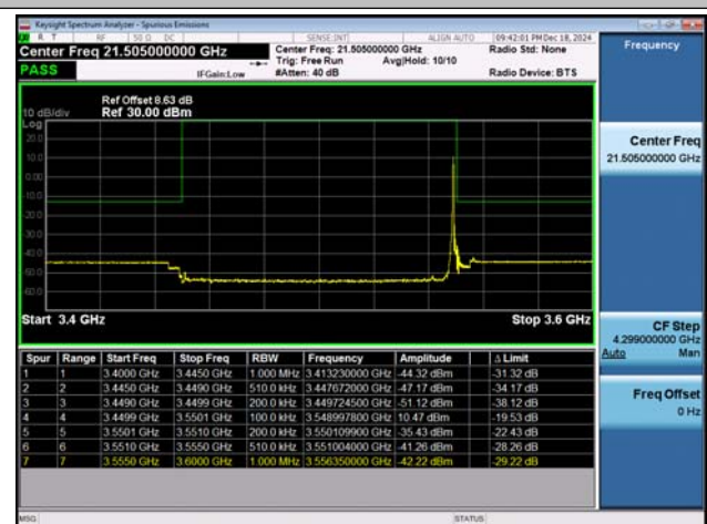
NTNV-n78(3450-3550)-PC2-30-100-M-CP-16QAM-Edge_1 RB_Right-PASS
