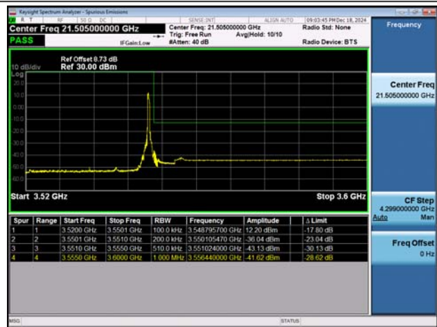
NTNV-n77(3450-3550)-PC3-30-30-H-DFT-BPSK-Edge_1RB_ Right-PASS
