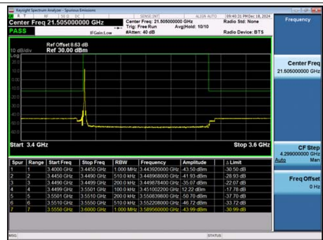
NTNV-n78(3450-3550)-PC2-30-100-M-CP-QPSK-Edge_1R B_Left-PASS
