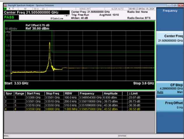
NTNV-n77(3450-3550)-PC3-30-20-H-DFT-BPSK-Edge_1RB_ Right-PASS
