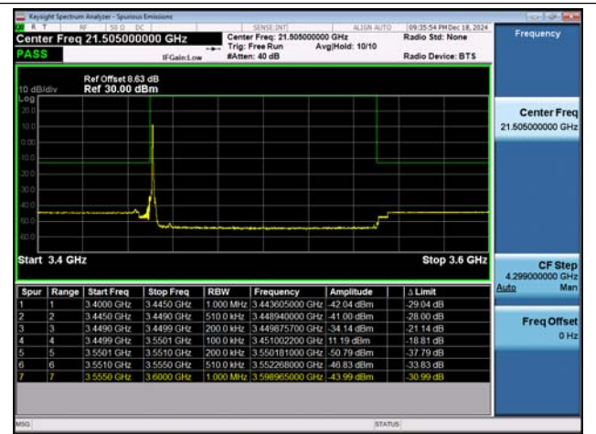
NTNV-n78(3450-3550)-PC2-30-100-M-DFT-QPSK-Edge_1 RB_Left-PASS
