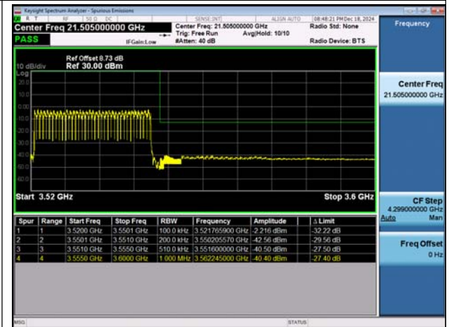
NTNV-n78(3450-3550)-PC2-30-30-H-DFT-BPSK-Outer_ Full-PASS
