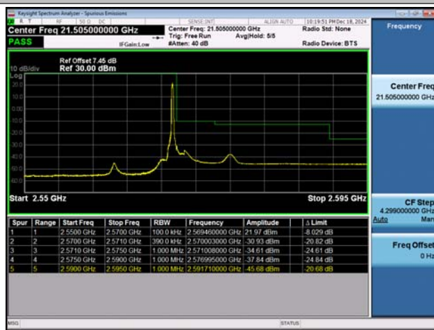
NTNV-n7-PC3-15-20-H-DFT-BPSK-Edge_1RB_Right-PASS
