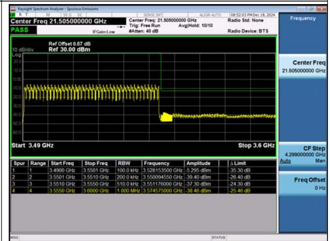
NTNV-n78(3450-3550)-PC2-30-60-H-DFT-BPSK-Outer_ Full-PASS
