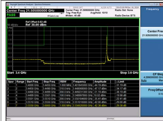
NTNV-n78(3450-3550)-PC2-30-100-M-CP-64QAM-Edge_1RB_Right-PASS
