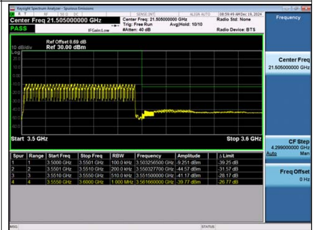
NTNV-n78(3450-3550)-PC2-30-50-H-DFT-BPSK-Outer_ Full-PASS
