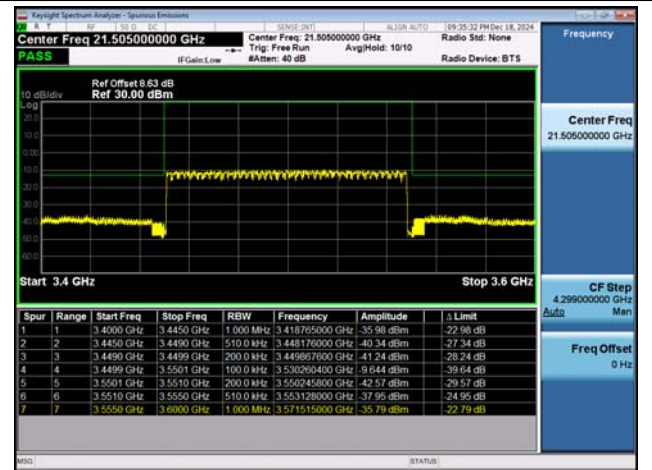
NTNV-n78(3450-3550)-PC2-30-100-M-DFT-QPSK-Outter_F ull-PASS
