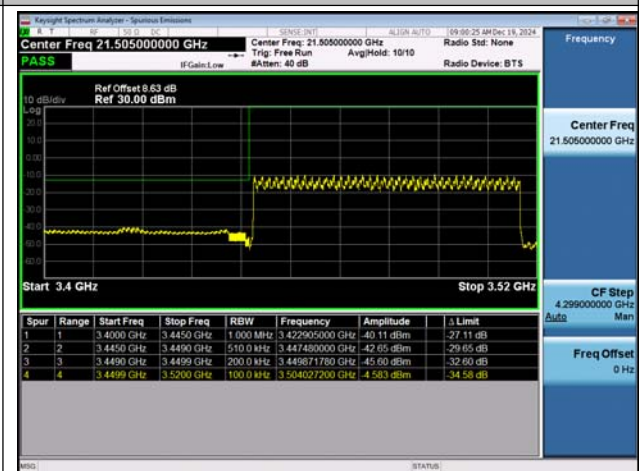
NTNV-n78(3450-3550)-PC2-30-70-L-DFT-BPSK-Outer_ Full-PASS
