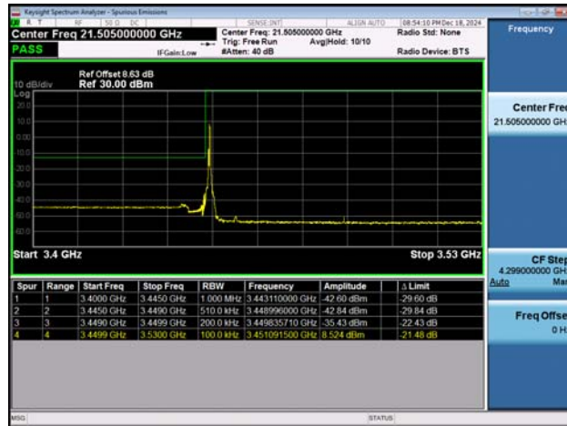
NTNV-n78(3450-3550)-PC2-30-80-L-DFT-BPSK-Edge_1RB_ Left-PASS
