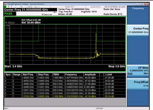
NTNV-n78(3450-3550)-PC2-30-100-M-DFT-16QAM-Edge_1 RB_Right-PASS
