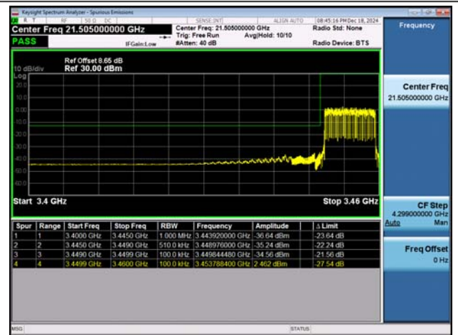
NTNV-n78(3450-3550)-PC2-30-10-L-DFT-BPSK-Out_Ful l-PASS
