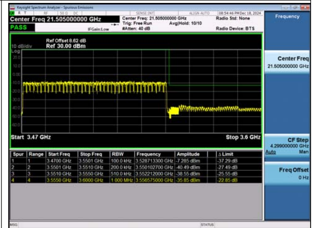
NTNV-n78(3450-3550)-PC2-30-80-H-DFT-BPSK-Outer_ Full-PASS
