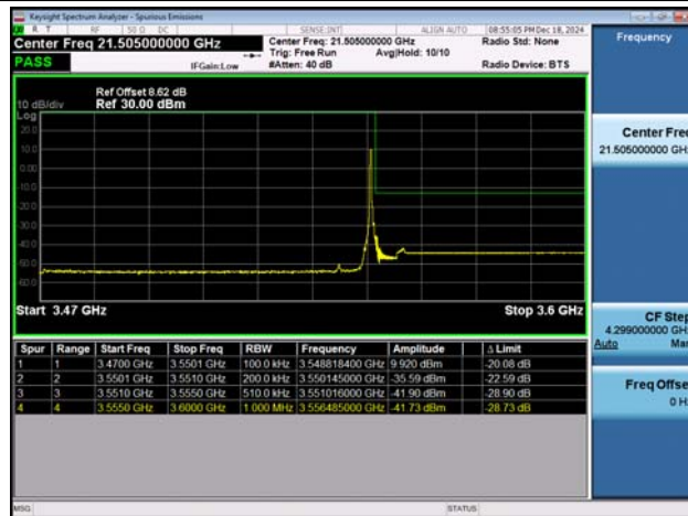
NTNV-n78(3450-3550)-PC2-30-80-H-DFT-BPSK-Edge_1RB_ Right-PASS
