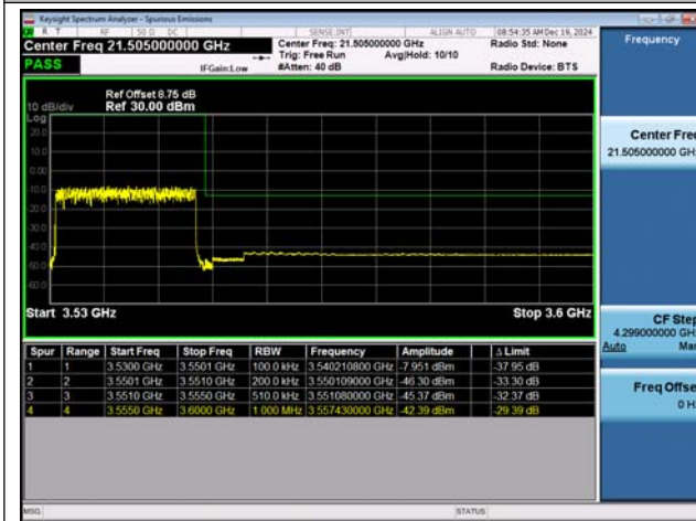
NTNV-n77(3450-3550)-PC3-30-20-H-DFT-BPSK-Outer_ Full-PASS
