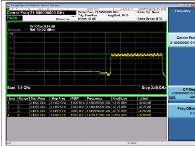
NTNV-n77(3450-3550)-PC3-30-30-L-DFT-BPSK-Outer_ Full-PASS
