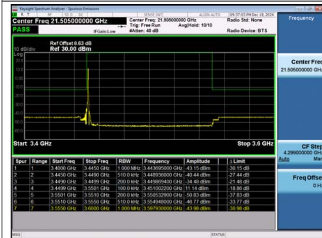
NTNV-n78(3450-3550)-PC2-30-100-M-DFT-16QAM-Edge_1 1RB_Left-PASS
