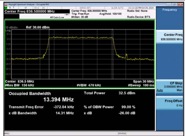
NTNV-n26(824-849)-PC3-15-15-M-DFT-BPSK-Outter_Full-Ant1-PASS
