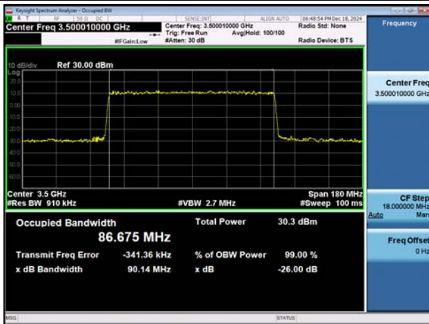
NTNV-n77(3450-3550)-PC3-30-90-M-DFT-QPSK-Outter_Fu ll-Ant1-PASS
