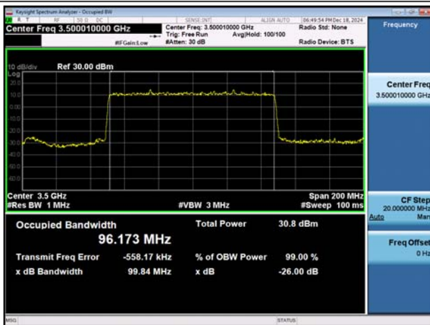
NTNV-n77(3450-3550)-PC3-30-100-M-DFT-BPSK-Outter_F ull-Ant1-PASS
