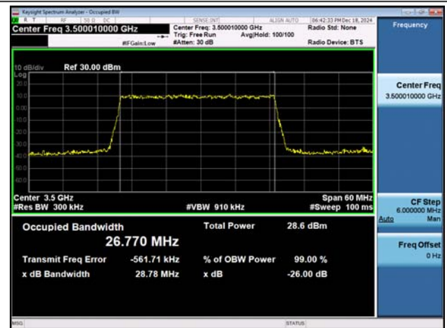
NTNV-n77(3450-3550)-PC3-30-30-M-DFT-16QAM-Outter_Full-Ant1-PASS
