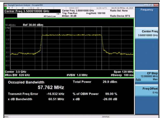
NTNV-n77(3450-3550)-PC3-30-60-M-DFT-QPSK-Out_Ful l-Ant1-PASS
