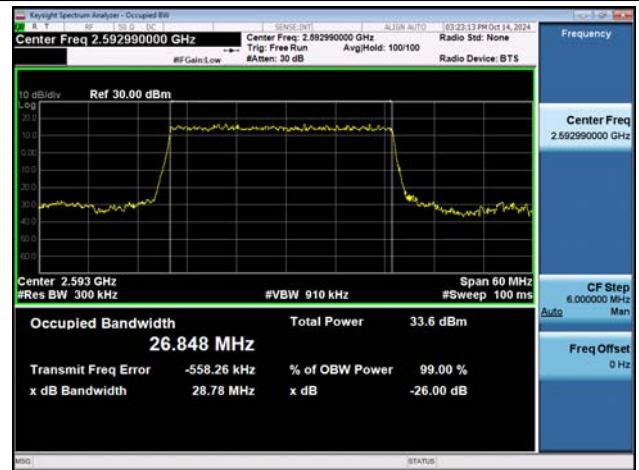
NTNV-n41-PC2-30-20-M-DFT-QPSK-Outer_Full-Ant1-PAS S
