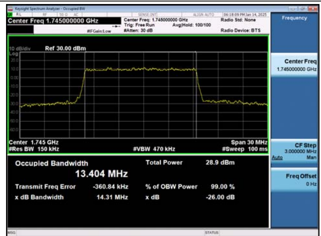
NTVN-n66-PC3-15-15-M-DFT-16QAM-Outer_Full-Ant1-PASS SS
