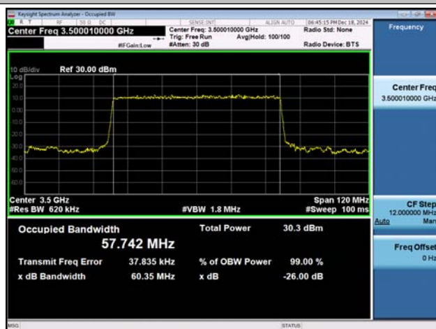
NTNV-n77(3450-3550)-PC3-30-60-M-DFT-BPSK-Out_Ful l-Ant1-PASS
