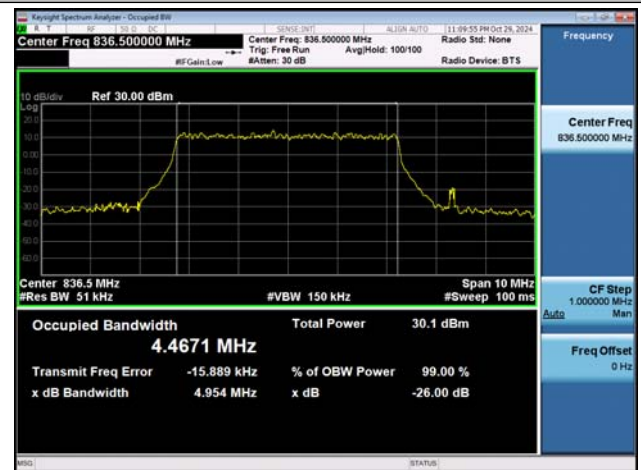
NTNV-n26(824-849)-PC3-15-5-M-DFT-16QAM-Outet_Full-Ant1-PASS
