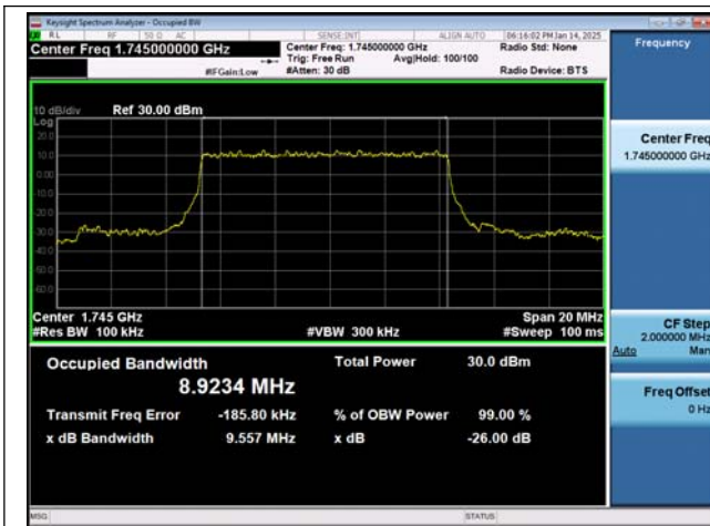
NTVN-n66-PC3-15-10-M-DFT-BPSK-Outer_Full-Ant1-PASS
