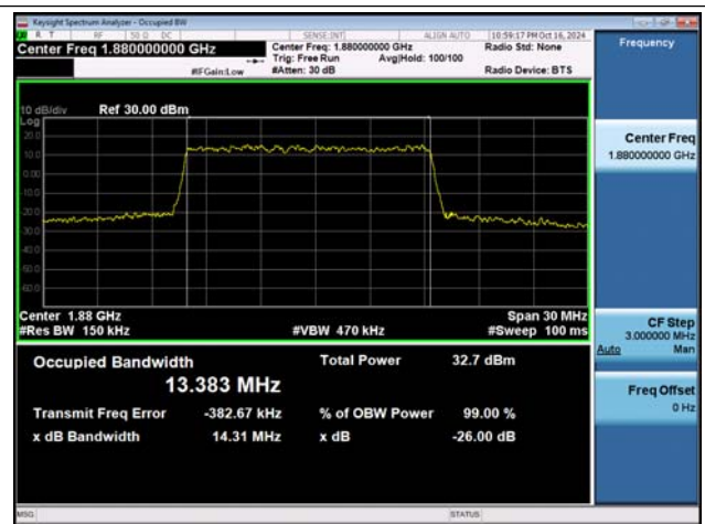
NTVN-n2-PC3-15-15-M-DFT-QPSK-Outet_Full-Ant1-PASS
