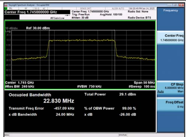
NTVN-n66-PC3-15-25-M-DFT-16QAM-Outer_Full-Ant1-PASS SS
