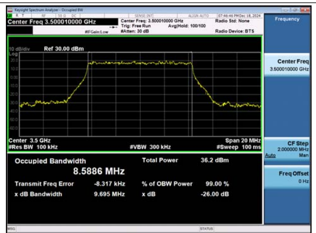
NTNV-n78(3450-3550)-PC2-30-10-M-DFT-BPSK-Out_ Fu ll-Ant1-PASS
