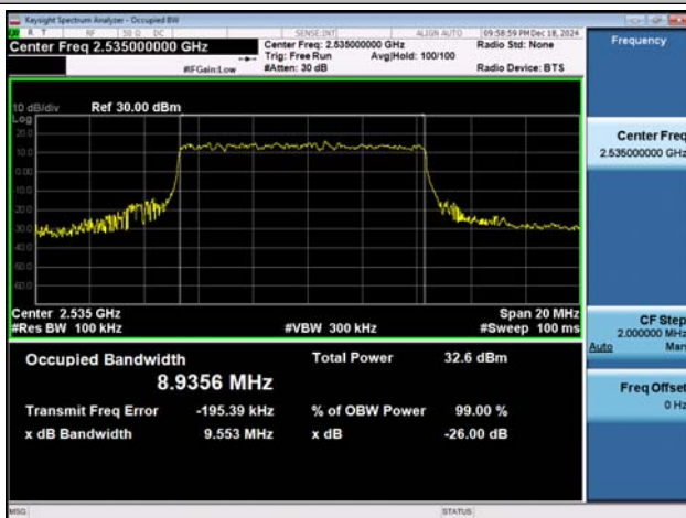
NTVN-n7-PC3-15-5-M-DFT-16QAM-Outer_Full-Ant1-PASS
