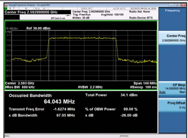
NTNV-n41-PC2-30-60-M-DFT-QPSK-Outer_Full-Ant1-PASS S
