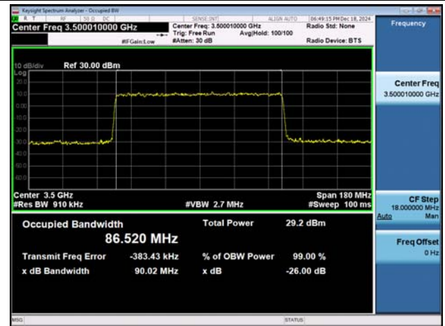
NTNV-n77(3450-3550)-PC3-30-90-M-DFT-16QAM-Outter_F ull-Ant1-PASS
