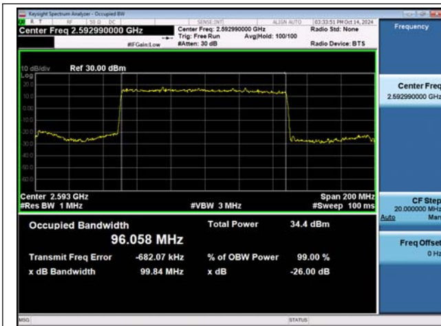
NTNV-n41-PC2-30-100-M-DFT-BPSK-Outter_Full-Ant1-PAS
