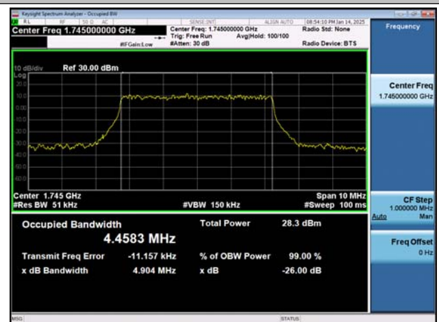
NTNV-n66-PC3-15-5-M-DFT-16QAM-Outter_Full-Ant1-PAS
