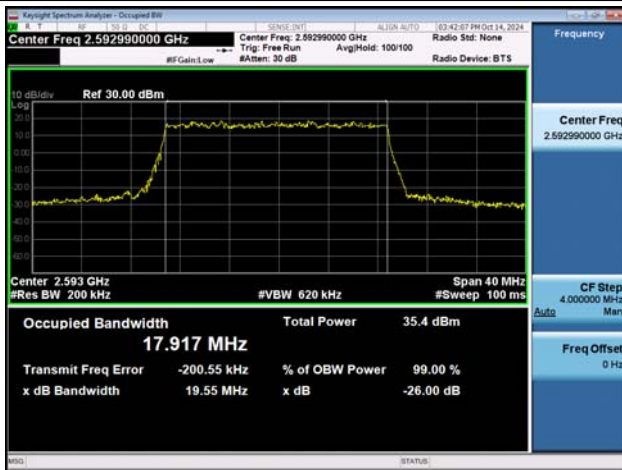
NTNV-n41-PC2-30-20-M-DFT-16QAM-Outer_Full-Ant1-PA SS
