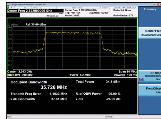
NTNV-n41-PC2-30-40-M-DFT-BPSK-Outer_Full-Ant1-PASS
