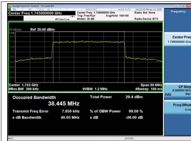
NTNV-n66-PC3-15-40-M-DFT-16QAM-Outter_Full-Ant1-PA SS
