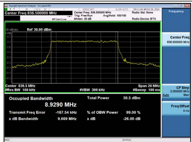
NTVN-n5-PC3-15-10-M-DFT-BPSK-Outer_Full-Ant1-PASS
