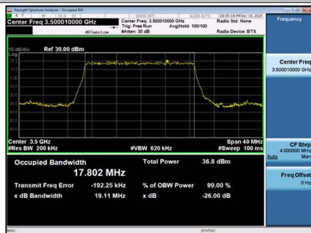
NTNV-n78(3450-3550)-PC2-30-20-M-DFT-BPSK-Out_ Full -Ant1-PASS
