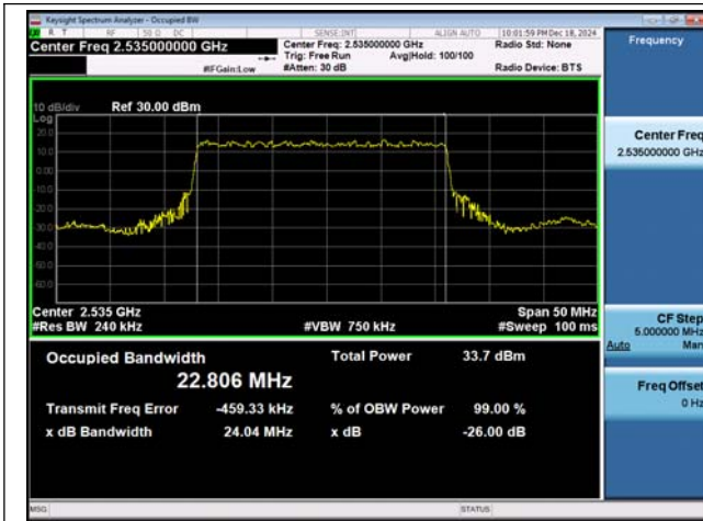
NTVN-n7-PC3-15-25-M-DFT-BPSK-Outter_Full-Ant1-PASS
