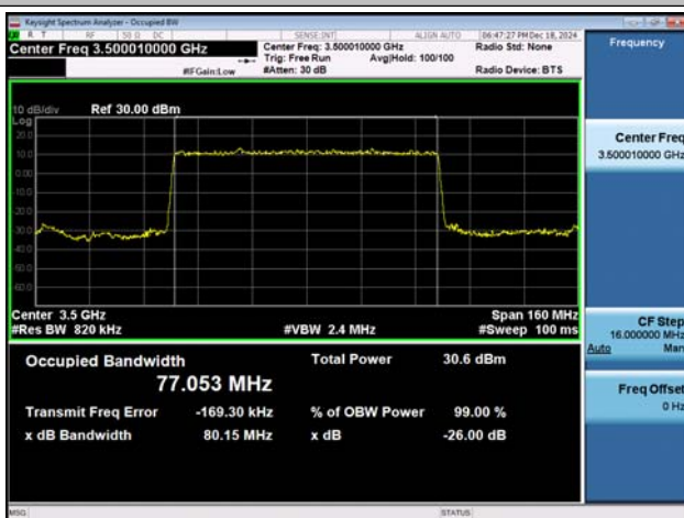
NTNV-n77(3450-3550)-PC3-30-80-M-DFT-BPSK-Outter_Full-Ant1-PASS
