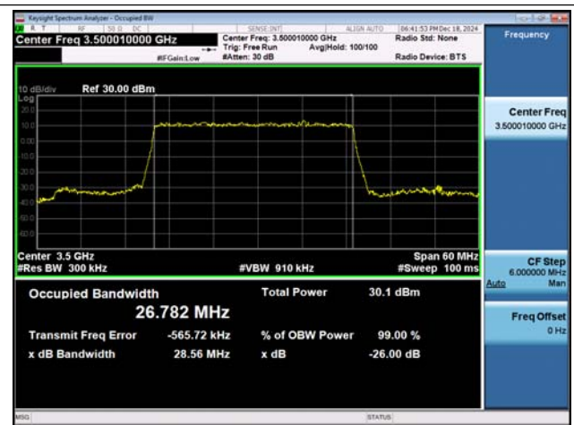
NTNV-n77(3450-3550)-PC3-30-30-M-DFT-BPSK-Outter_Full-Ant1-PASS
