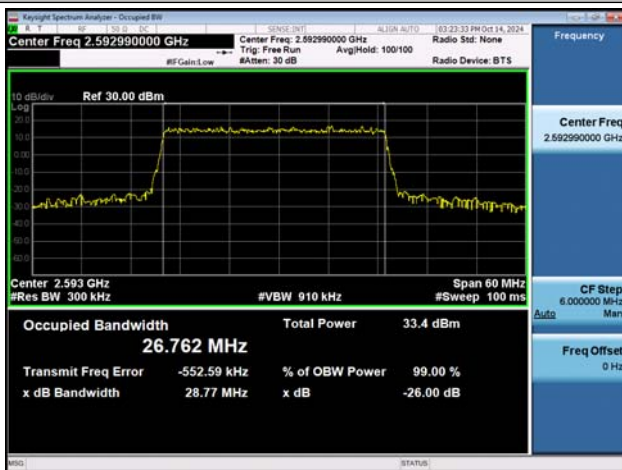
NTNV-n41-PC2-30-30-M-DFT-QPSK-Outer_Full-Ant1-PAS S
