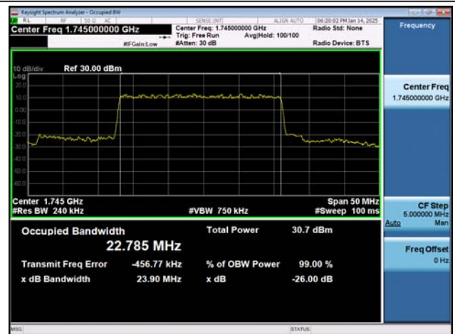
NTVN-n66-PC3-15-20-M-DFT-QPSK-Outer_Full-Ant1-PASS S
