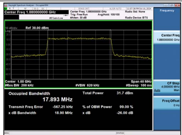
NTVN-n2-PC3-15-20-M-DFT-16QAM-Outet_Full-Ant1-PASS
