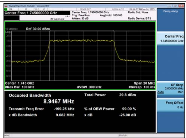
NTVN-n66-PC3-15-10-M-DFT-QPSK-Outer_Full-Ant1-PASS S
