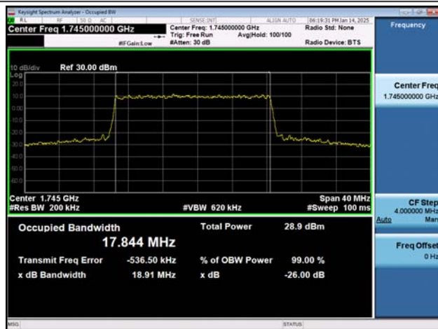
NTVN-n66-PC3-15-20-M-DFT-16QAM-Outer_Full-Ant1-PASS SS
