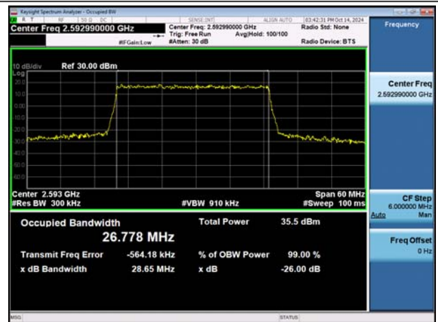
NTNV-n41-PC2-30-30-M-DFT-16QAM-Outer_Full-Ant1-PA SS
