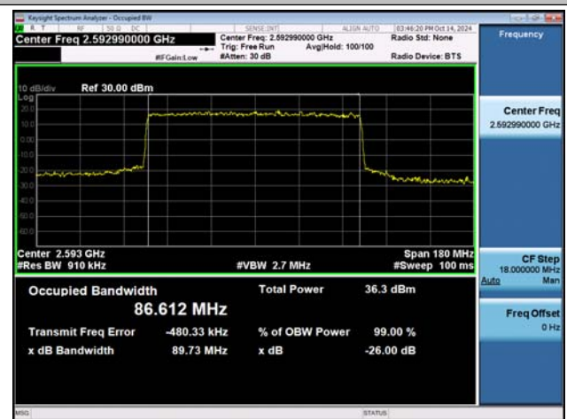
NTNV-n41-PC2-30-90-M-DFT-16QAM-Outer_Full-Ant1-PA SS
