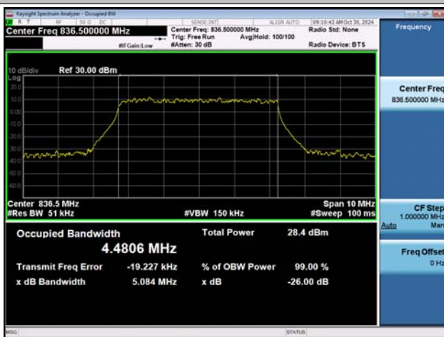
NTVN-n5-PC3-15-5-M-DFT-16QAM-Outer_Full-Ant1-PASS
