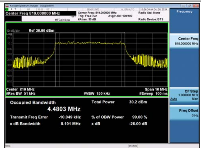
NTNV-n26(814-824)-PC3-15-5-M-DFT-16QAM-Outet1-PASS
