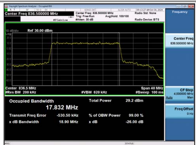
NTVN-n5-PC3-15-20-M-DFT-16QAM-Outter_Full-Ant1-PASS
