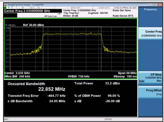
NTVN-n7-PC3-15-25-M-DFT-QPSK-Outter_Full-Ant1-PASS
