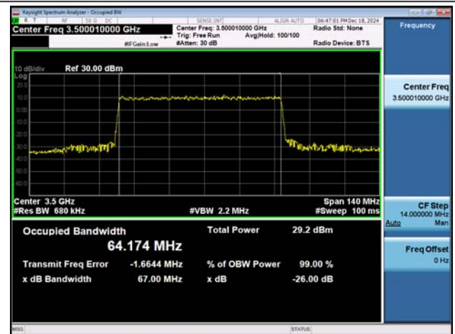
NTNV-n77(3450-3550)-PC3-30-70-M-DFT-16QAM-Outter_Full-Ant1-PASS
