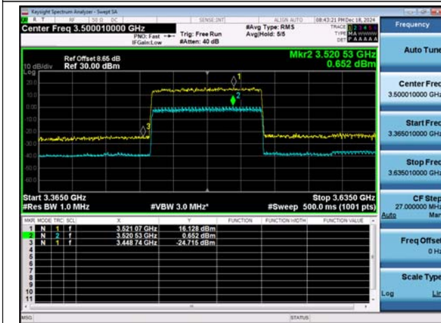
NTNT-n78(3450-3550)-PC2-30-90-M-DFT-256QAM-Out_ Full-Ant1-PASS
