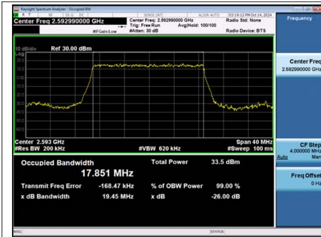
NTNV-n41-PC2-30-20-M-DFT-BPSK-Outer_Full-Ant1-PASS
