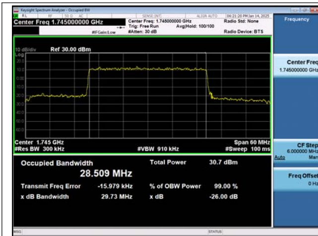
NTNV-n66-PC3-15-30-M-DFT-BPSK-Outer_Full-Ant1-PASS
