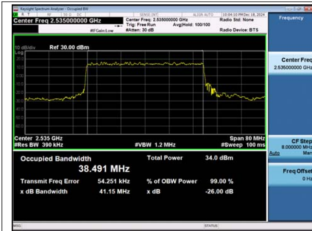
NTNV-n7-PC3-15-40-M-DFT-BPSK-Outet1-PASS
