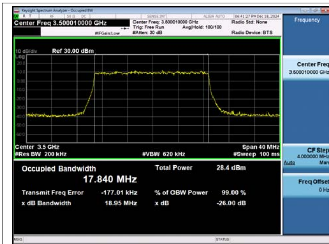
NTNV-n77(3450-3550)-PC3-30-20-M-DFT-16QAM-Outter_Full-Ant1-PASS
