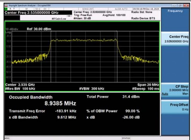
NTVN-n7-PC3-15-10-M-DFT-16QAM-Outer_Full-Ant1-PAS
