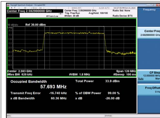
NTNV-n41-PC2-30-60-M-DFT-BPSK-Outer_Full-Ant1-PASS
