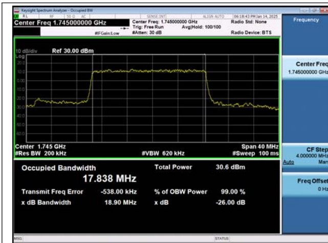
NTVN-n66-PC3-15-20-M-DFT-BPSK-Outer_Full-Ant1-PASS
