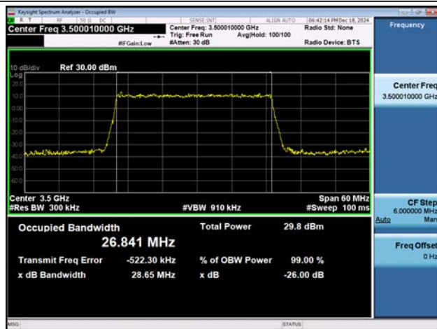
NTNV-n77(3450-3550)-PC3-30-30-M-DFT-QPSK-Outter_Full-Ant1-PASS
