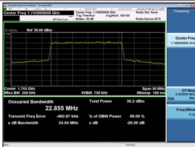
NTVN-n66-PC3-15-25-M-DFT-QPSK-Outer_Full-Ant1-PASS S
