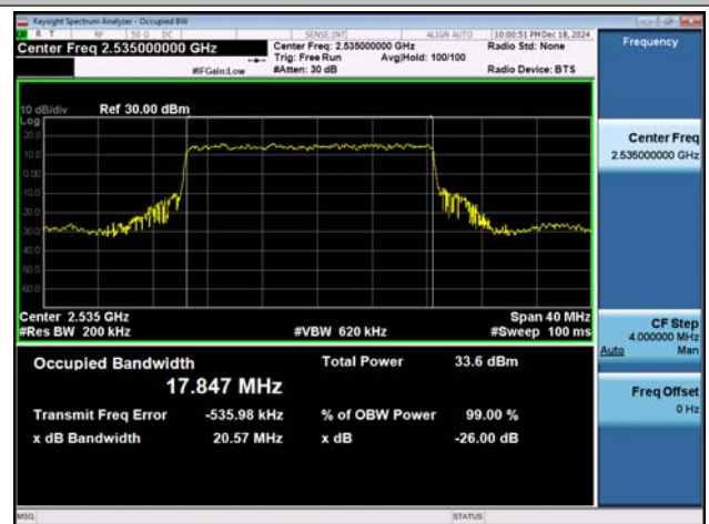
NTVN-n7-PC3-15-15-M-DFT-QPSK-Outter_Full-Ant1-PASS
