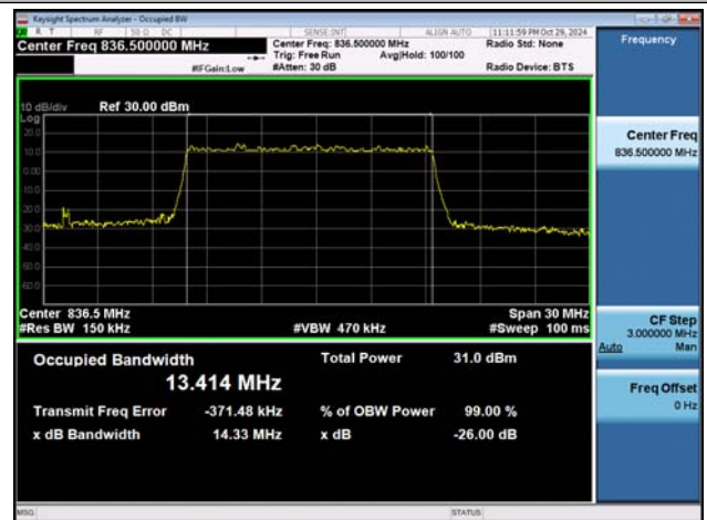
NTNV-n26(824-849)-PC3-15-15-M-DFT-16QAM-Outter_Full-Ant1-PASS
