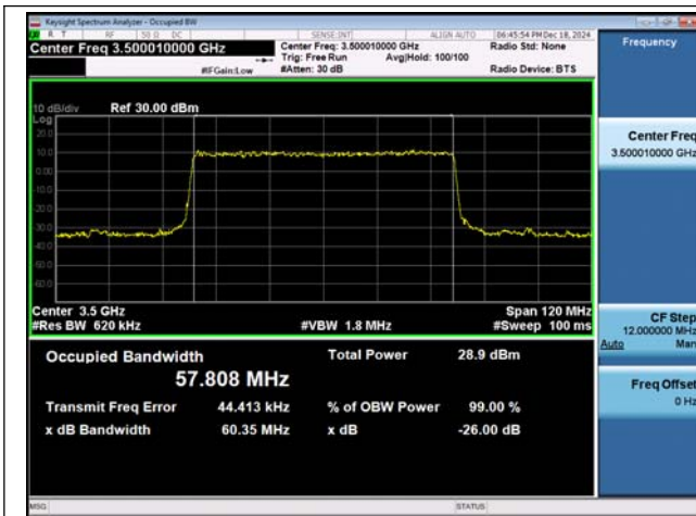
NTNV-n77(3450-3550)-PC3-30-60-M-DFT-16QAM-Outter_Full-Ant1-PASS
