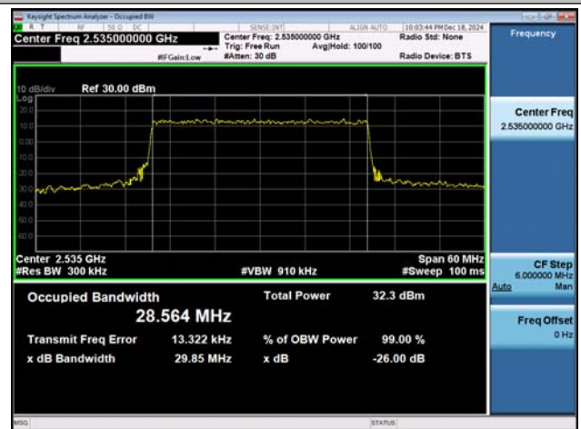
NTVN-n7-PC3-15-30-M-DFT-16QAM-Outter_Full-Ant1-PASS
