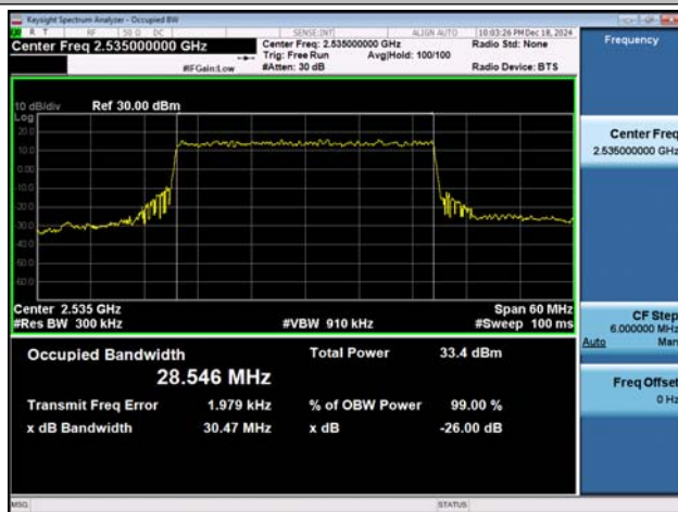
NTVN-n7-PC3-15-25-M-DFT-16QAM-Outter_Full-Ant1-PASS
