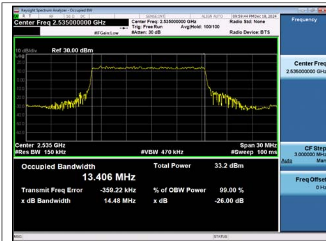
NTVN-n7-PC3-15-15-M-DFT-BPSK-Outter_Full-Ant1-PASS
