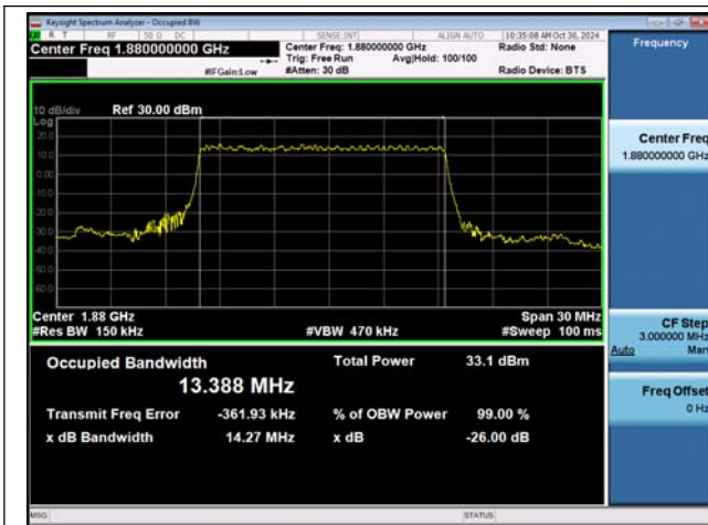
NTVN-n2-PC3-15-15-M-DFT-BPSK-Outet_Full-Ant1-PASS
