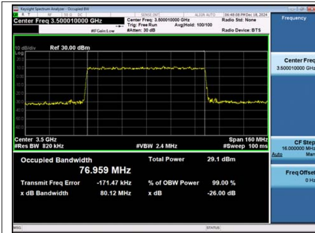
NTNV-n77(3450-3550)-PC3-30-80-M-DFT-16QAM-Outter_F ull-Ant1-PASS
