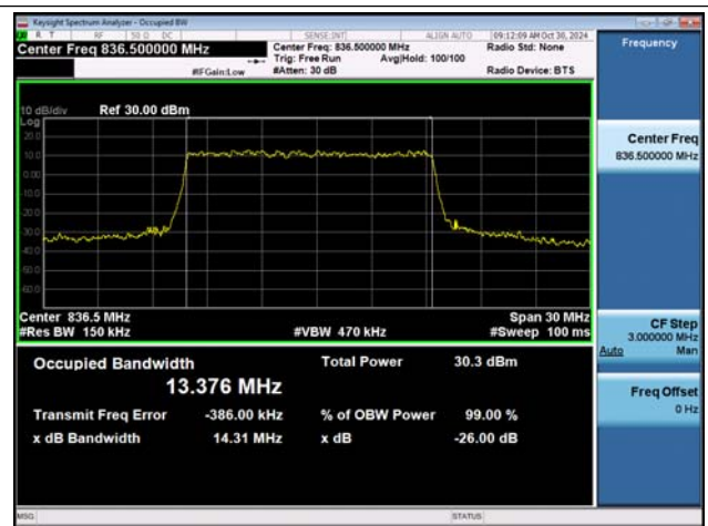
NTVN-n5-PC3-15-15-M-DFT-QPSK-Outter_Full-Ant1-PASS
