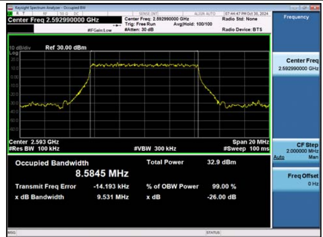
NTNV-n41-PC2-30-10-M-DFT-BPSK-Outet_Full-Ant1-PASS
