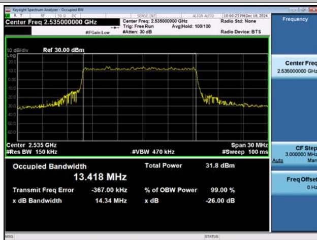
NTVN-n7-PC3-15-15-M-DFT-16QAM-Outter_Full-Ant1-PASS
