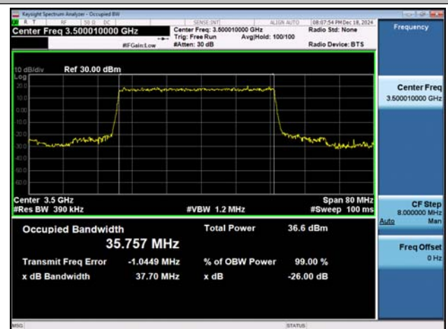
NTNV-n78(3450-3550)-PC2-30-40-M-DFT-QPSK-Outer_Full-Ant1-PASS
