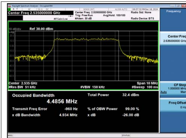
NTVN-n7-PC3-15-5-M-DFT-BPSK-Outer_Full-Ant1-PASS
