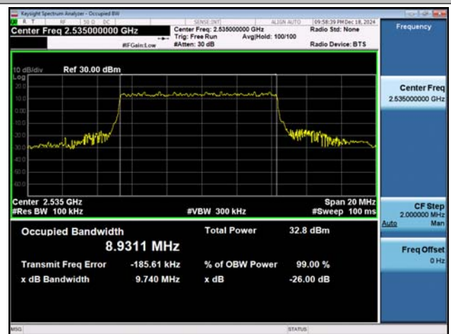
NTVN-n7-PC3-15-10-M-DFT-BPSK-Outer_Full-Ant1-PASS
