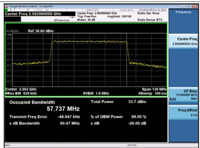
NTNV-n41-PC2-30-60-M-DFT-QPSK-Outer_Full-Ant1-PASS S
