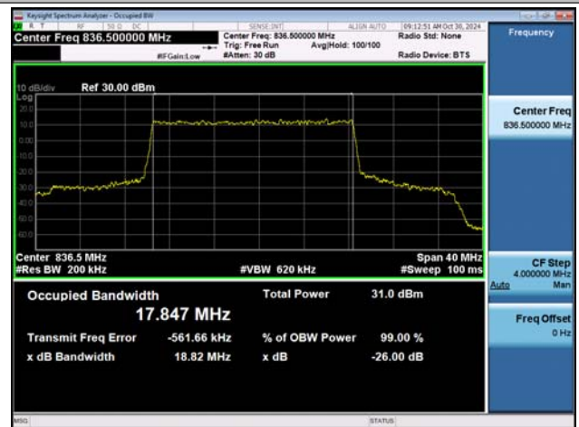
NTVN-n5-PC3-15-15-M-DFT-QPSK-Outter_Full-Ant1-PASS
