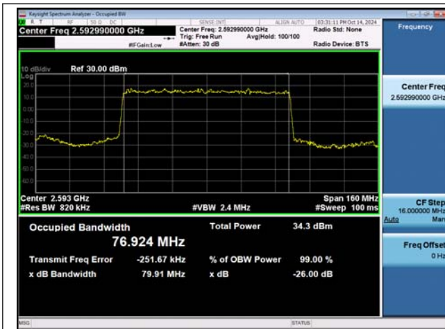
NTNV-n41-PC2-30-80-M-DFT-BPSK-Outer_Full-Ant1-PASS
