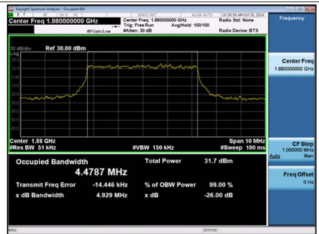
NTNV-n2-PC3-15-5-M-DFT-QPSK-Outer_Full-Ant1-PASS
