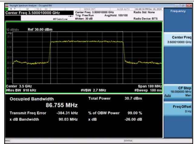
NTNV-n77(3450-3550)-PC3-30-90-M-DFT-BPSK-Outter_Ful l-Ant1-PASS
