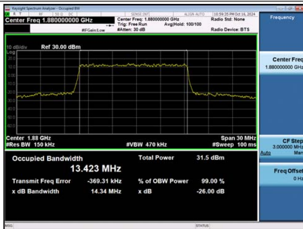
NTVN-n2-PC3-15-15-M-DFT-16QAM-Outet_Full-Ant1-PASS
