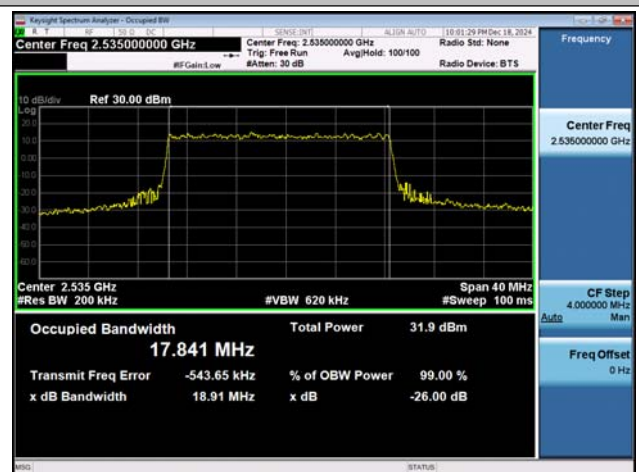
NTVN-n7-PC3-15-20-M-DFT-16QAM-Outter_Full-Ant1-PASS
