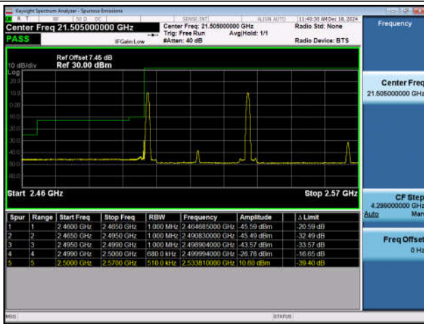
15MHz-20MHz_QPSK@QPSK-QPSK@QPSK_20828-209 99_1RB#0@75RB#0-1RB#99@100RB#0
