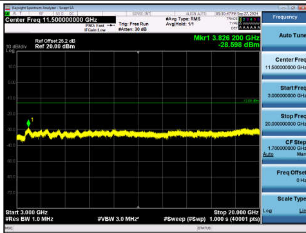
Band2_20MHz_QPSK_19100_1RB#0_3000~20000_3000~20000
