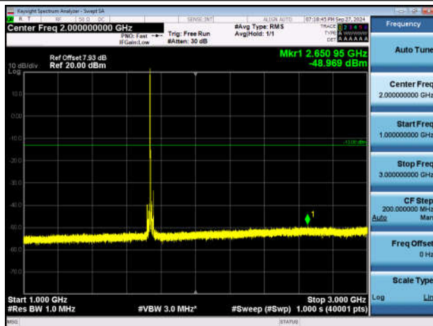
Band66_20MHz_QPSK_132322_1RB#0_1000~3000_1000
