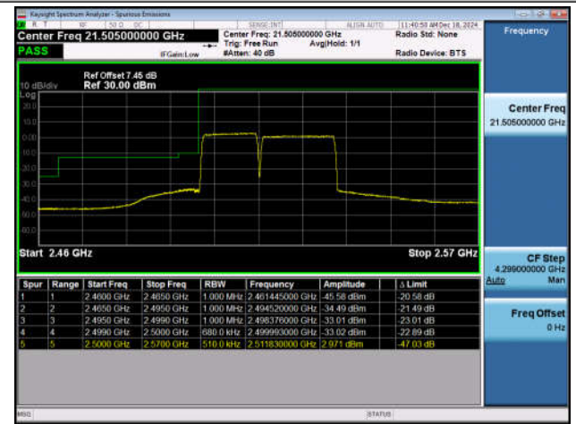
15MHz-20MHz_QPSK@QPSK-QPSK@QPSK_20828-2099 9_75RB#0@75RB#0-100RB#0@100RB#0
