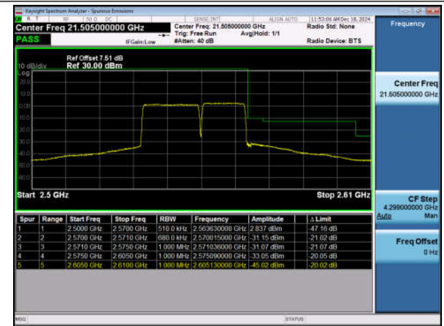
20MHz-20MHz_QPSK@QPSK-QPSK@QPSK_20850-2104 8_100RB#0@100RB#0-100RB#0@100RB#0
