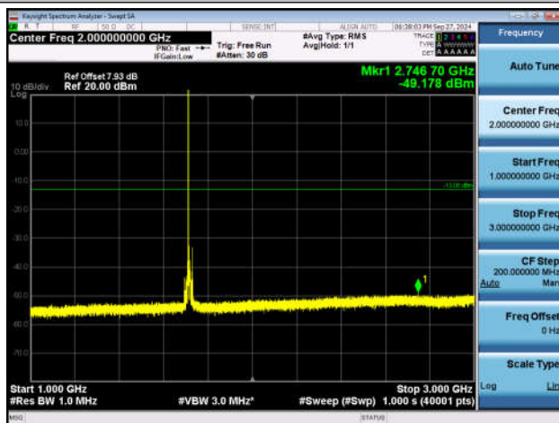
Band4_20MHz_QPSK_20050_1RB#0_1000~3000_1000~3000
