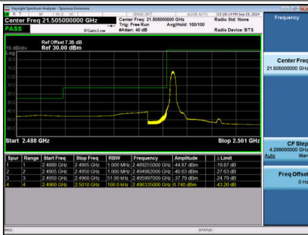
Band41_5MHz_QPSK_39675_1RB#0
