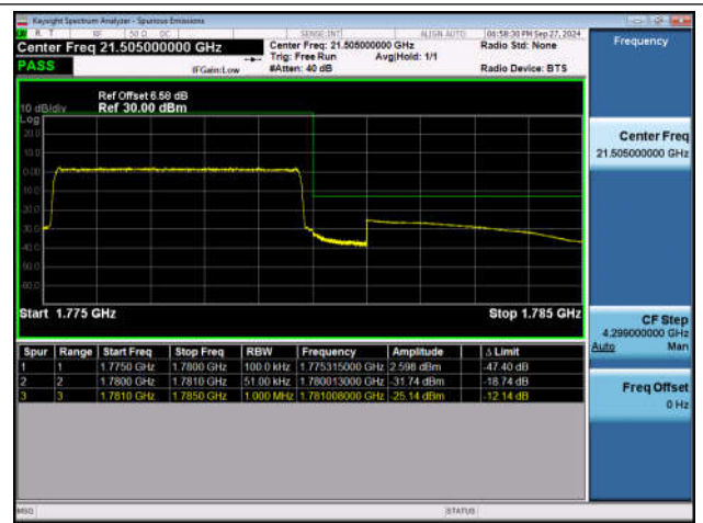
Band66_5MHz_QPSK_132647_25RB#0
