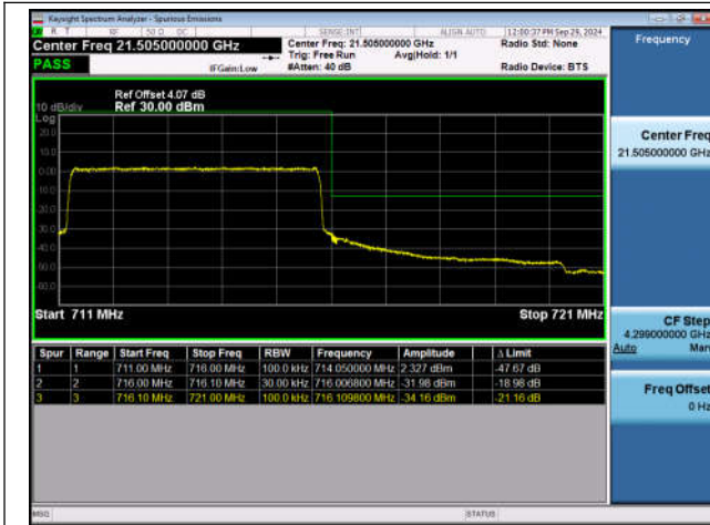
Band17_5MHz_QPSK_23825_25RB#0
