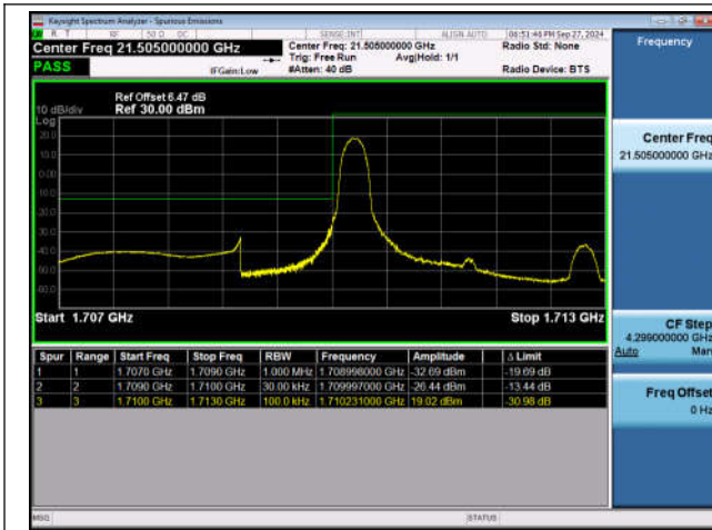
Band66_3MHz_QPSK_131987_1RB#0
