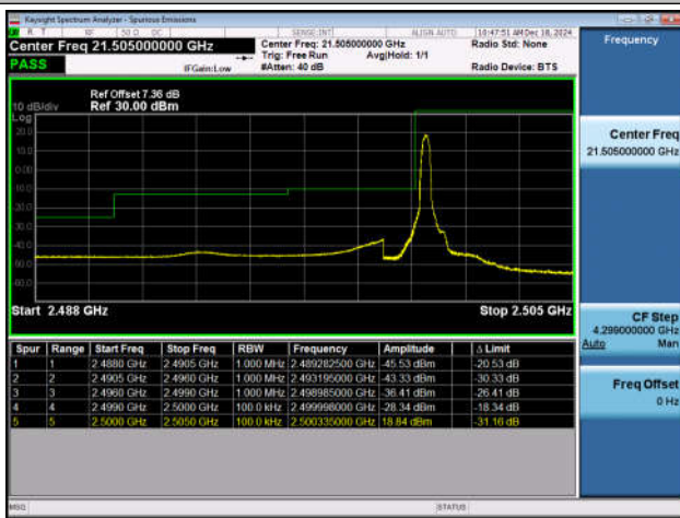
Band7_5MHz_QPSK_20775_1RB#0
