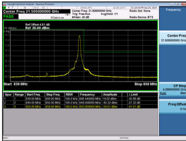
Band26_10MHz_QPSK_26990_1RB#49
