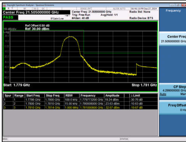
Band66_1.4MHz_QPSK_132665_1RB#5
