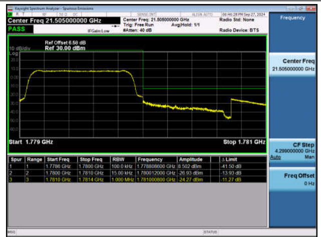
Band66_1.4MHz_QPSK_132665_6RB#0
