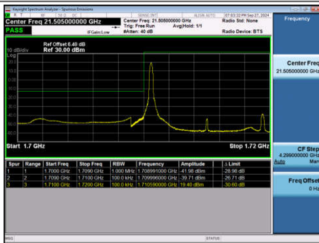
Band66_10MHz_QPSK_132022_1RB#0
