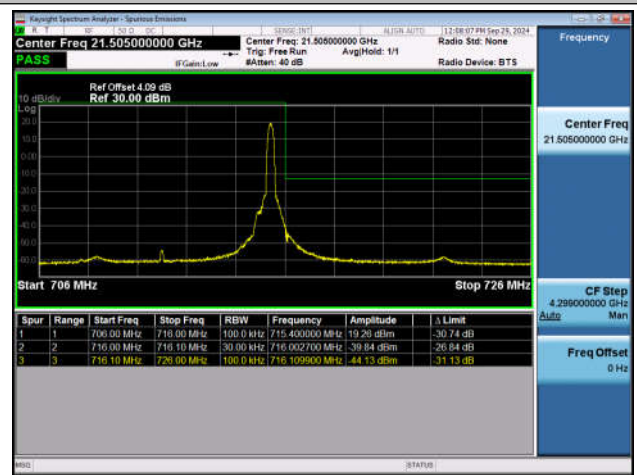
Band17_10MHz_QPSK_23800_1RB#49
