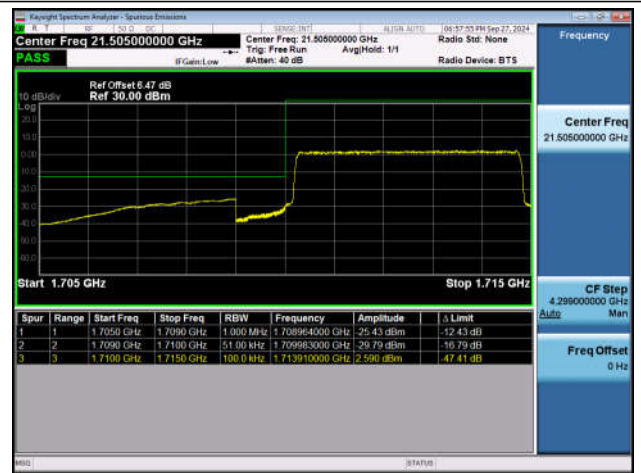
Band66_5MHz_QPSK_131997_25RB#0
