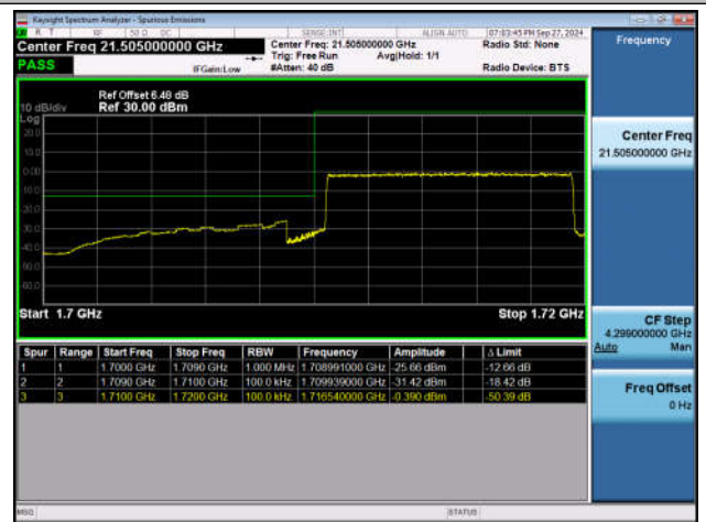
Band66_10MHz_QPSK_132022_50RB#0
