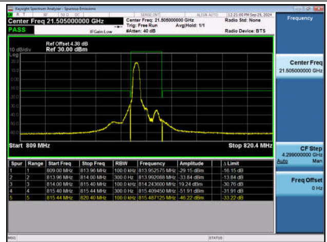
Band26_1.4MHz_QPSK_26697_1RB#0
