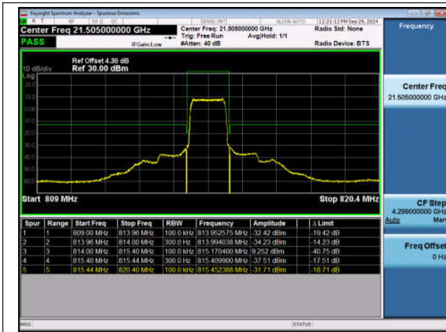
Band26_1.4MHz_QPSK_26697_6RB#0
