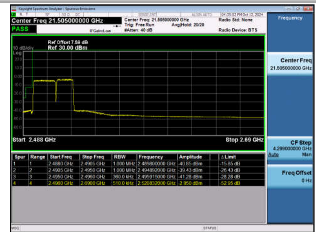
20MHz-15MHz_QPSK@QPSK-QPSK@QPSK_41341-4151 2_100RB#0@100RB#0-75RB#0@75RB#0
