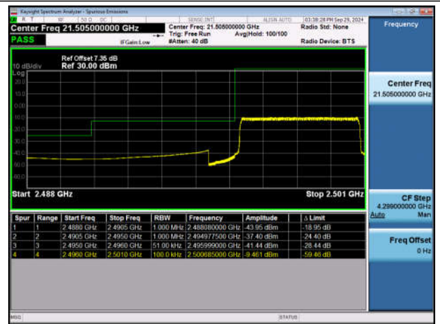
Band41_5MHz_QPSK_39675_25RB#0
