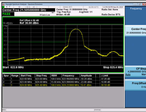
Band26_1.4MHz_QPSK_26797_1RB#0
