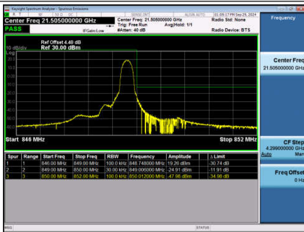
Band26_3MHz_QPSK_27025_1RB#14
