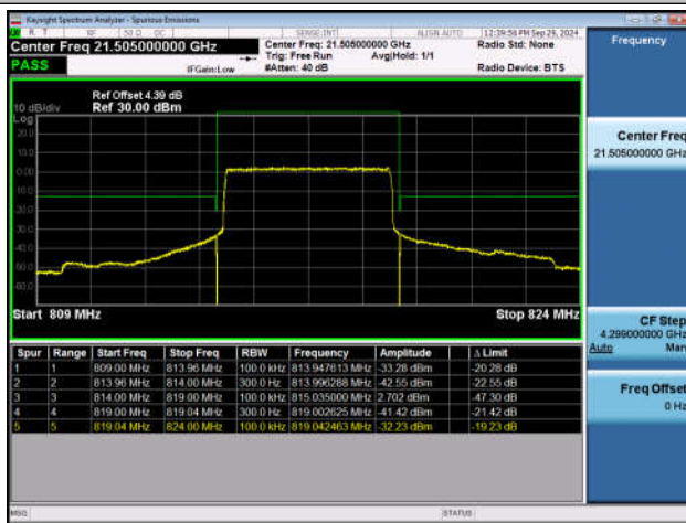
Band26_5MHz_QPSK_26715_25RB#0
