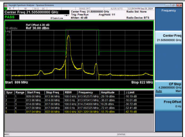
Band26_3MHz_QPSK_26705_1RB#0
