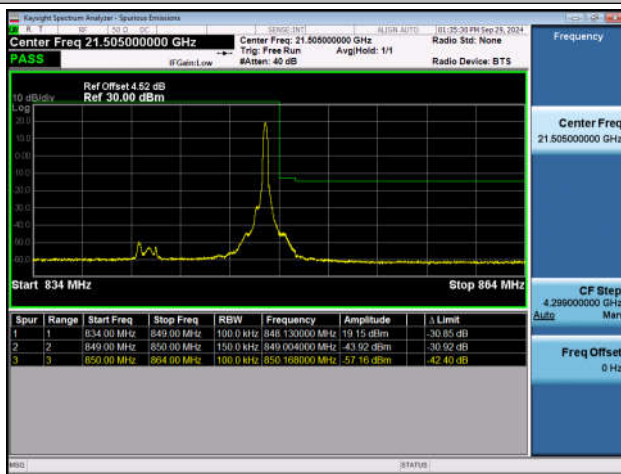
Band26_15MHz_QPSK_26965_1RB#74
