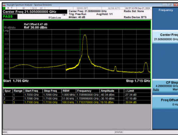
Band66_5MHz_QPSK_131997_1RB#0
