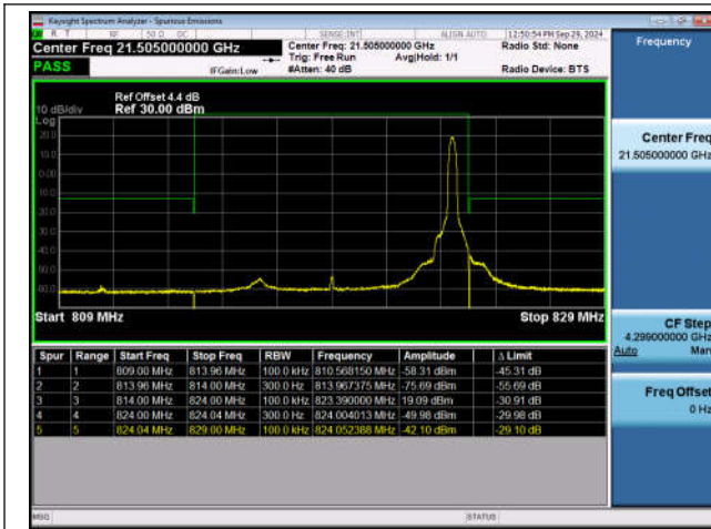
Band26_10MHz_QPSK_26740_1RB#49
