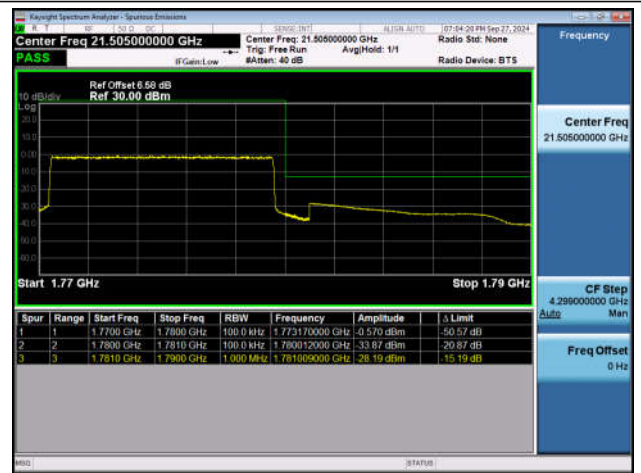
Band66_10MHz_QPSK_132622_50RB#0
