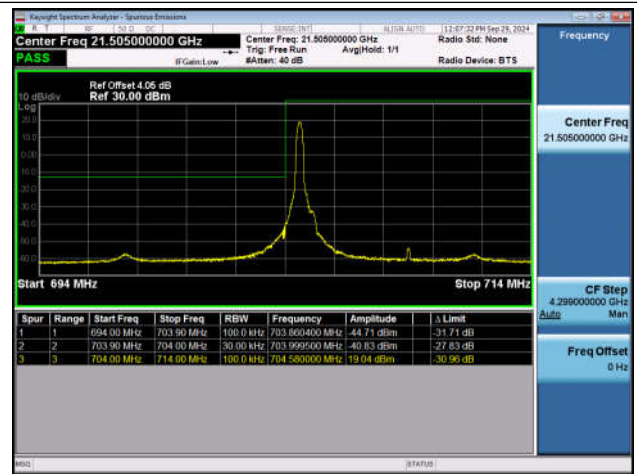
Band17_10MHz_QPSK_23780_1RB#0
