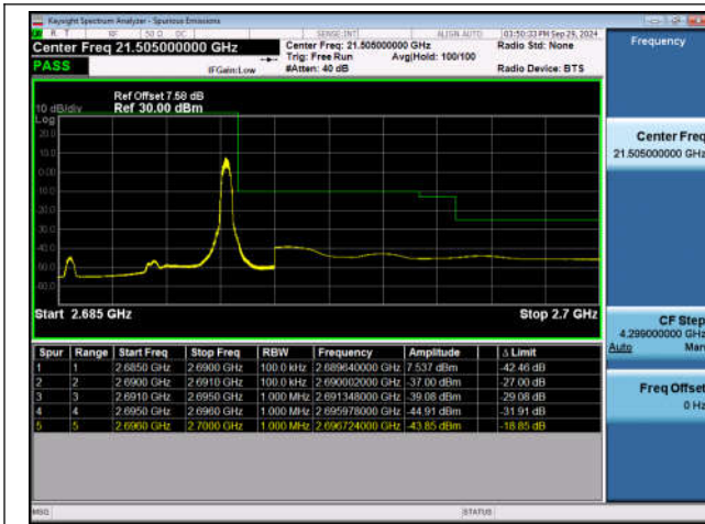
Band41_5MHz_QPSK_41565_1RB#24
