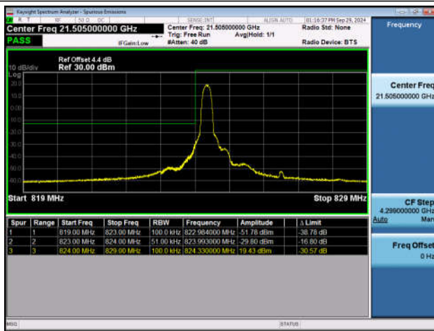
Band26_5MHz_QPSK_26815_1RB#0
