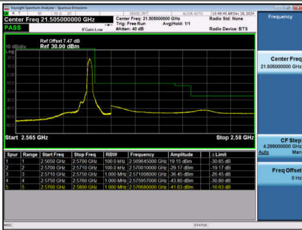
Band7_5MHz_QPSK_21425_1RB#24
