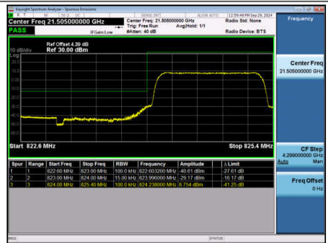
Band26_1.4MHz_QPSK_26797_6RB#0
