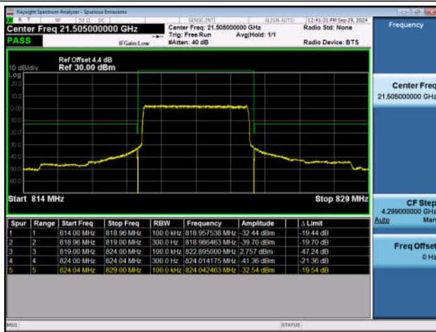
Band26_5MHz_QPSK_26765_25RB#0
