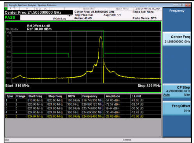
Band26_3MHz_QPSK_26775_1RB#14
