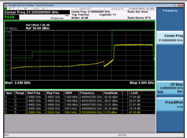
Band7_5MHz_QPSK_20775_25RB#0
