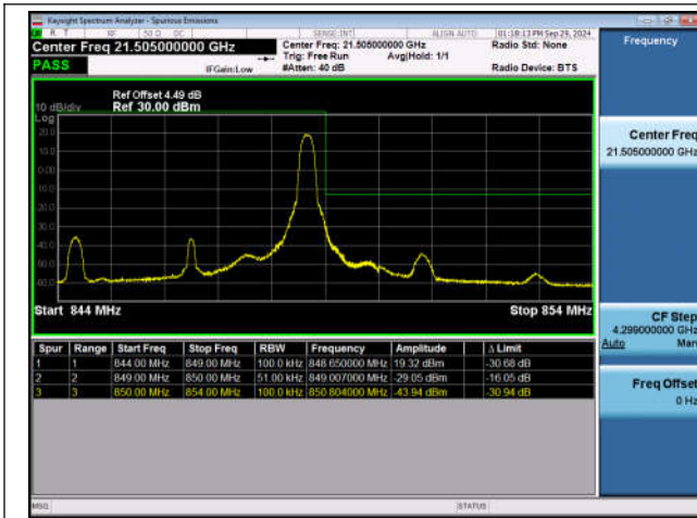
Band26_5MHz_QPSK_27015_1RB#24
