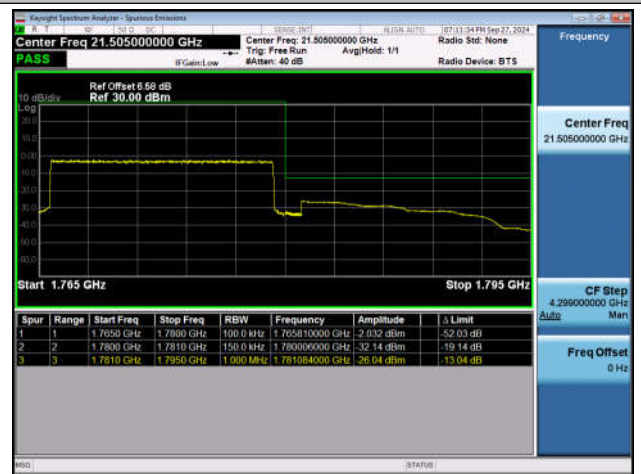
Band66_15MHz_QPSK_132597_75RB#0
