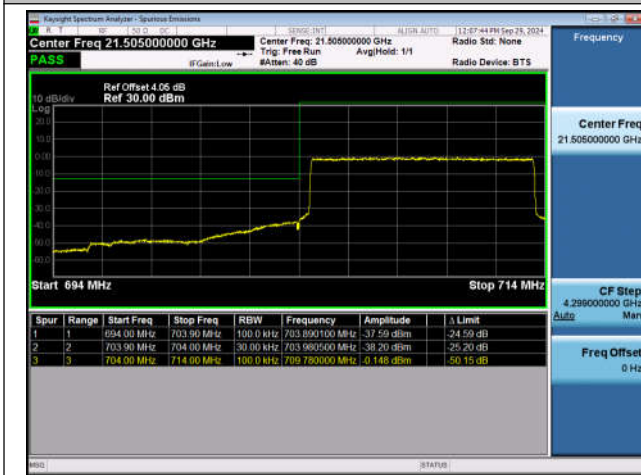
Band17_10MHz_QPSK_23780_50RB#0
