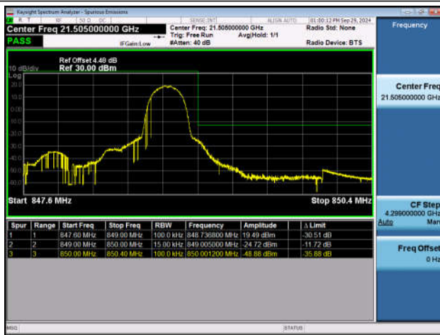
Band26_1.4MHz_QPSK_27033_1RB#5
