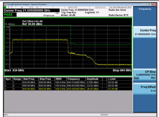
Band26_15MHz_QPSK_26965_75RB#0
