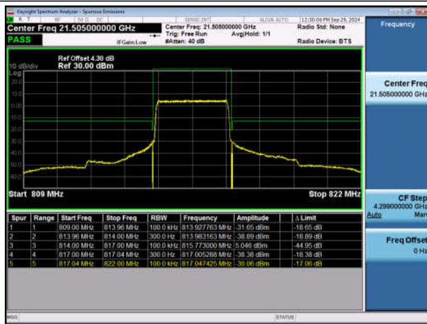
Band26_3MHz_QPSK_26705_15RB#0
