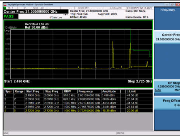
20MHz-15MHz_QPSK@QPSK-QPSK@QPSK_39750-399 21_1RB#0@100RB#0-1RB#74@75RB#0
