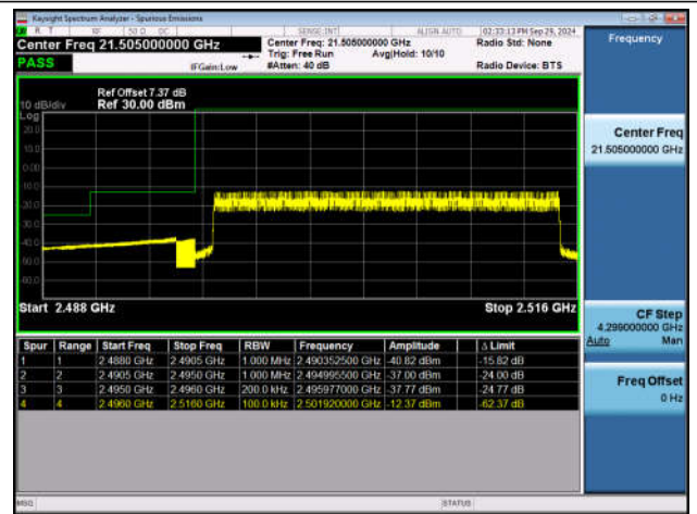
Band41_20MHz_QPSK_39750_100RB#0
