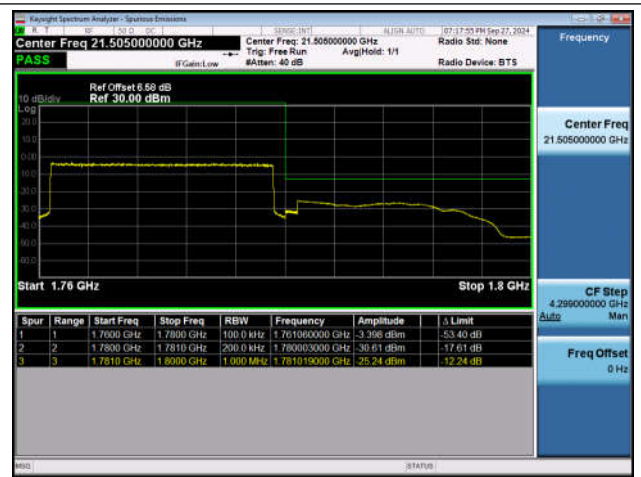
Band66_20MHz_QPSK_132572_100RB#0
