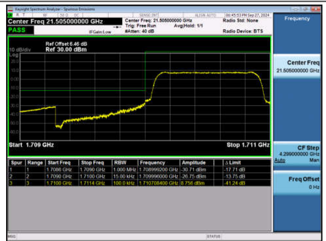
Band66_1.4MHz_QPSK_131979_6RB#0
