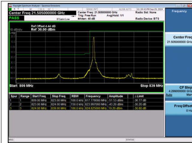
Band26_15MHz_QPSK_26865_1RB#0
