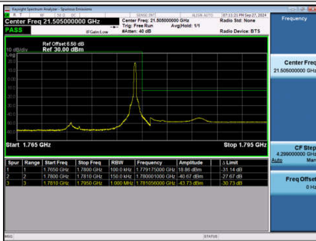
Band66_15MHz_QPSK_132597_1RB#74
