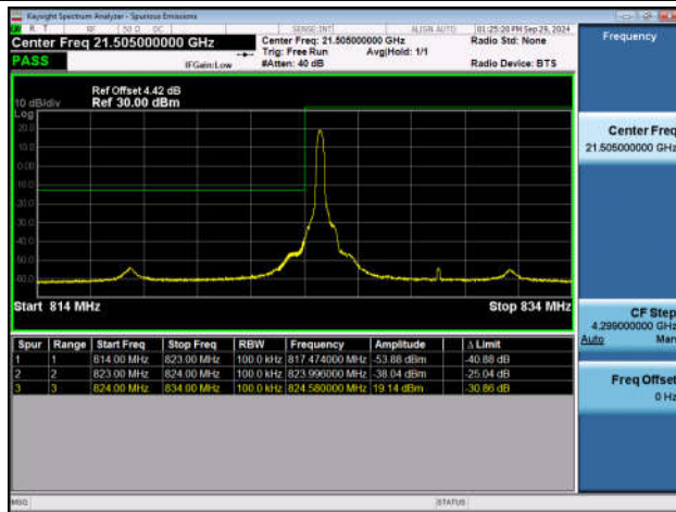
Band26_10MHz_QPSK_26840_1RB#0
