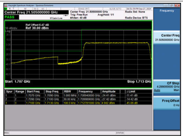
Band66_3MHz_QPSK_131987_15RB#0
