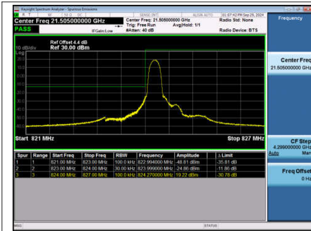
Band26_3MHz_QPSK_26805_1RB#0
