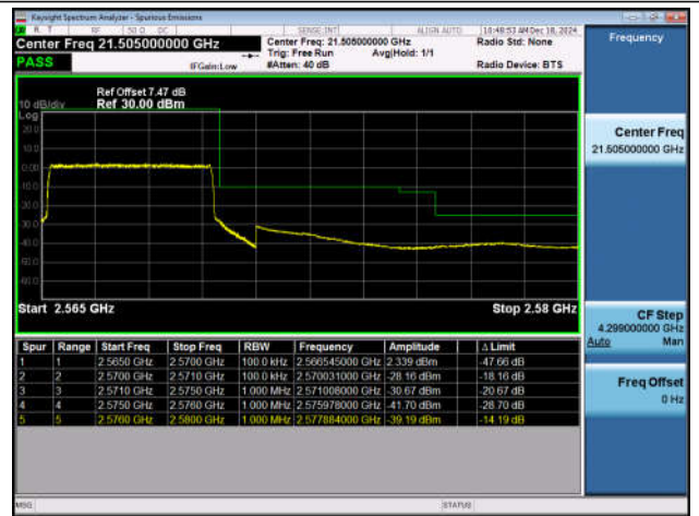
Band7_5MHz_QPSK_21425_25RB#0
