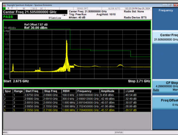
Band41_15MHz_QPSK_41515_1RB#74
