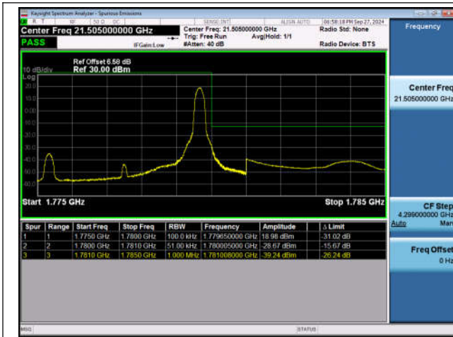
Band66_5MHz_QPSK_132647_1RB#24
