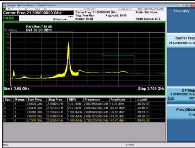
Band41_10MHz_QPSK_41540_1RB#49
