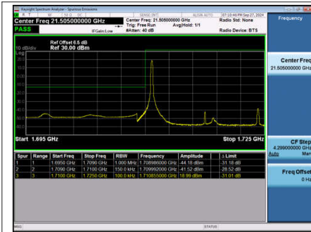
Band66_15MHz_QPSK_132047_1RB#0
