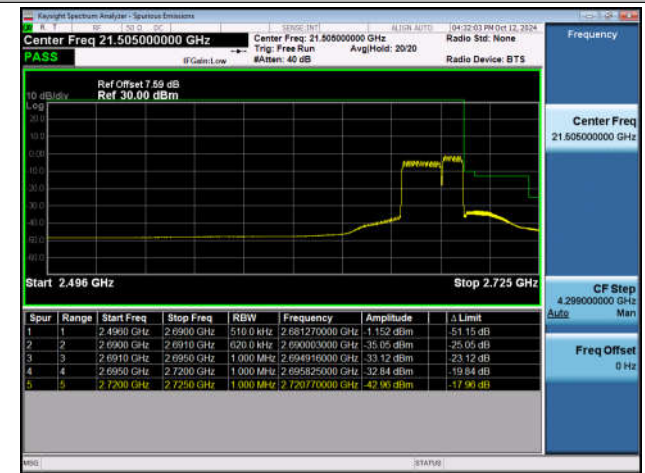
20MHz-15MHz_QPSK@QPSK-QPSK@QPSK_39750-3992 1_100RB#0@100RB#0-75RB#0@75RB#0
