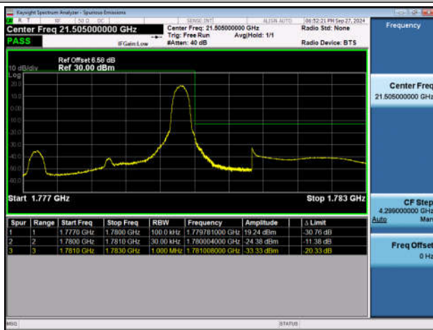
Band66_3MHz_QPSK_132657_1RB#14
