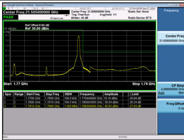
Band66_10MHz_QPSK_132622_1RB#49
