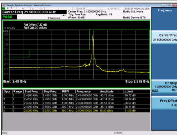
Band7_15MHz_QPSK_20825_1RB#0
