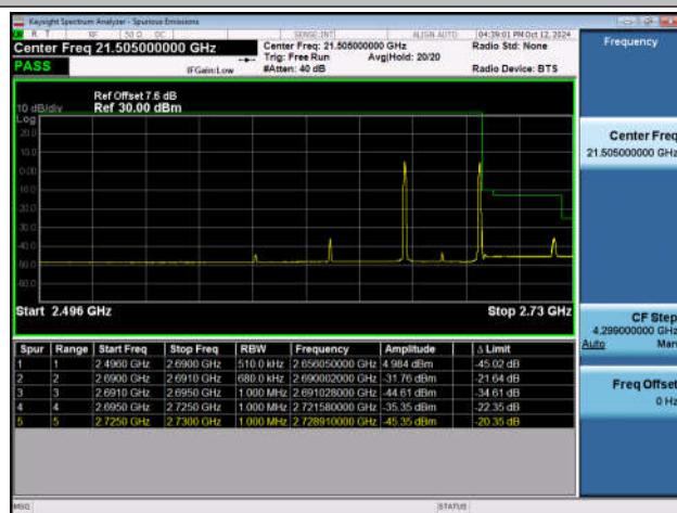
20MHz-15MHz_QPSK@QPSK-QPSK@QPSK_41341-415 12_1RB#0@100RB#0-1RB#74@75RB#0
