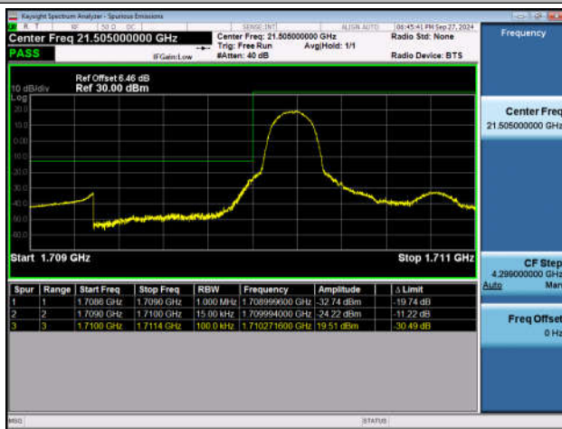
Band66_1.4MHz_QPSK_131979_1RB#0
