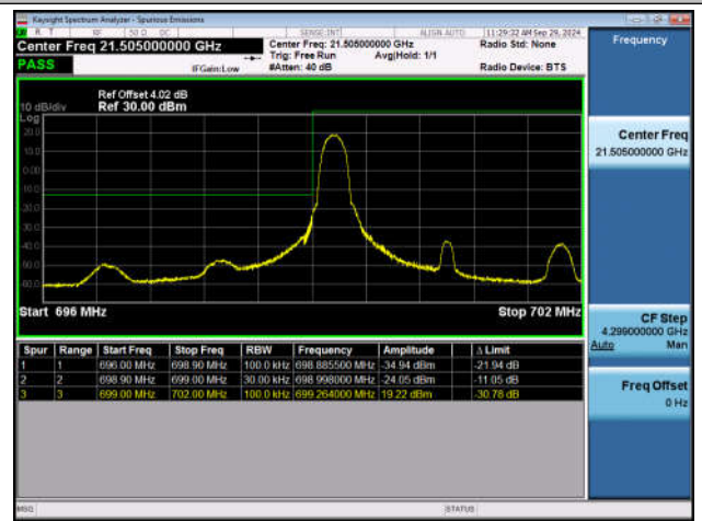
Band12_3MHz_QPSK_23025_1RB#0
