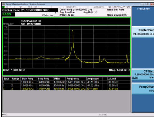
Band2_15MHz_QPSK_18675_1RB#0
