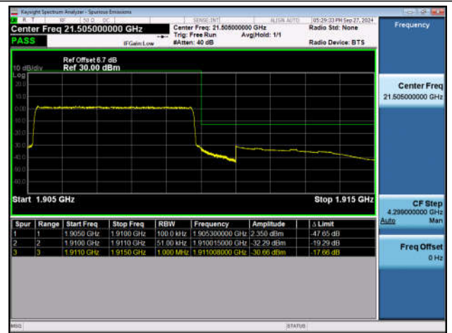
Band2_5MHz_QPSK_19175_25RB#0
