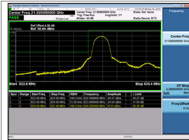
Band5_1.4MHz_QPSK_20407_1RB#0
