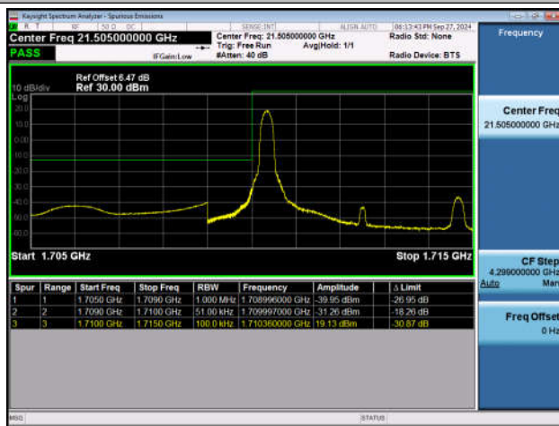
Band4_5MHz_QPSK_19975_1RB#0
