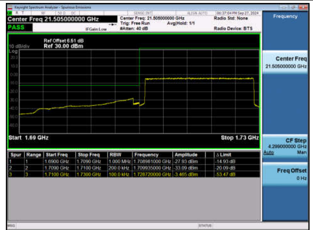
Band4_20MHz_QPSK_20050_100RB#0
