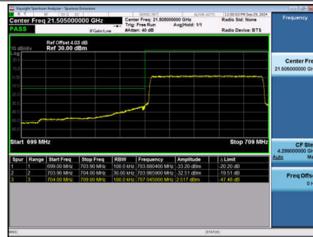
Band17_5MHz_QPSK_23755_25RB#0
