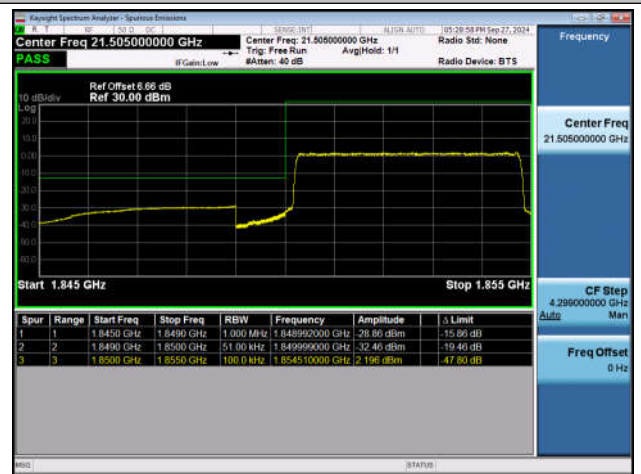
Band2_5MHz_QPSK_18625_25RB#0
