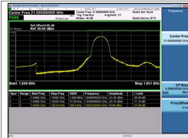
Band2_1.4MHz_QPSK_18607_1RB#0
