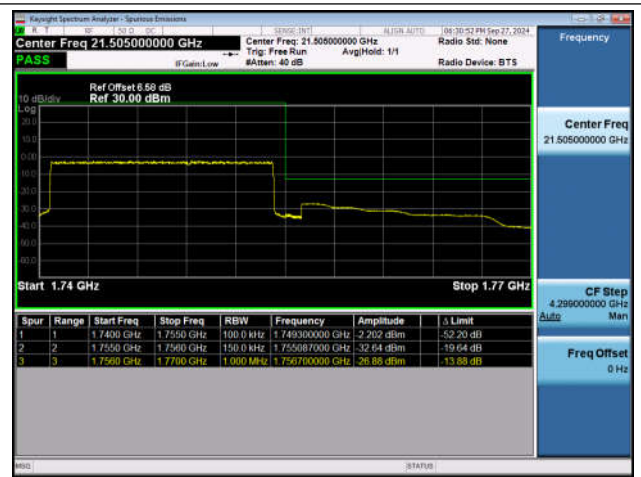
Band4_15MHz_QPSK_20325_75RB#0
