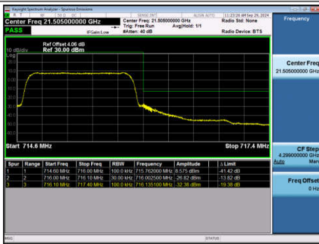
Band12_1.4MHz_QPSK_23173_6RB#0
