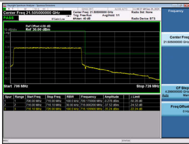
Band12_10MHz_QPSK_23130_50RB#0
