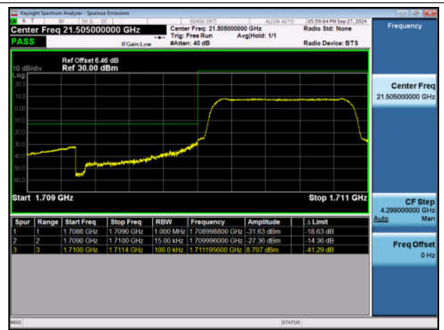
Band4_1.4MHz_QPSK_19957_6RB#0
