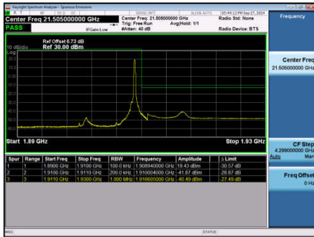
Band2_20MHz_QPSK_19100_1RB#99
