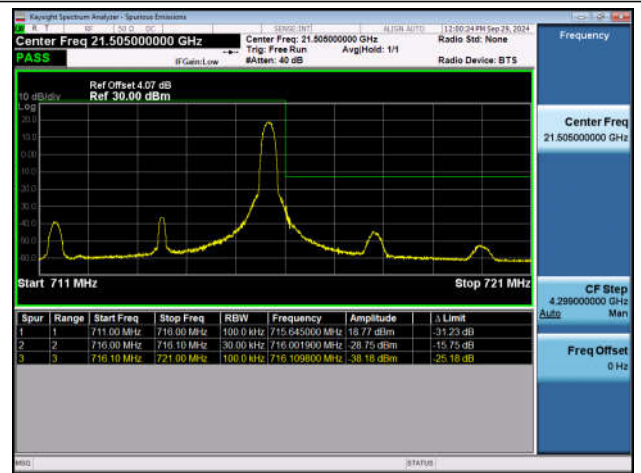
Band17_5MHz_QPSK_23825_1RB#24
