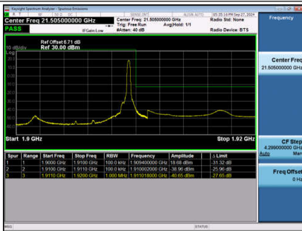
Band2_10MHz_QPSK_19150_1RB#49
