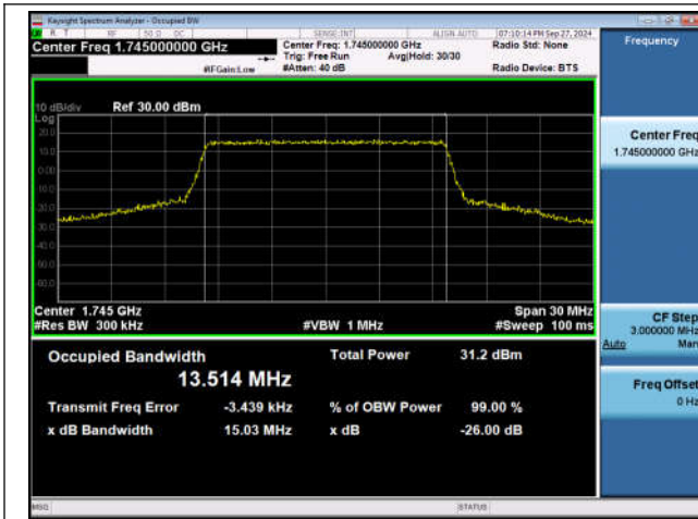
Band66-15MHz-QPSK-132322-75RB#0-PASS
