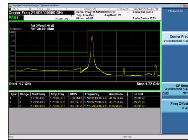
Band4_10MHz_QPSK_20000_1RB#0
