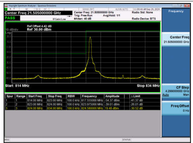
Band5_10MHz_QPSK_20450_1RB#0
