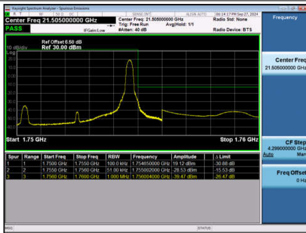
Band4_5MHz_QPSK_20375_1RB#24
