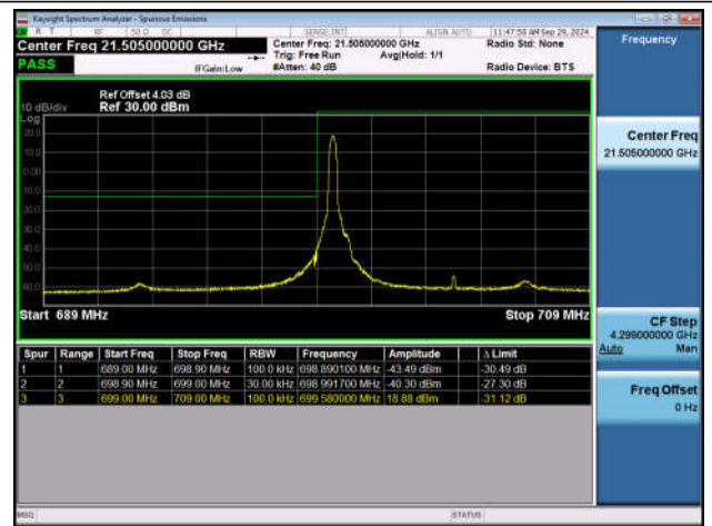
Band12_10MHz_QPSK_23060_1RB#0
