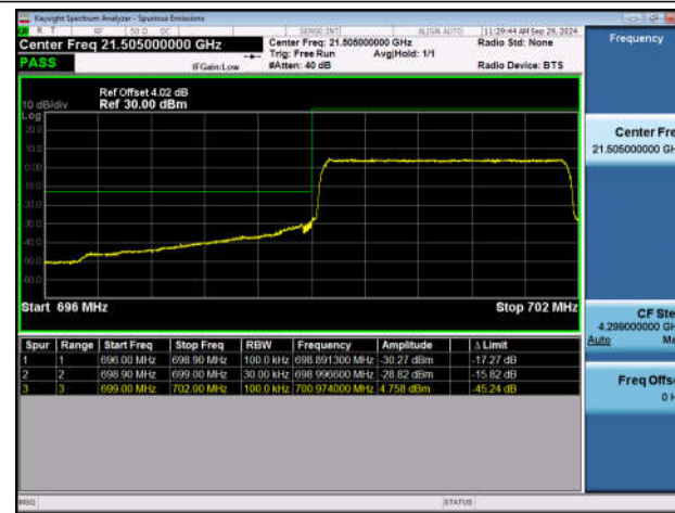
Band12_3MHz_QPSK_23025_15RB#0
