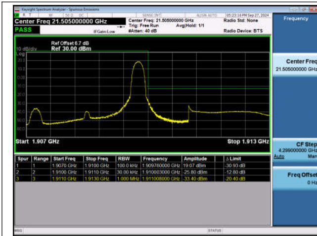
Band2_3MHz_QPSK_19185_1RB#14
