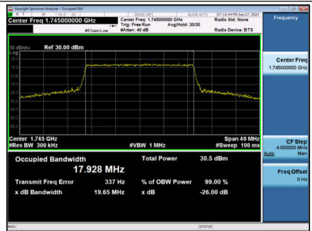
Band66-20MHz-16QAM-132322-100RB#0-PASS
