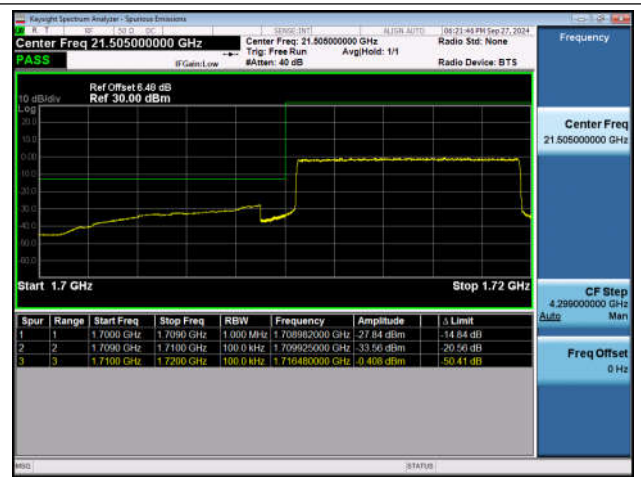
Band4_10MHz_QPSK_20000_50RB#0
