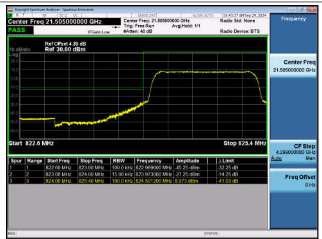
Band5_1.4MHz_QPSK_20407_6RB#0
