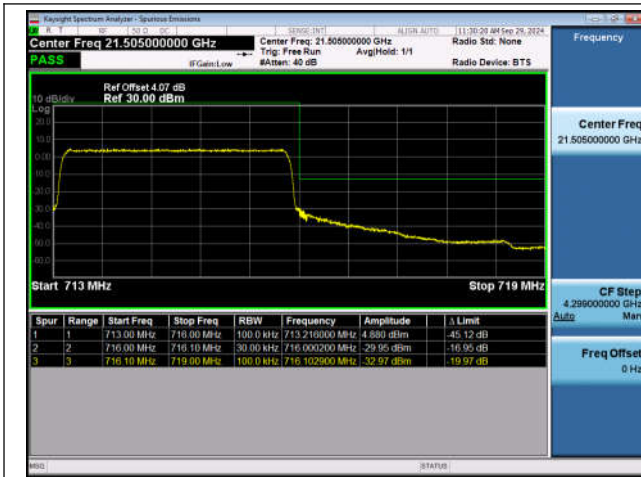
Band12_3MHz_QPSK_23165_15RB#0
