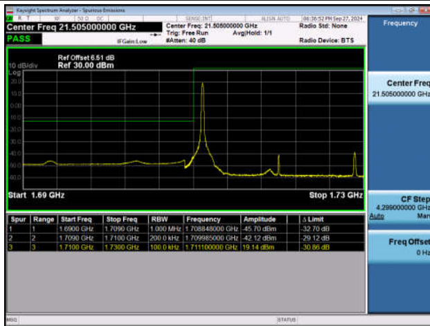
Band4_20MHz_QPSK_20050_1RB#0
