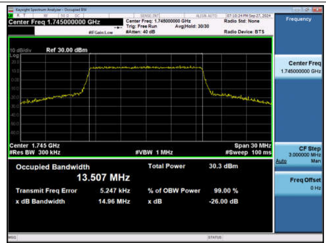
Band66-15MHz-16QAM-132322-75RB#0-PASS
