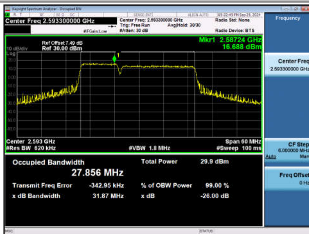
41-41-10MHz-20MHz-QPSK-QPSK-40526-40670-50RB#0-100RB#0-PASS
