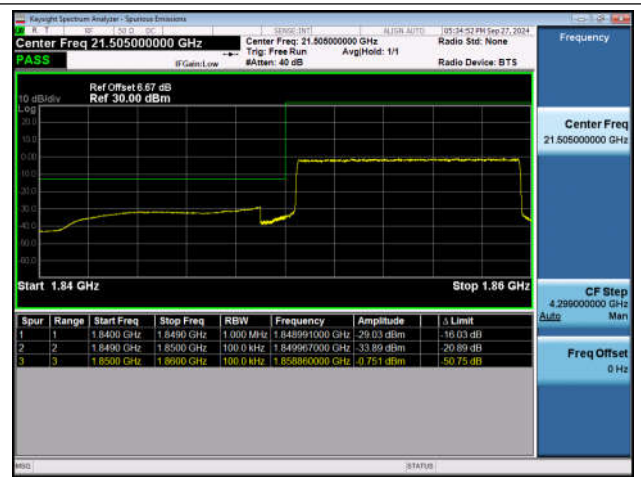
Band2_10MHz_QPSK_18650_50RB#0
