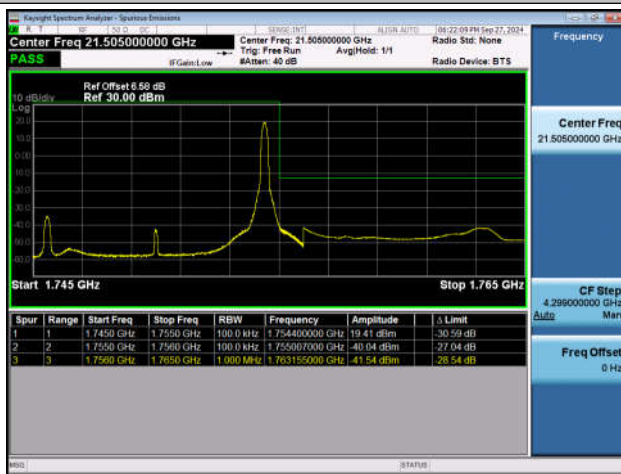
Band4_10MHz_QPSK_20350_1RB#49
