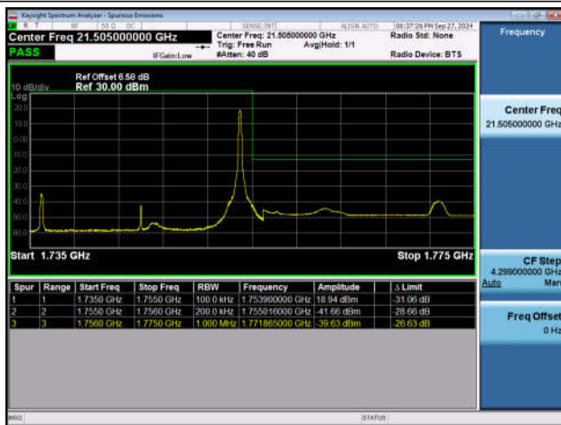
Band4_20MHz_QPSK_20300_1RB#99
