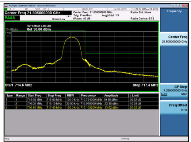
Band12_1.4MHz_QPSK_23173_1RB#5
