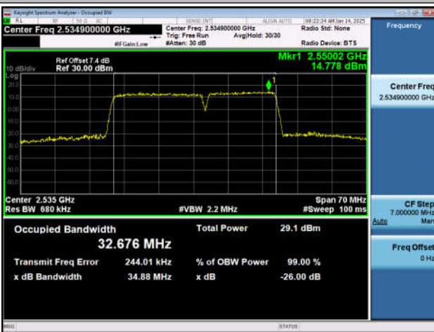
7-7-20MHz-15MHz-QPSK-QPSK-21026-21197-100RB#0-75RB#0-PASS
