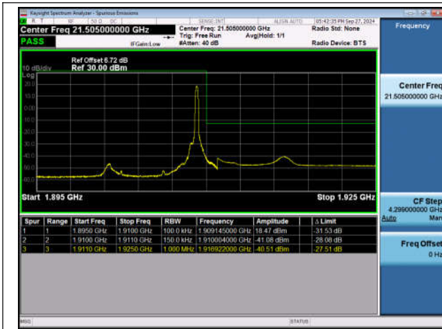
Band2_15MHz_QPSK_19125_1RB#74
