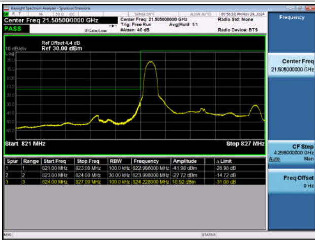
Band5_3MHz_QPSK_20415_1RB#0
