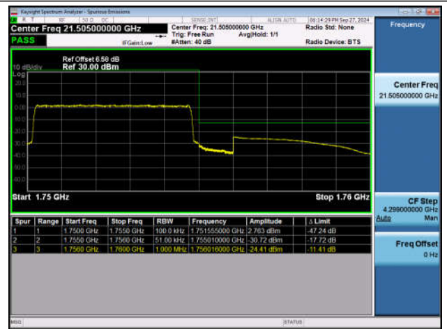
Band4_5MHz_QPSK_20375_25RB#0
