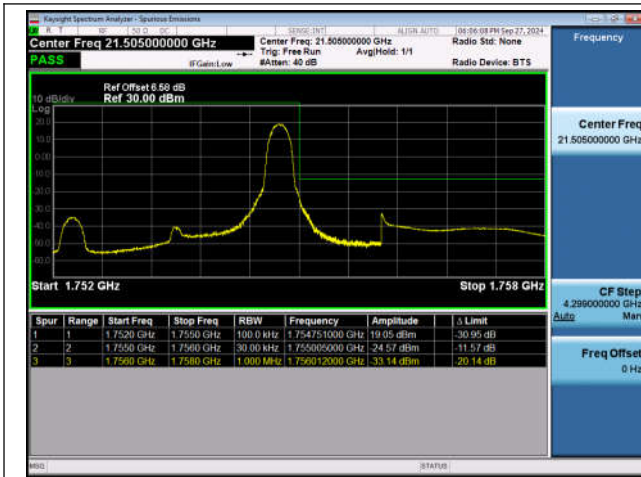
Band4_3MHz_QPSK_20385_1RB#14
