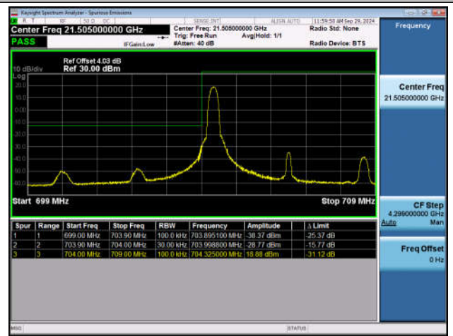
Band17_5MHz_QPSK_23755_1RB#0
