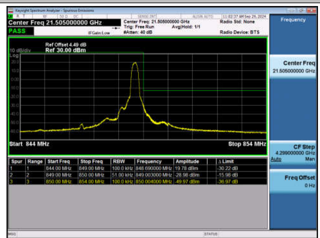
Band5_5MHz_QPSK_20625_1RB#24
