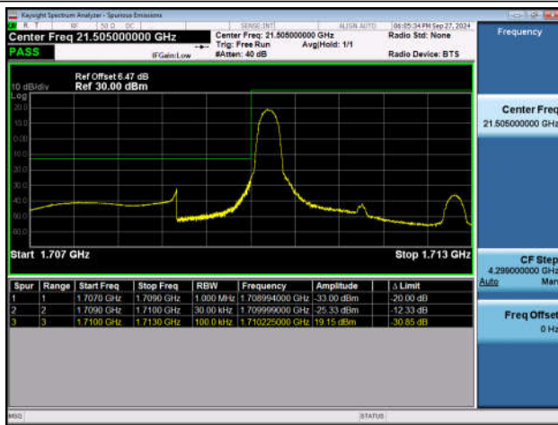
Band4_3MHz_QPSK_19965_1RB#0
