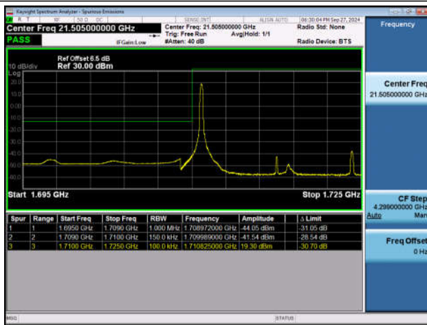
Band4_15MHz_QPSK_20025_1RB#0
