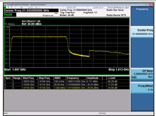
Band2_3MHz_QPSK_19185_15RB#0
