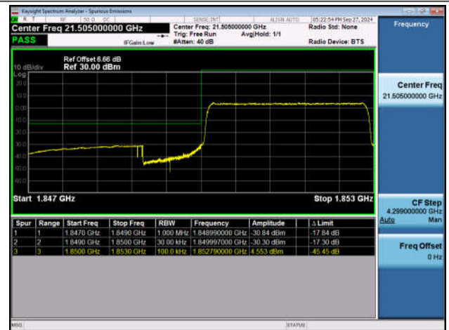
Band2_3MHz_QPSK_18615_15RB#0
