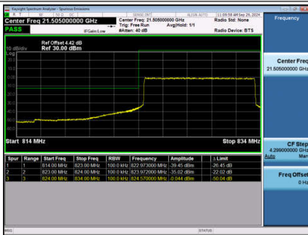
Band5_10MHz_QPSK_20450_50RB#0
