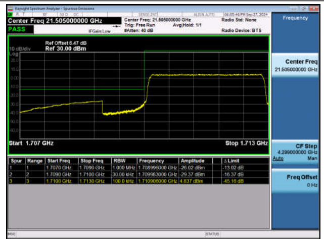
Band4_3MHz_QPSK_19965_15RB#0
