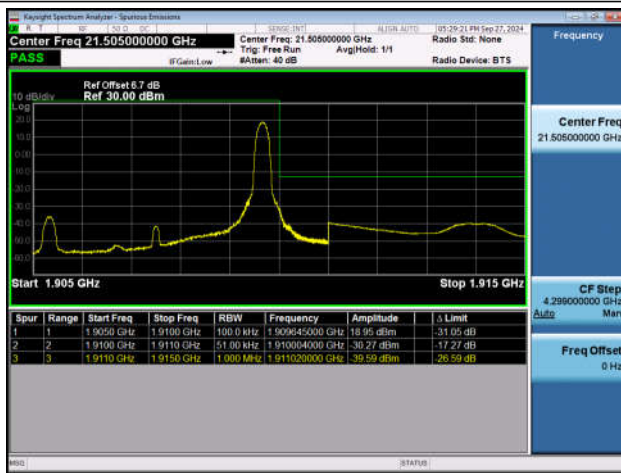
Band2_5MHz_QPSK_19175_1RB#24
