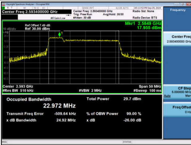
41-41-10MHz-15MHz-QPSK-QPSK-40549-40669-50RB#0-75RB#0-PASS
