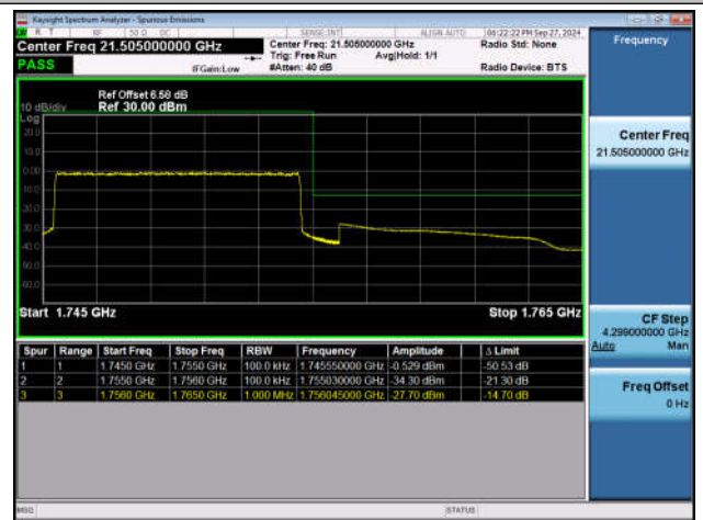
Band4_10MHz_QPSK_20350_50RB#0
