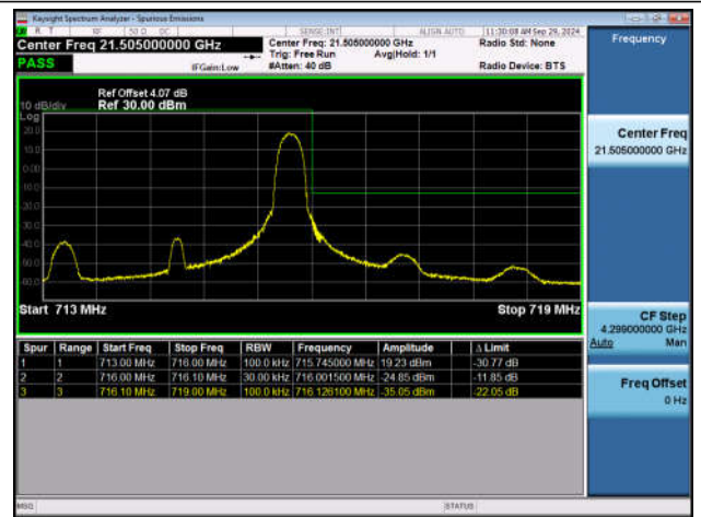
Band12_3MHz_QPSK_23165_1RB#14
