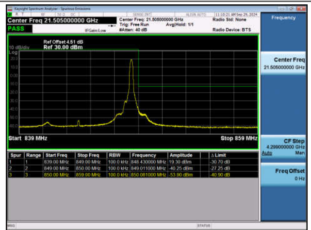
Band5_10MHz_QPSK_20600_1RB#49
