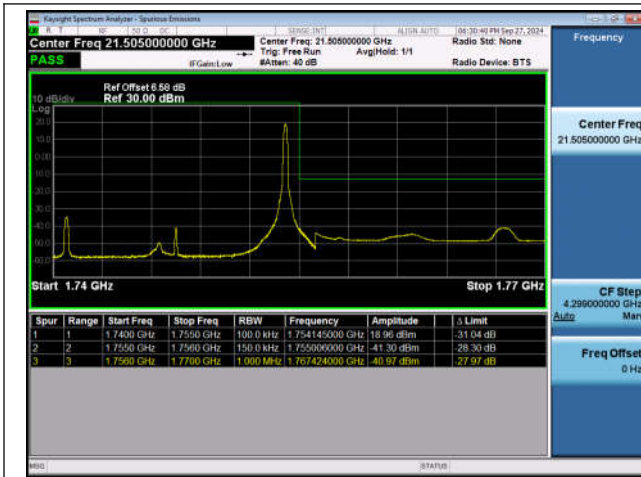
Band4_15MHz_QPSK_20325_1RB#74
