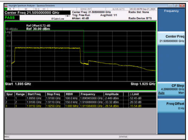
Band2_15MHz_QPSK_19125_75RB#0
