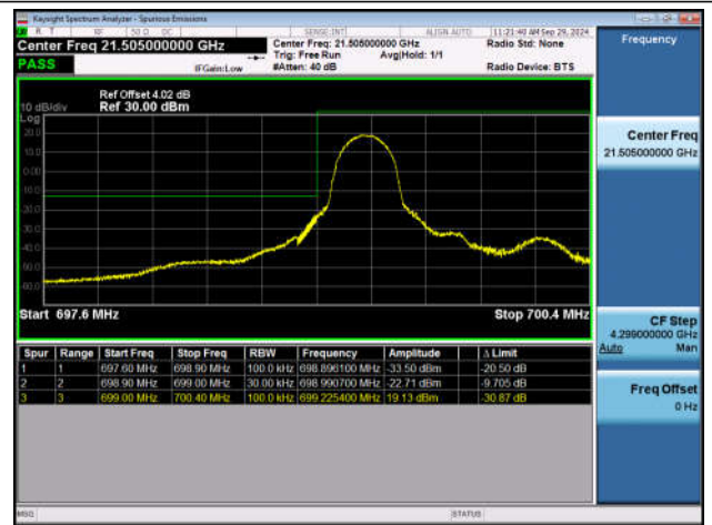
Band12_1.4MHz_QPSK_23017_1RB#0
