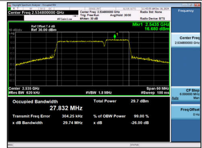
7-7-20MHz-15MHz-16QAM-16QAM-21026-21197-100RB#0-75RB#0-PASS
