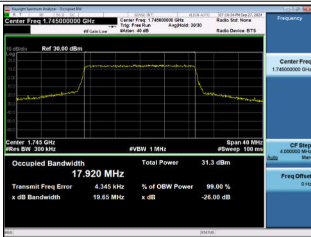
Band66-20MHz-QPSK-132322-100RB#0-PASS
