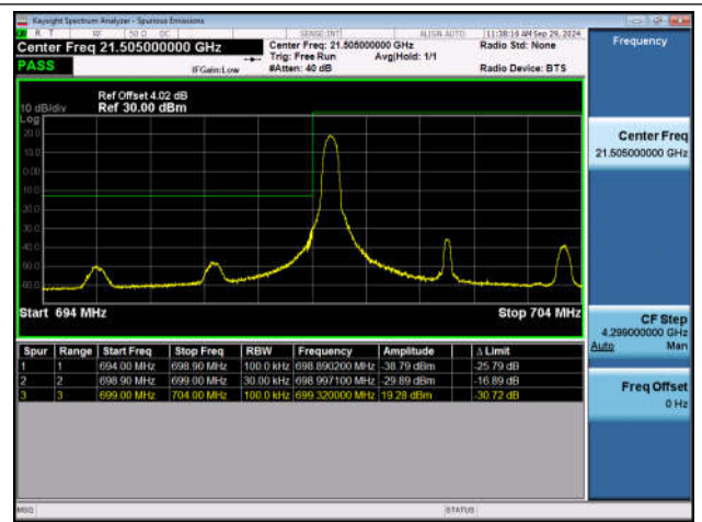
Band12_5MHz_QPSK_23035_1RB#0
