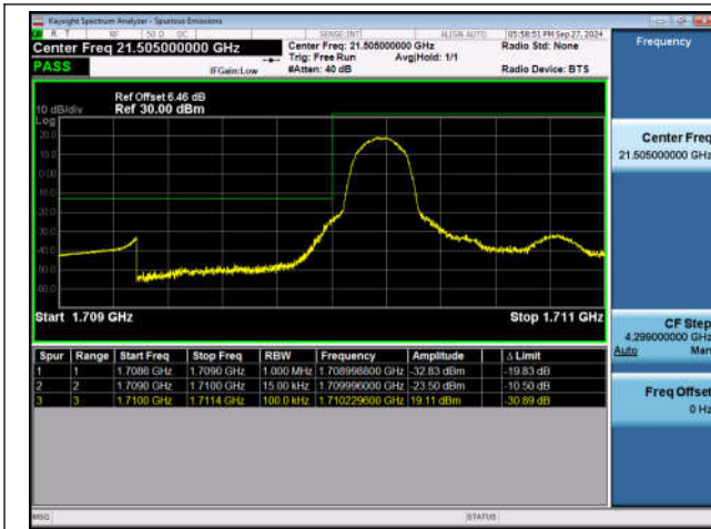
Band4_1.4MHz_QPSK_19957_1RB#0
