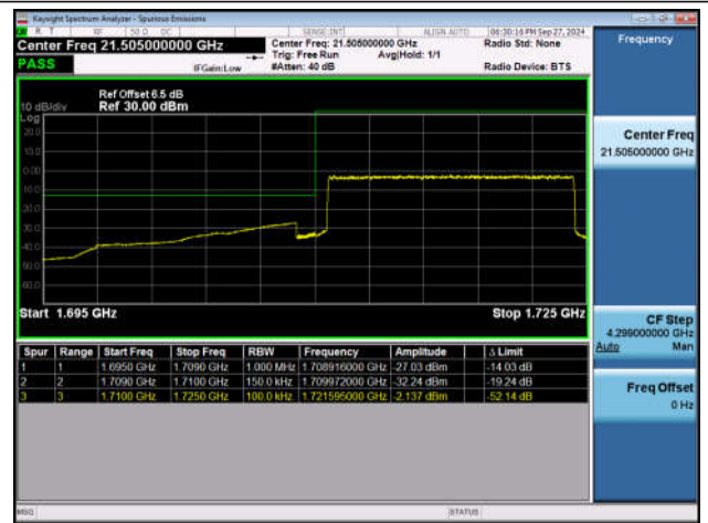
Band4_15MHz_QPSK_20025_75RB#0
