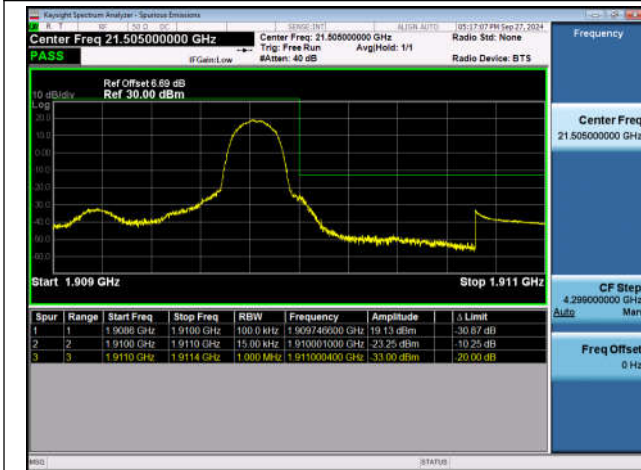
Band2_1.4MHz_QPSK_19193_1RB#5
