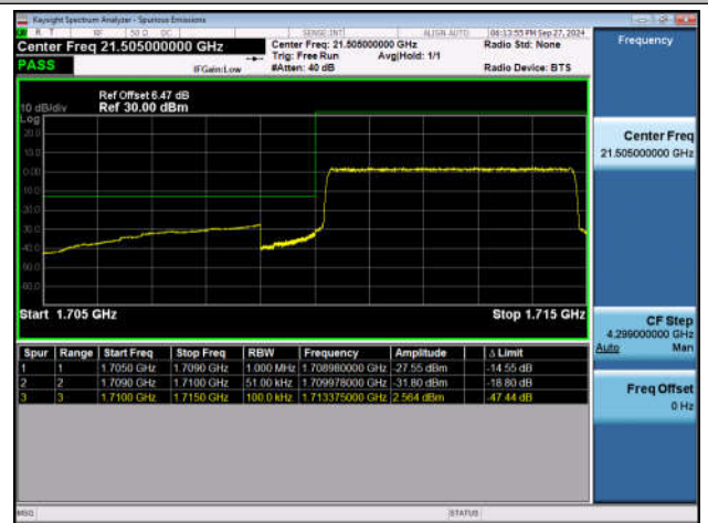
Band4_5MHz_QPSK_19975_25RB#0
