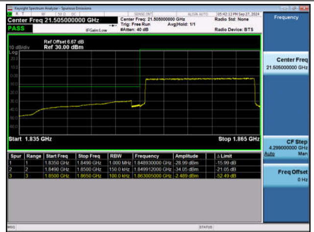
Band2_15MHz_QPSK_18675_75RB#0
