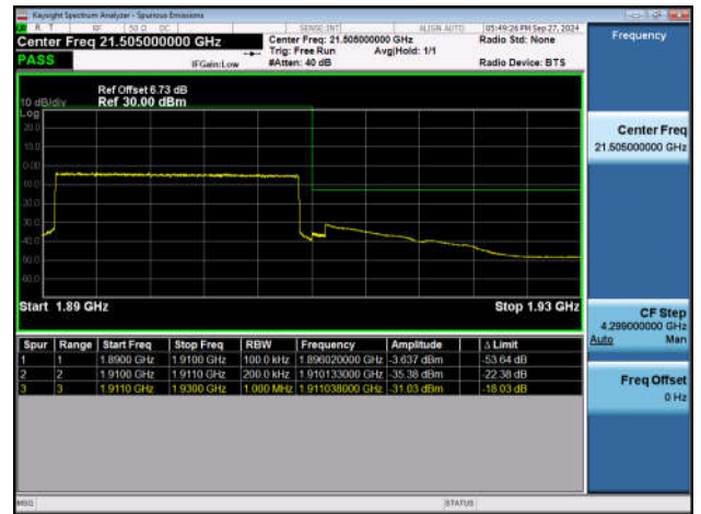
Band2_20MHz_QPSK_19100_100RB#0
