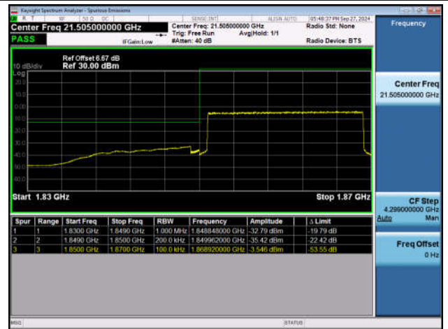
Band2_20MHz_QPSK_18700_100RB#0
