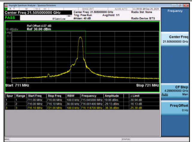
Band12_5MHz_QPSK_23155_1RB#24
