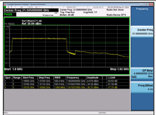
Band2_10MHz_QPSK_19150_50RB#0
