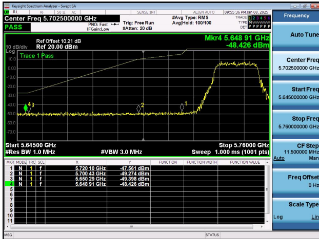
11AX20SISO-Ant1-5745-PASS
