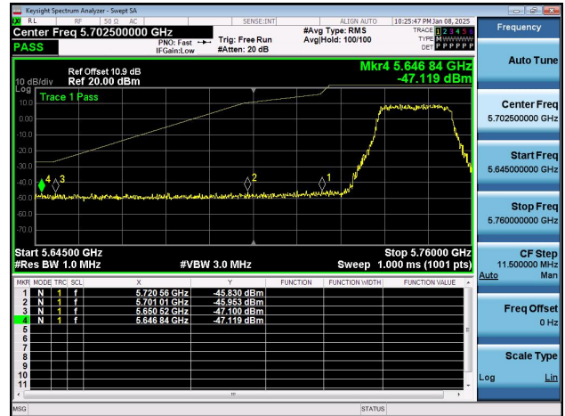
11AX20SISO-Ant2-5745-PASS
