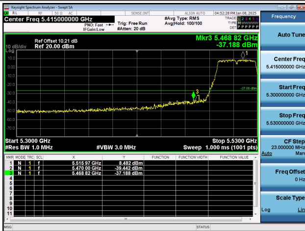
11N40SISO-Ant1-5510-PASS
