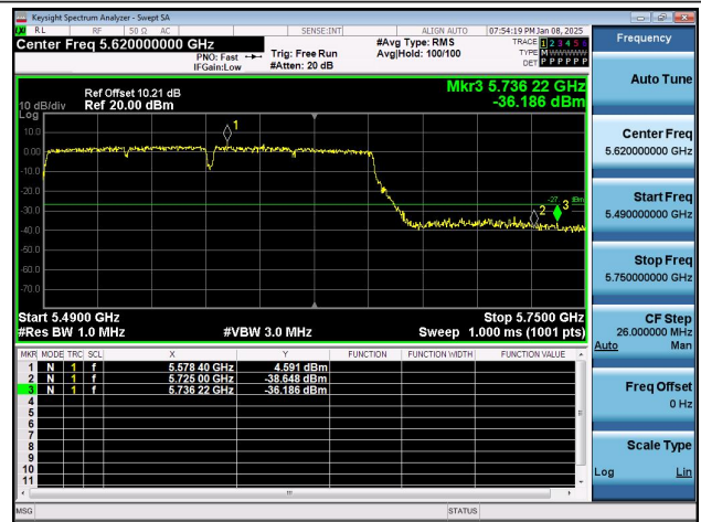
11AC160SISO-Ant2-5570-PASS
