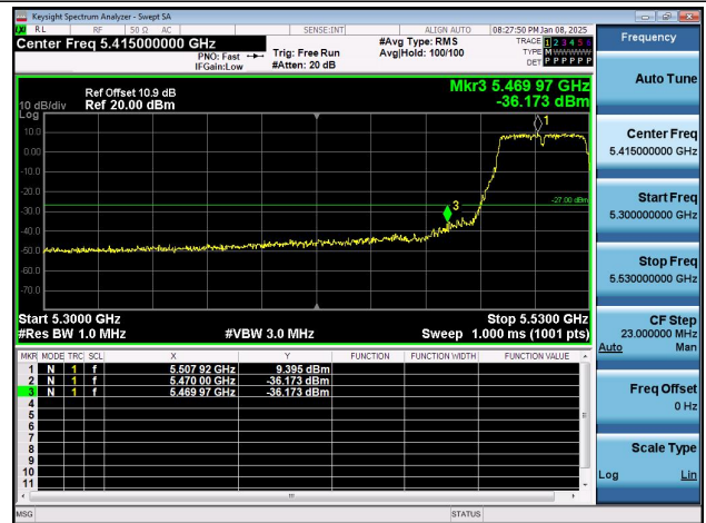
11N40SISO-Ant2-5510-PASS
