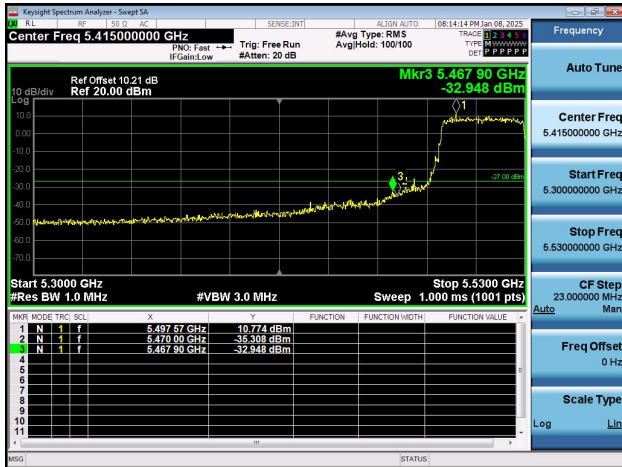
11AX40SISO-Ant1-5510-PASS
