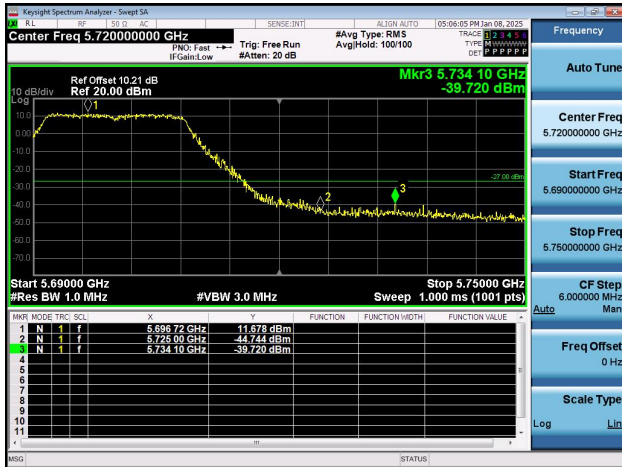
11AC20SISO-Ant1-5700-PASS
