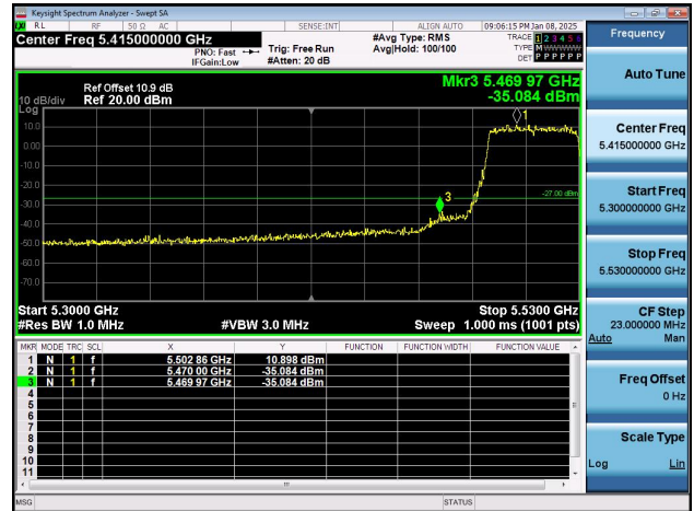
11AX40SISO-Ant2-5510-PASS
