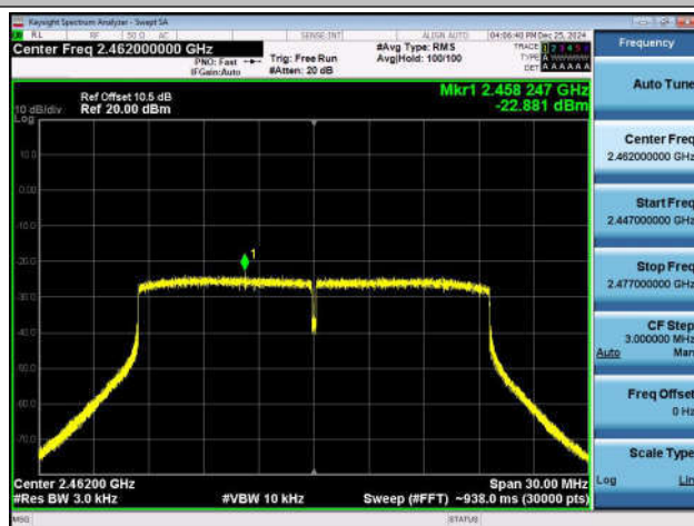
11AX20MIMO-Ant2-2462-PASS
