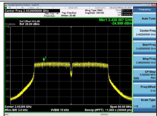
11N40MIMO-Ant2-2452-PASS
