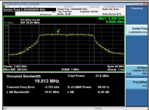
11AX20SISO-Ant2-2462
