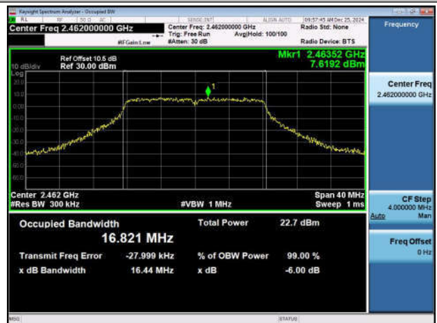
11G-Ant2-2462
