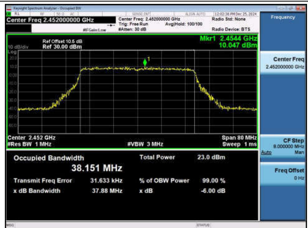
11AX40SISO-Ant2-2452
