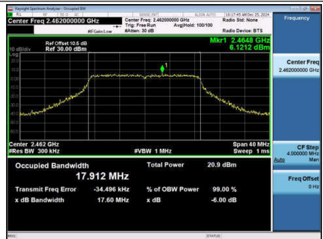
11N20SISO-Ant2-2462
