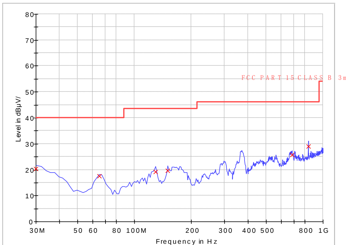
EMI Sweep-3M(30-1G)
