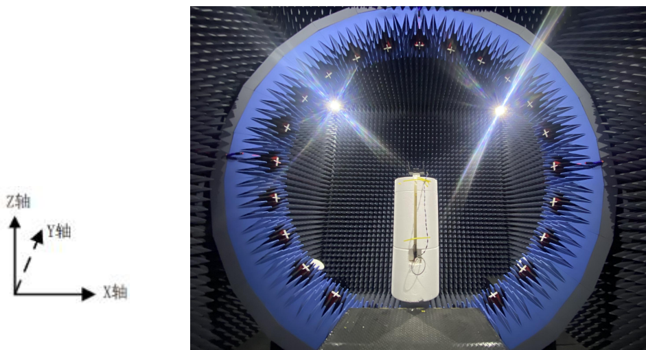
Front view
