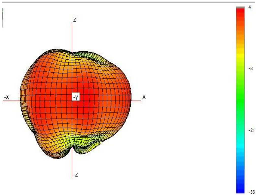
(5) Typical Free Space 3D Radiation Pattern at 5.5GHz:
