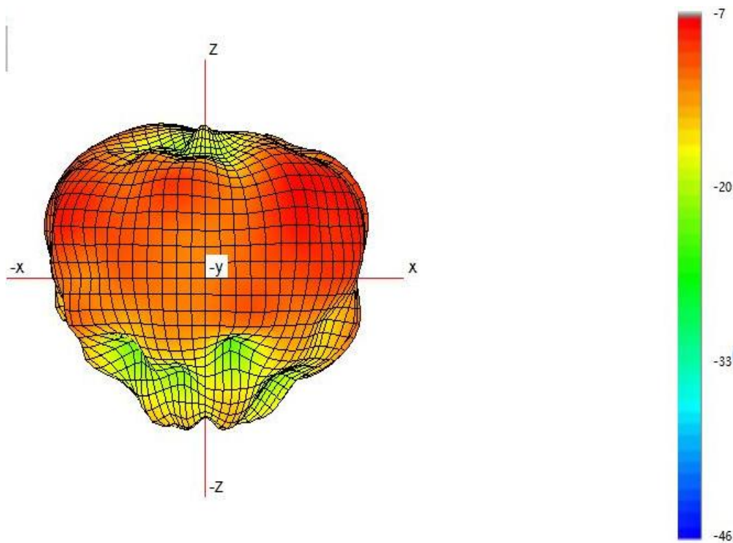
(5) Typical Free Space 3D Radiation Pattern at 5.5GHz:
