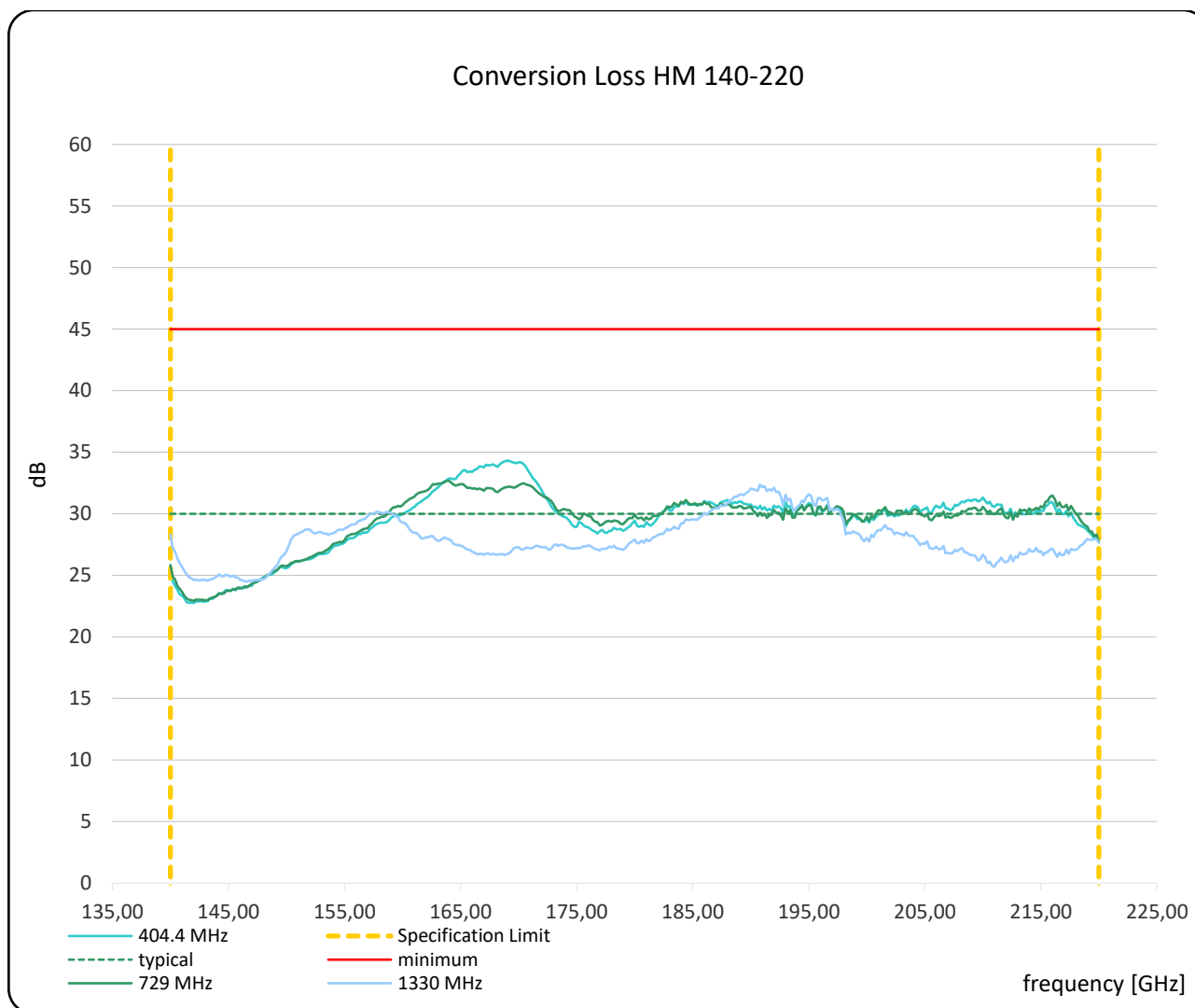
Figure 1: Measured conversion loss between 140 GHz and 220 GHz
