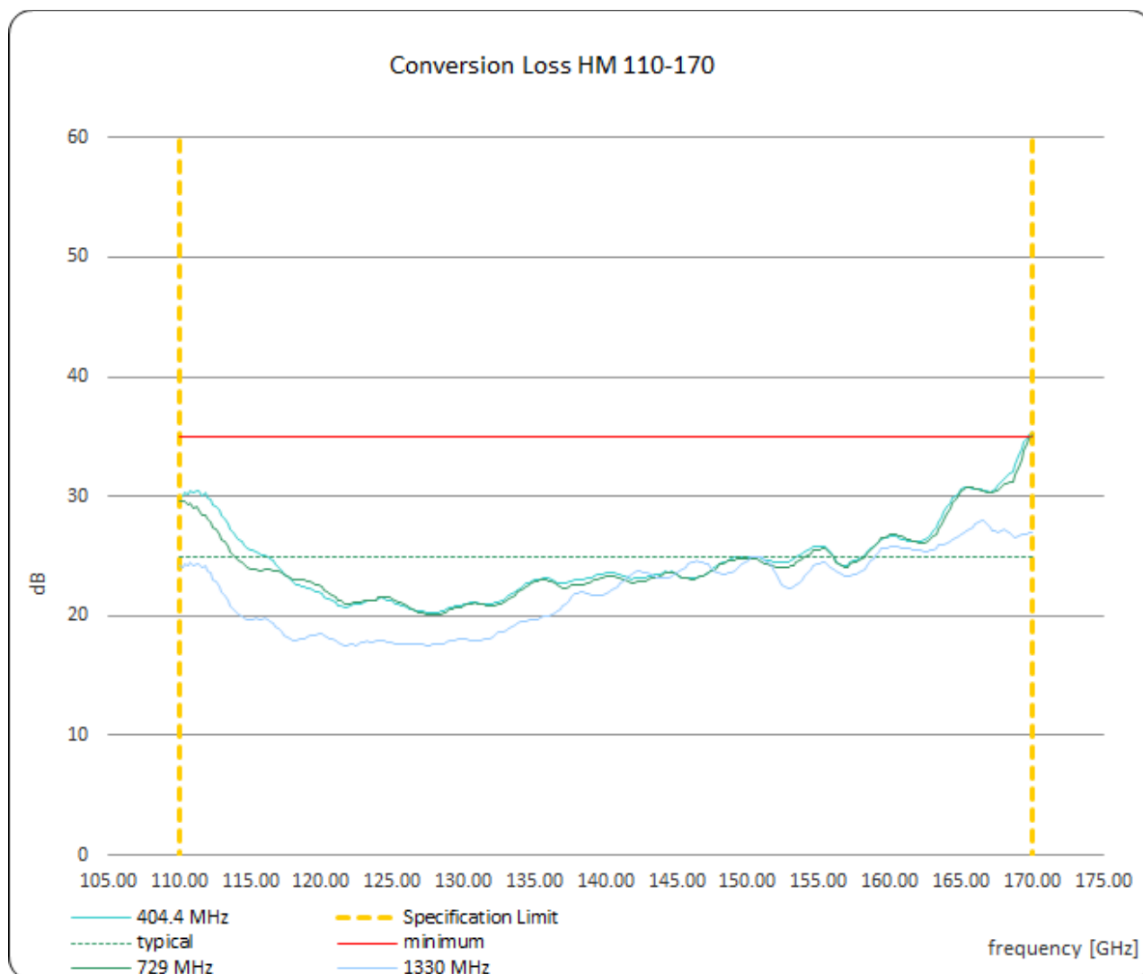
Figure 1: Measured conversion loss between 110 GHz and 170 GHz
