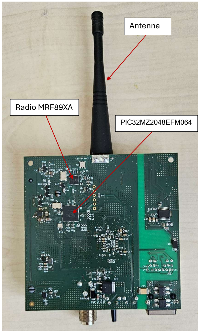
Internal bottom side
