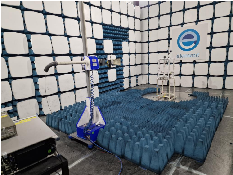
1 GHz to 10 GHz
