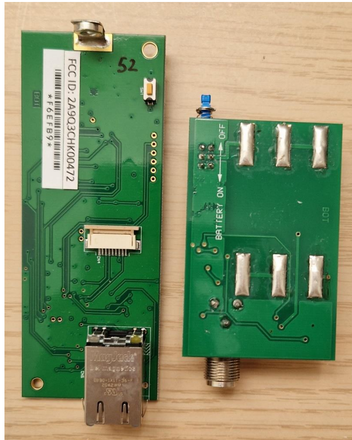
Ethernet Repeater
