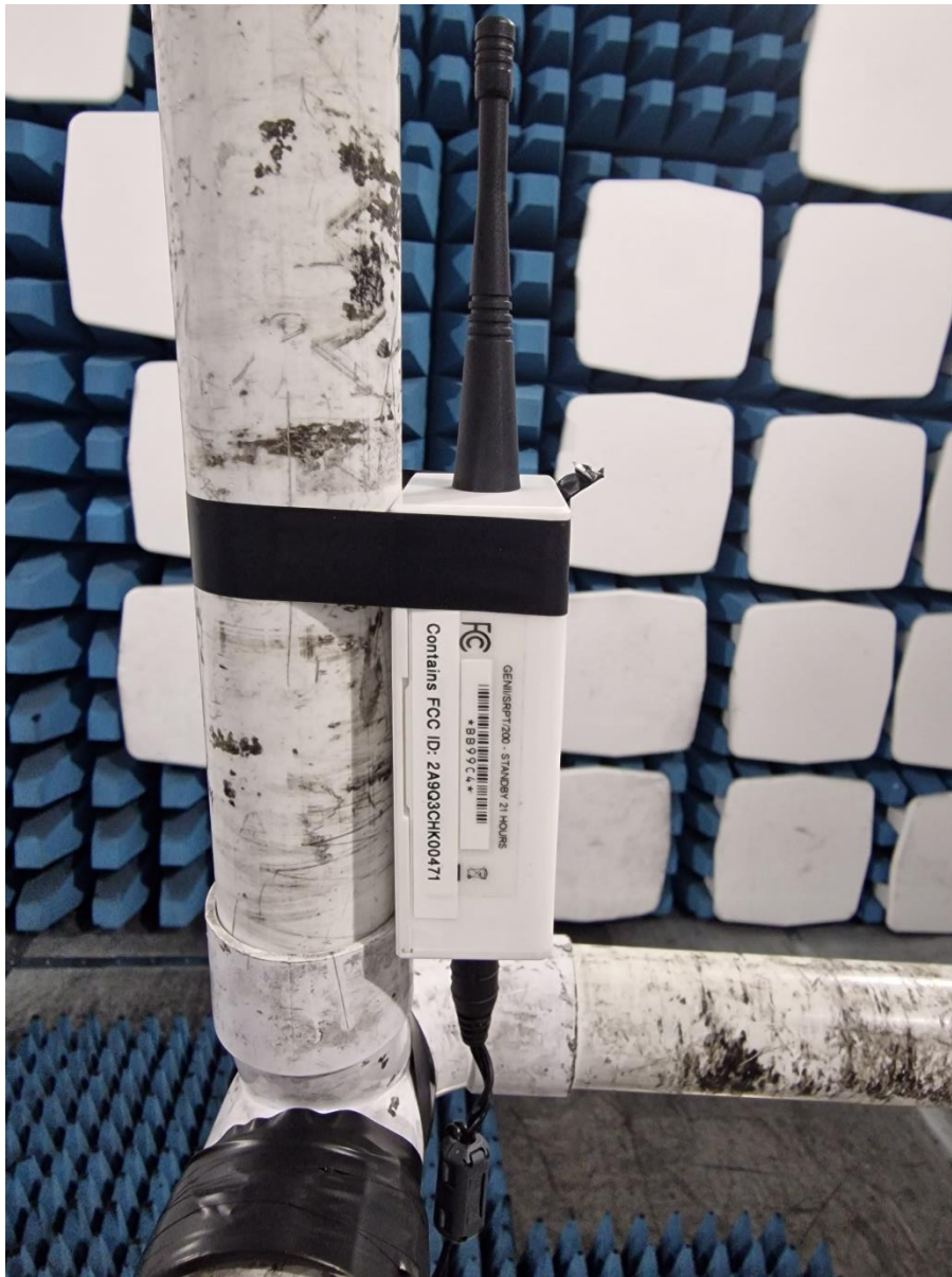
Close-up of EUT during Radiated tests
