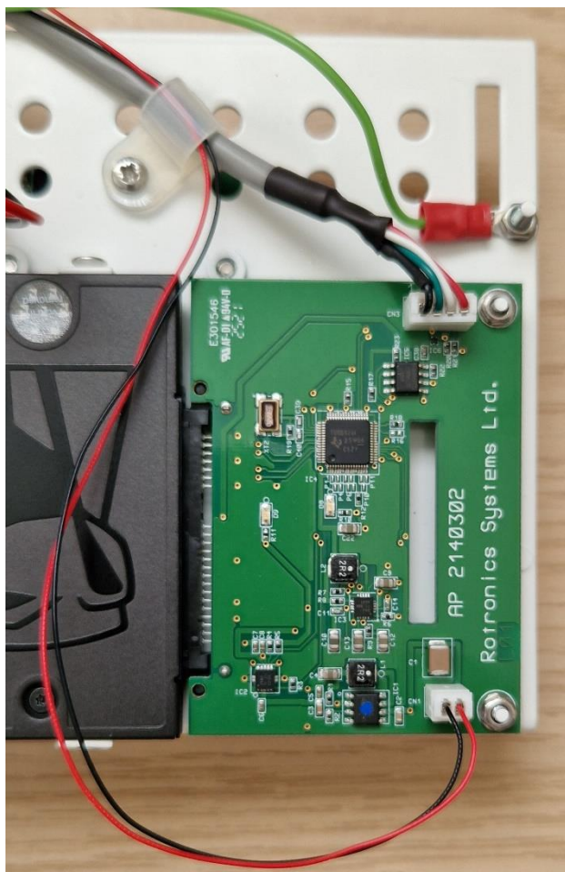
USB-SATA Adaptor PCB
