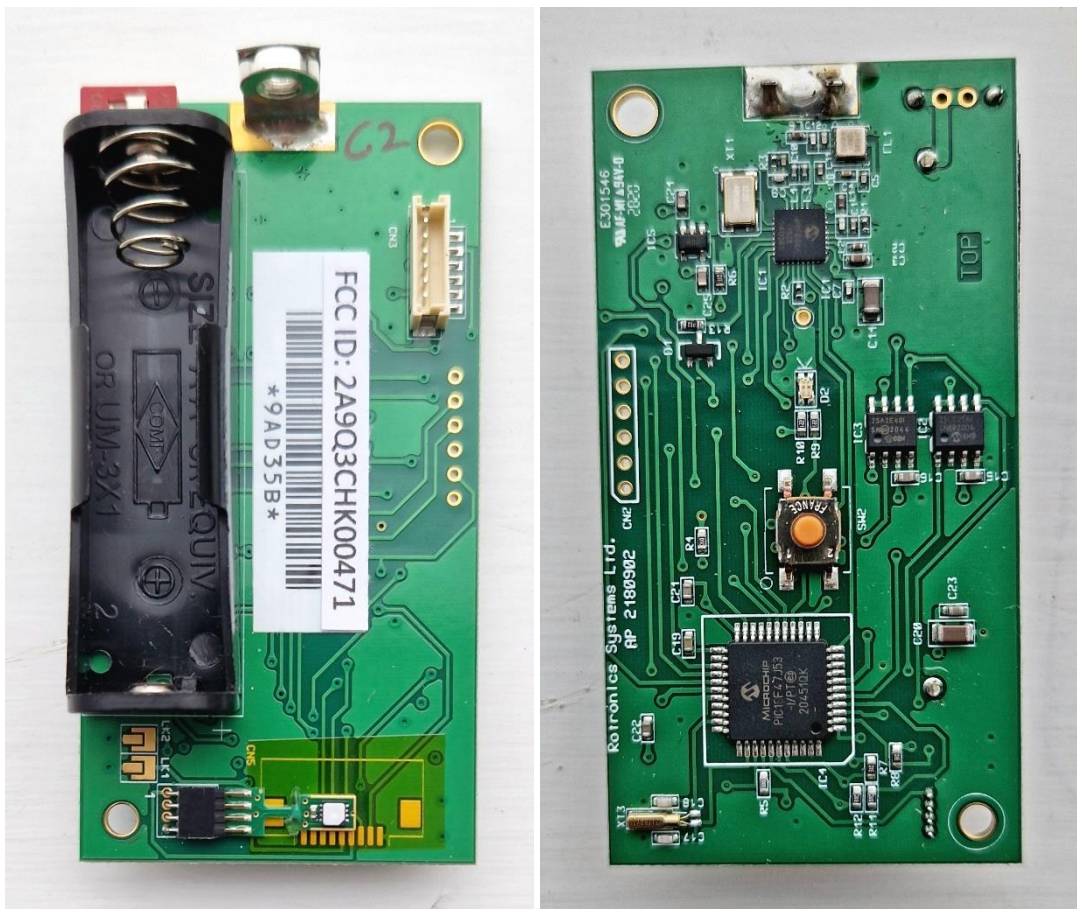
Ambient Transmitter: GENII/AMB/200EA
