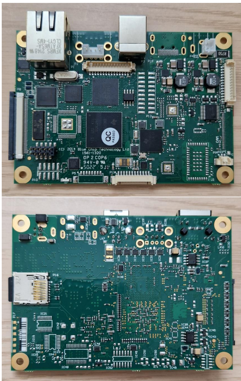
WARP Single Board Computer RE2G2
