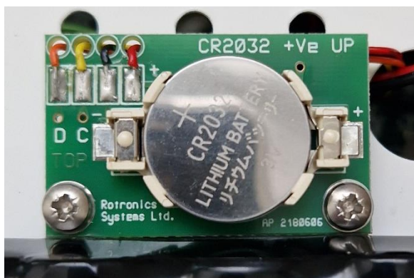
RTC & CMOS Battery PCB
