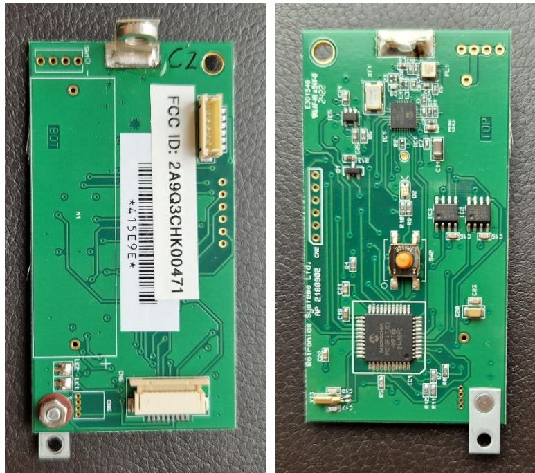
WARP RF transmitter module
