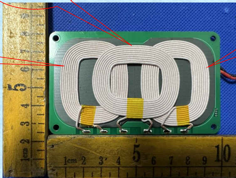
WPT Antennna TX 2
