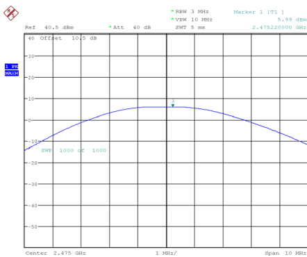
2475 MHz
