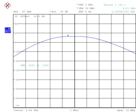
2440 MHz
