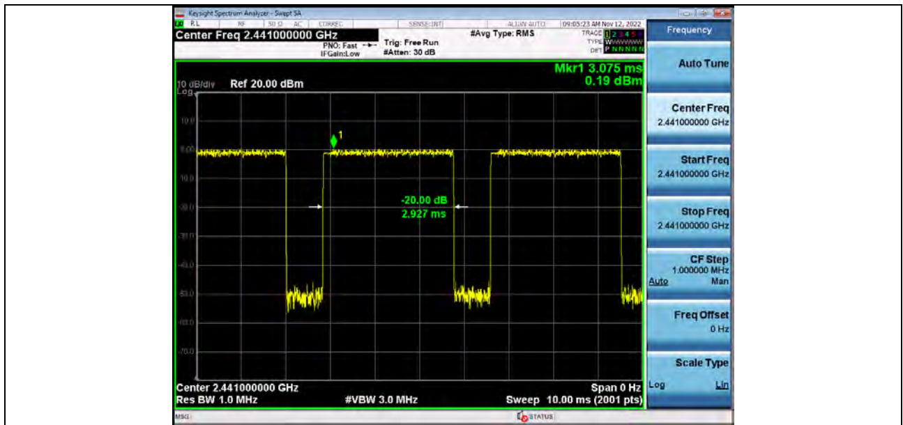
Dwell_Time_(Hopping)_BT_1-DH1_2441_One_Burst_Time
