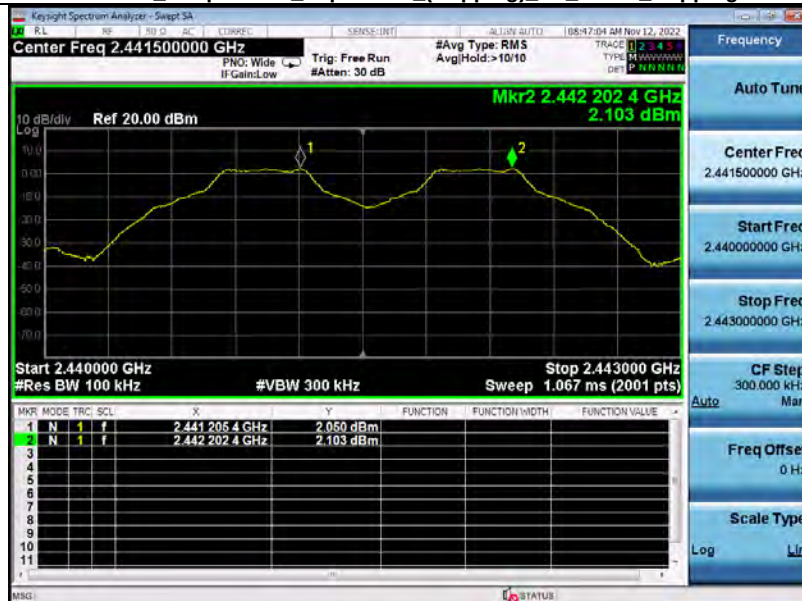
Carrier_Frequencies_Separation_(Hopping)_BT_1-DH5_Hopping
