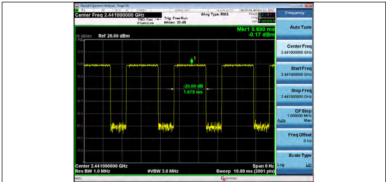
Dwell_Time (Hopping) BT_3-DH1_2441_One_Burst_Time
