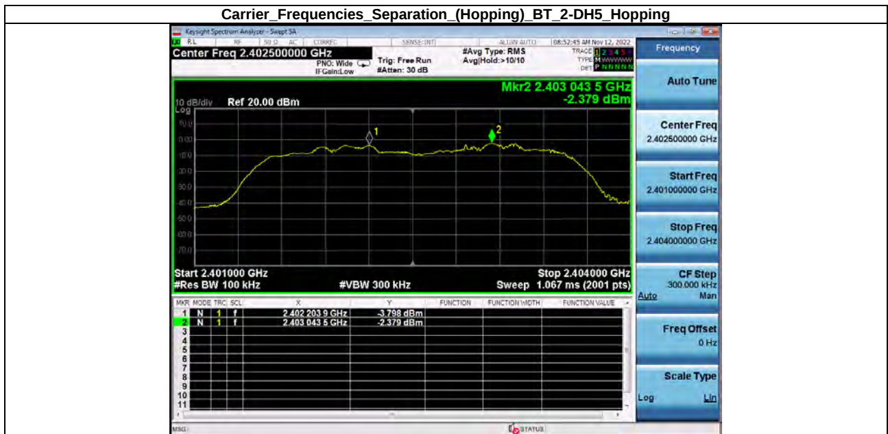
Carrier_Frequencies_Separation_(Hopping)_BT_2-DH5_Hopping
