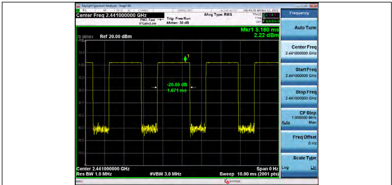
Dwell_Time (Hopping) BT_2-DH1_2441_One_Burst_Time
