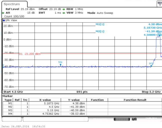
11N20MIMO-Ant1-5180-PASS
