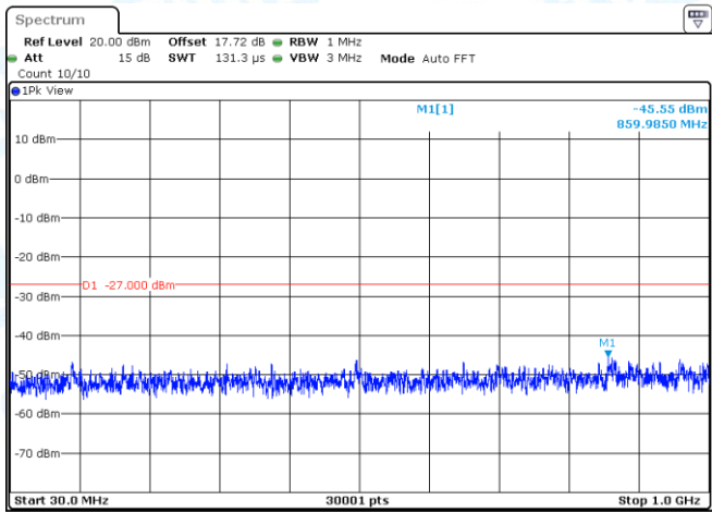
11AC80MIMO-Ant1-5775-30~1000-PASS
