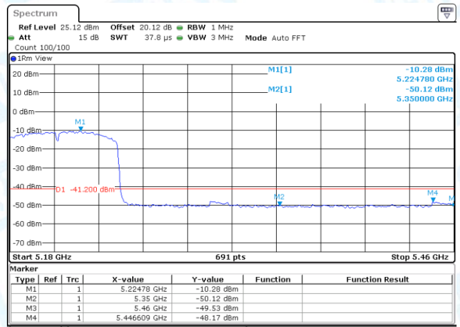
11AC80MIMO-Ant2-5210-PASS
