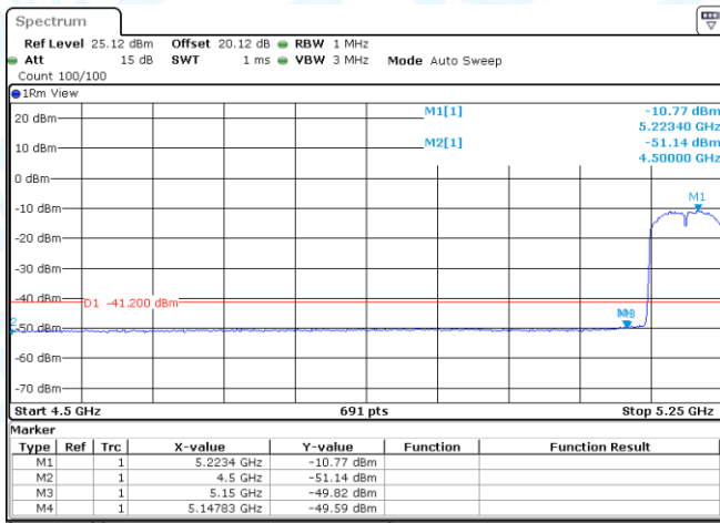
11AC80MIMO-Ant2-5210-PASS
