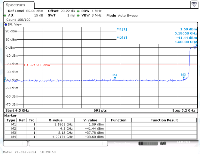
11AC40MIMO-Ant2-5190-PASS
