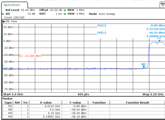
11AC80MIMO-Ant1-5210-PASS
