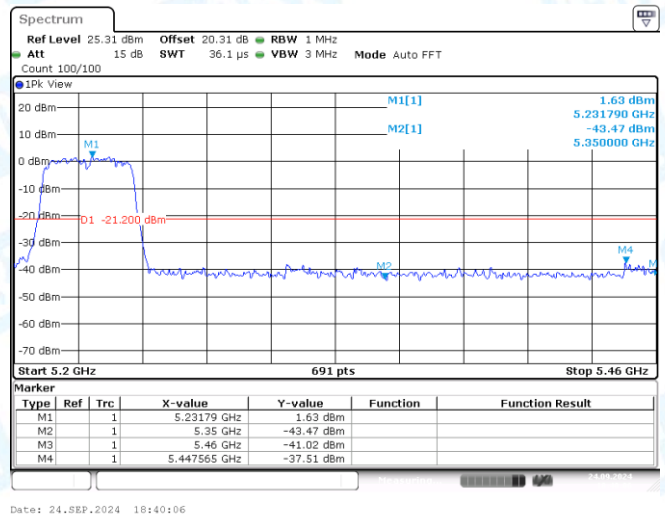
11AC40MIMO-Ant2-5230-PASS
