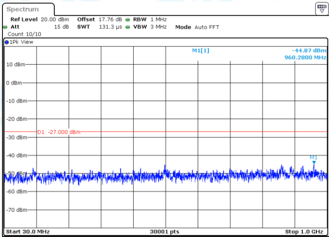
11AC80MIMO-Ant2-5775-30~1000-PASS
