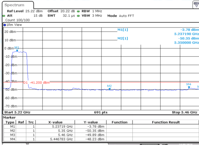
11AC20MIMO-Ant1-5240-PASS
