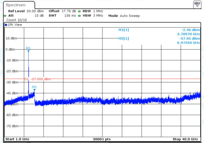
11AC40MIMO-Ant2-5795-1000~40000-PASS
