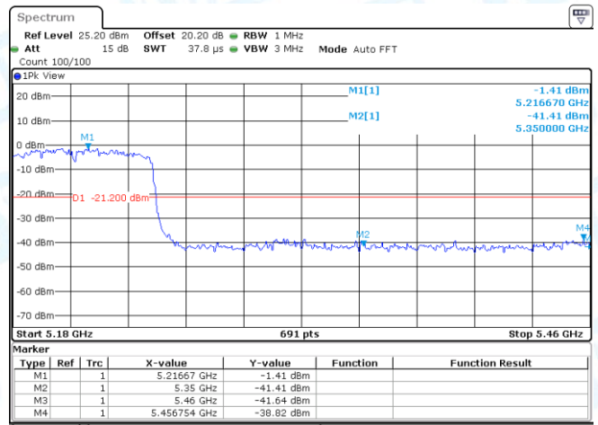
11AC80MIMO-Ant1-5210-PASS
