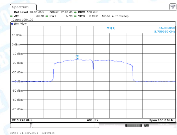
11AC80MIMO-Ant2-5775-PASS
