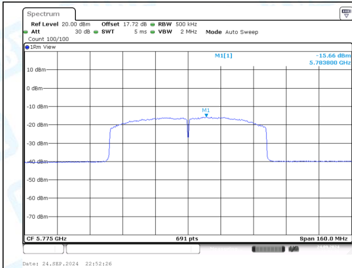
11AC80MIMO-Ant1-5775-PASS
