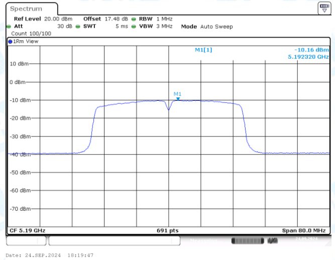
11AC40MIMO-Ant2-5190-PASS
