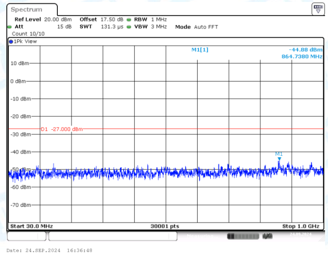
11A-CDD-Ant2-5180-30~1000-PASS
