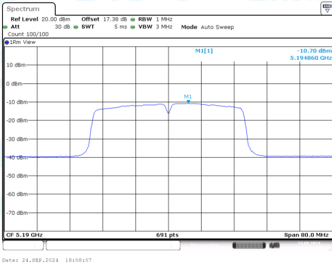
11AC40MIMO-Ant1-5190-PASS
