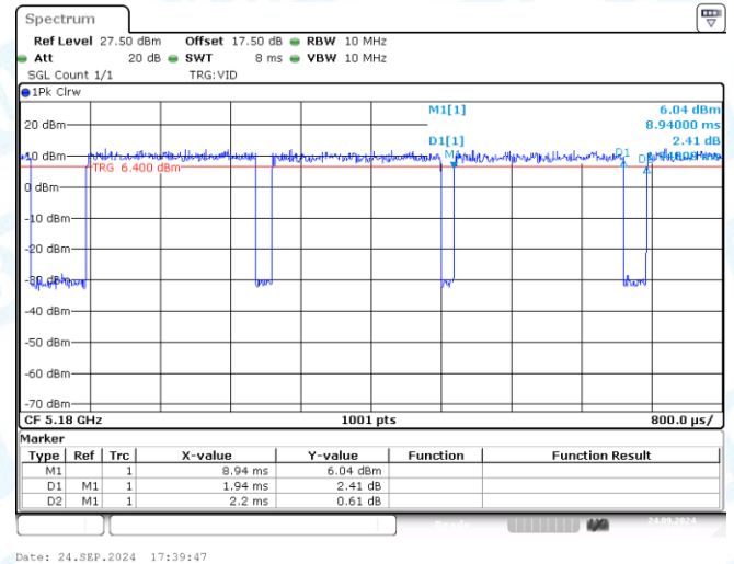
NTNV-11AC20MIMO-Ant2-5180
