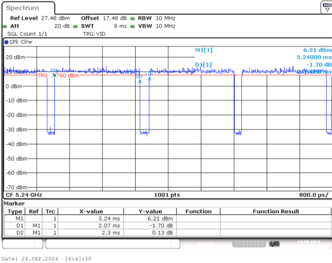
NTNV-11A-CDD-Ant1-5240
