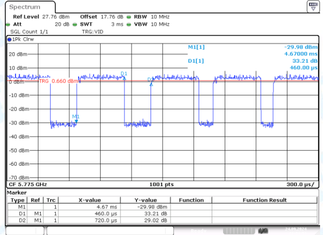
NTNV-11AC80MIMO-Ant2-5775
