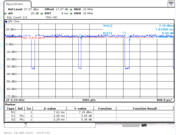
NTNV-11A-CDD-Ant2-5240
