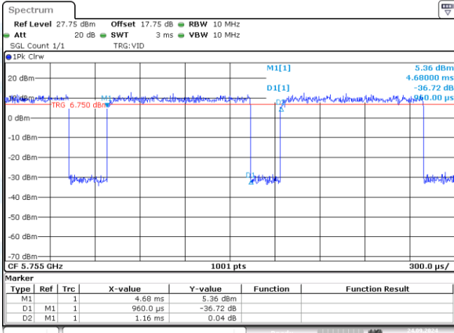
NTVN-11AC40MIMO-Ant1-5755
