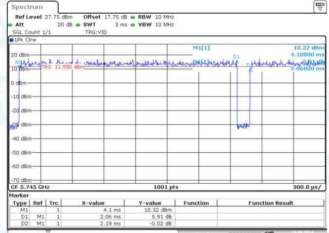
NTNV-11A-CDD-Ant2-5745
