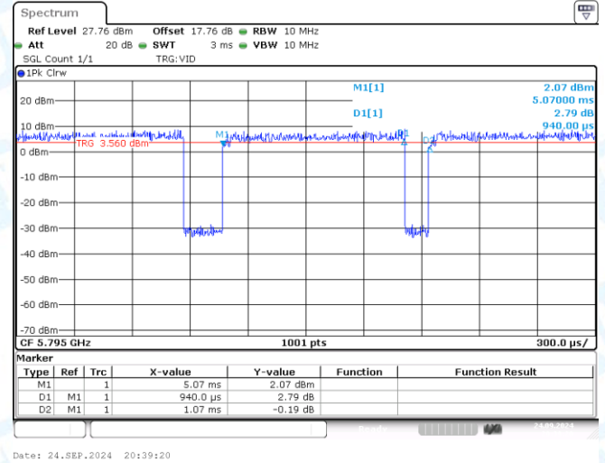
NTNV-11N40MIMO-Ant2-5795
