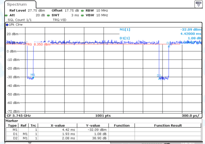
NTNV-11N20MIMO-Ant2-5745
