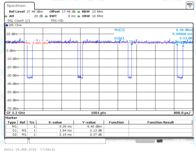
NTNV-11AC20MIMO-Ant2-5200
