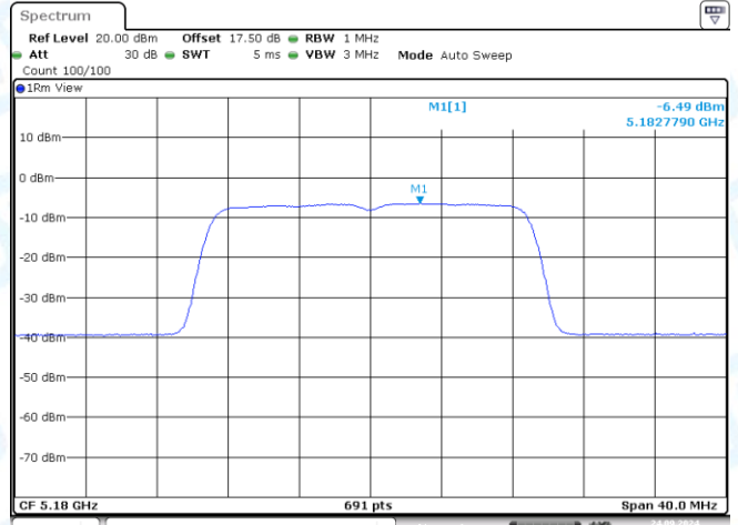
11N20MIMO-Ant2-5180-PASS
