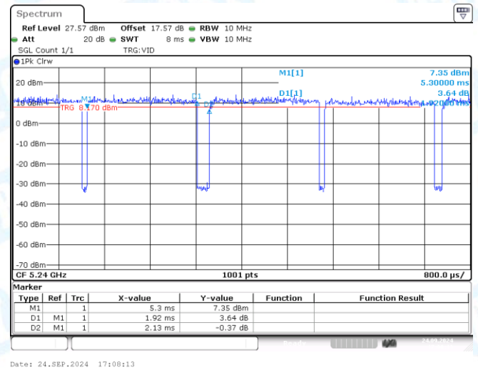
NTNV-11N20MIMO-Ant2-5240
