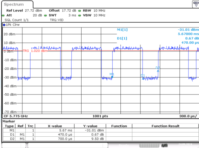
NTNV-11AC80MIMO-Ant1-5775
