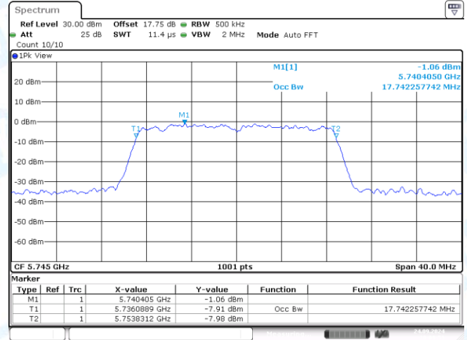
11N20MIMO-Ant2-5745
