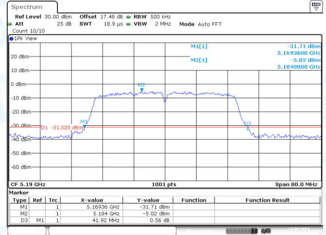
11N40MIMO-Ant2-5190
