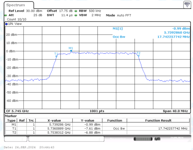
11AC20MIMO-Ant2-5745
