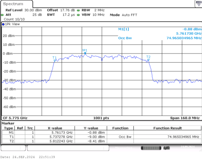
11AC80MIMO-Ant2-5775
