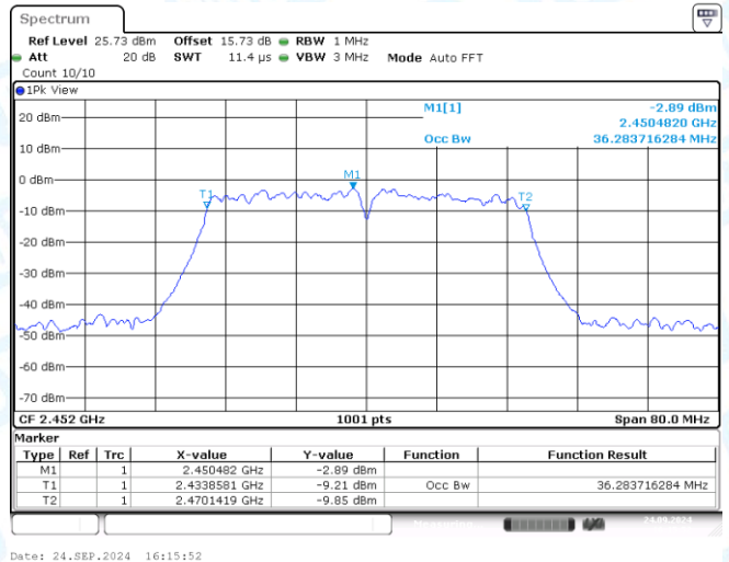
11N40MIMO-Ant2-2452
