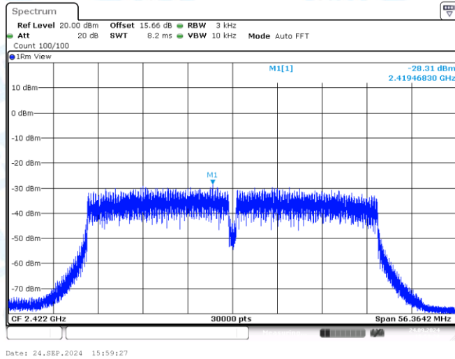
11N40MIMO-Ant1-2422-PASS
