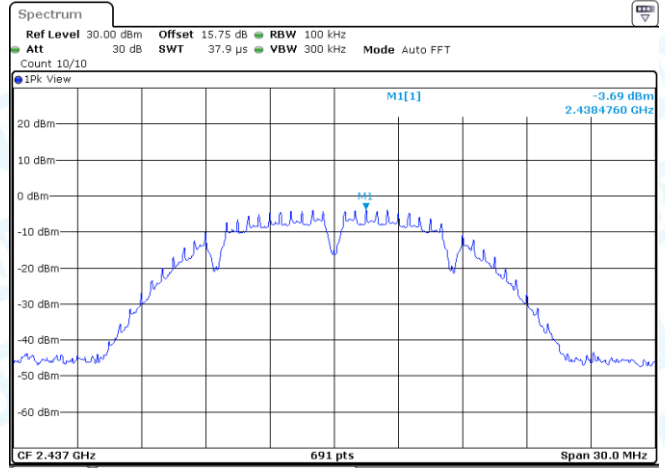
11B-CDD-Ant2-2437-0~Reference-PASS
