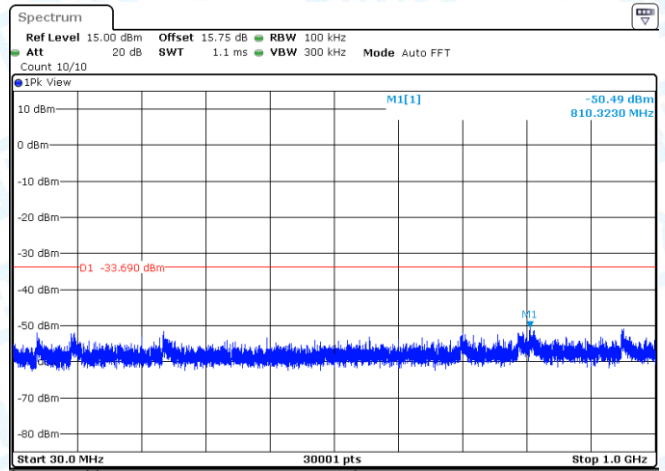
11B-CDD-Ant2-2437-0~Reference-PASS
