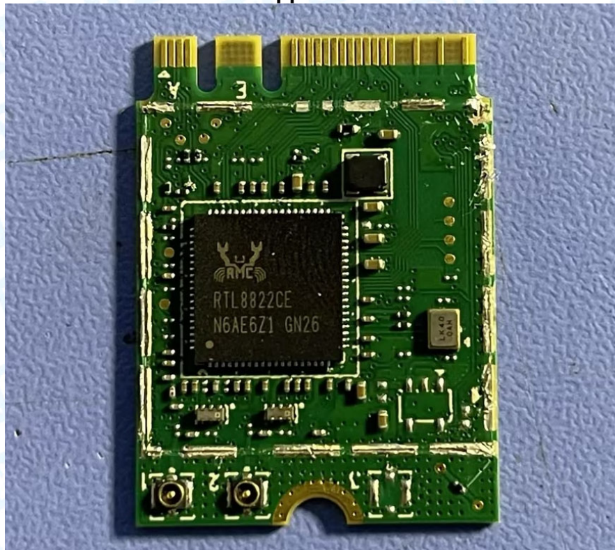
Photo 22 Appearance of PCB
