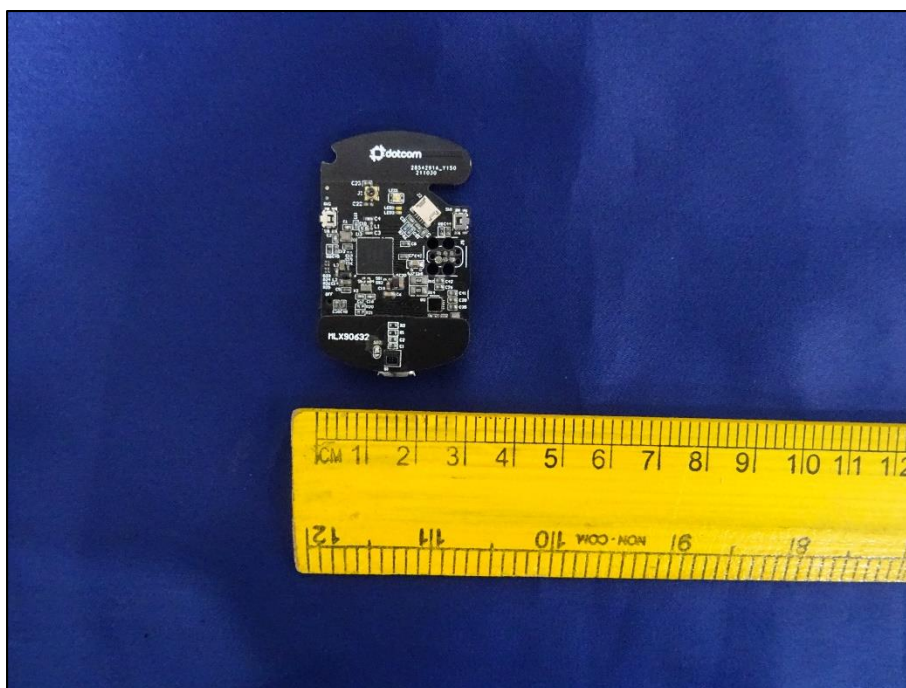
Figure 4: Dimensional view of PCB
