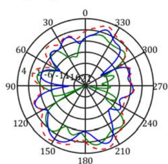
frequency=2450MHz, X-Y Plane
