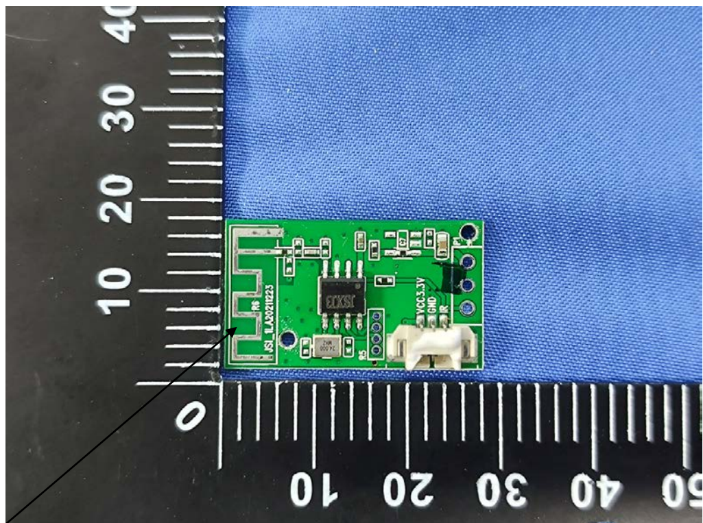
EUT View
