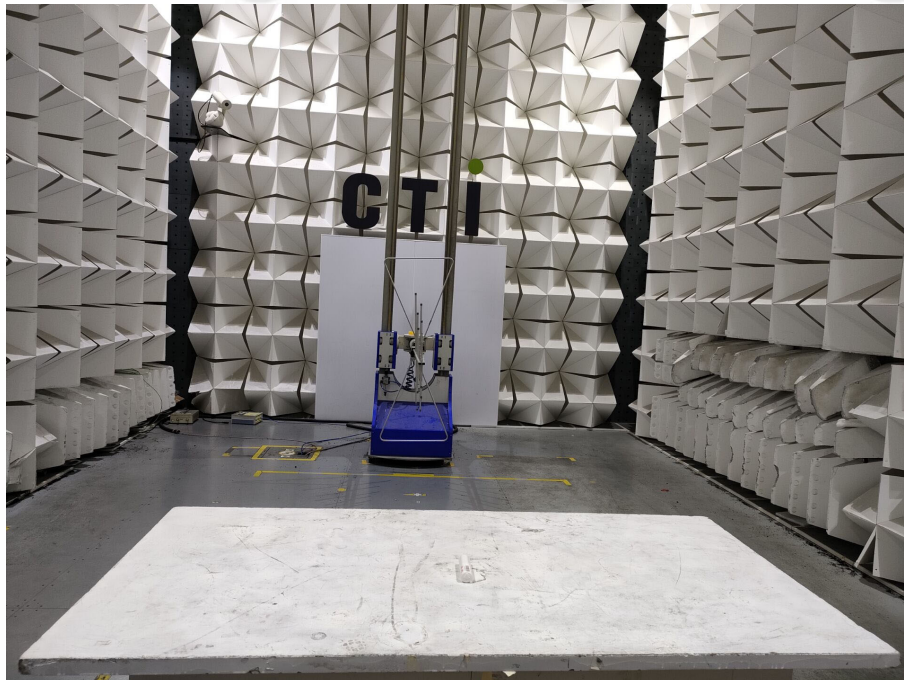
Radiated spurious emission Test Setup-1(Below 1GHz) (small)
