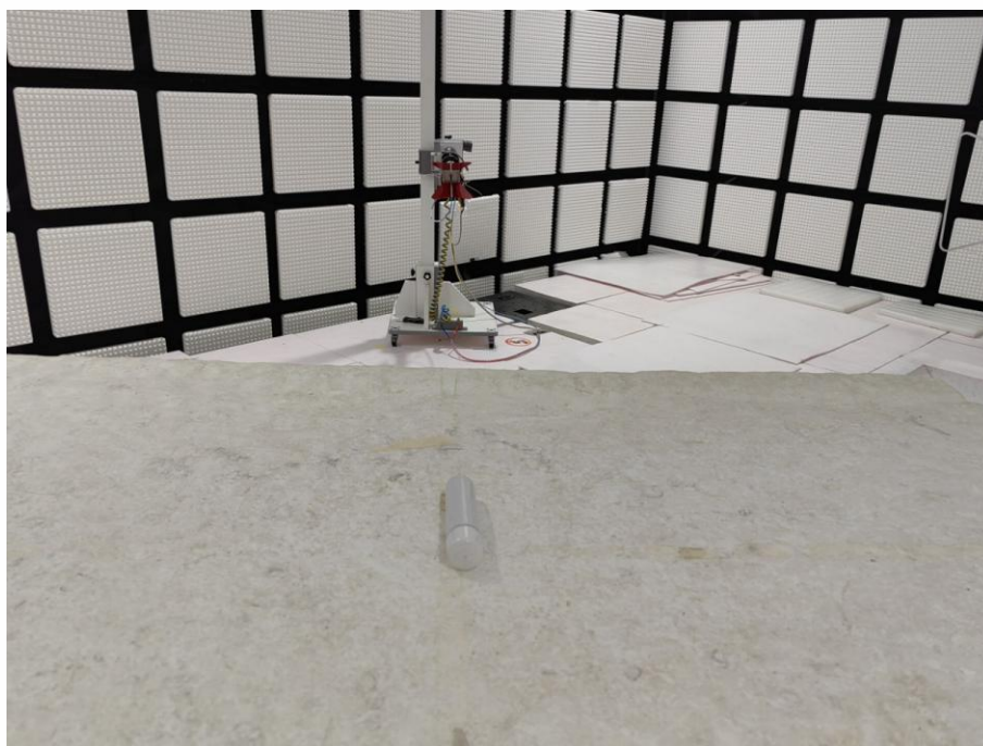
Radiated spurious emission Test Setup-6(Above 1GHz)(big)
