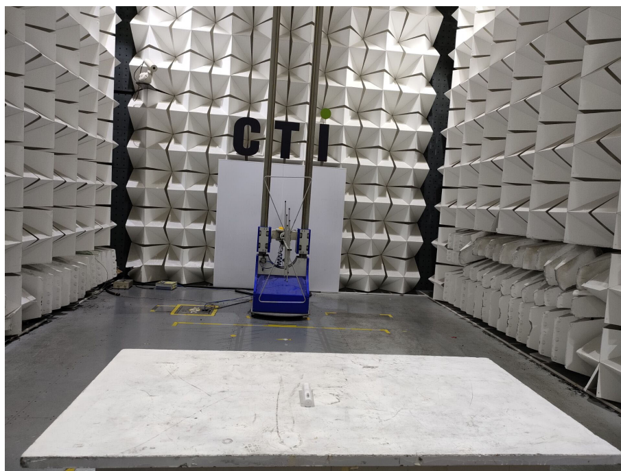
Radiated spurious emission Test Setup-3(Below 1GHz) (big)
