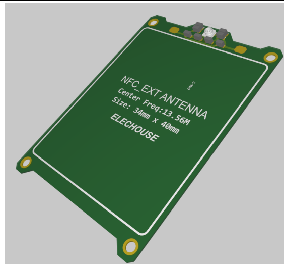
CAD 3D view
