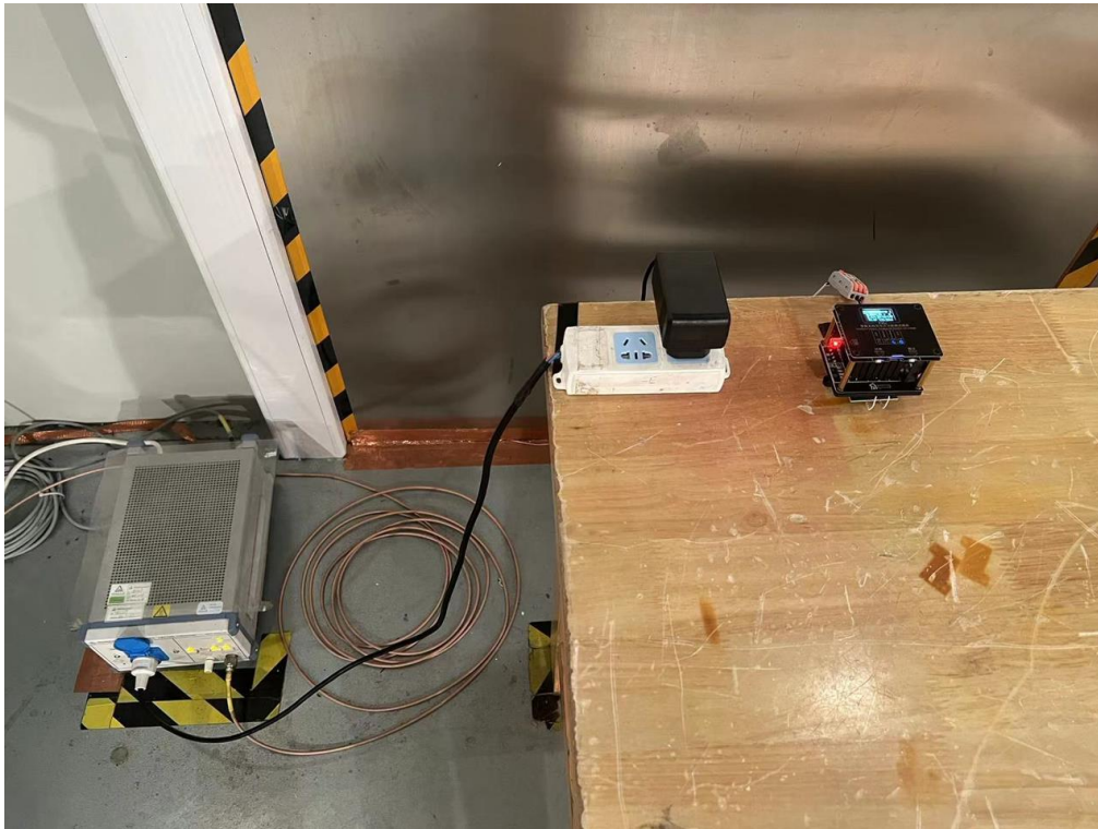
Conducted emission 150KHz-30MHz
