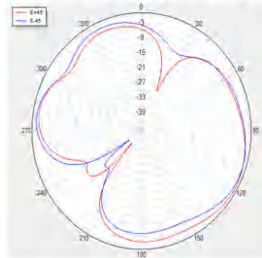
H Theta=90 freq=2450MHz
