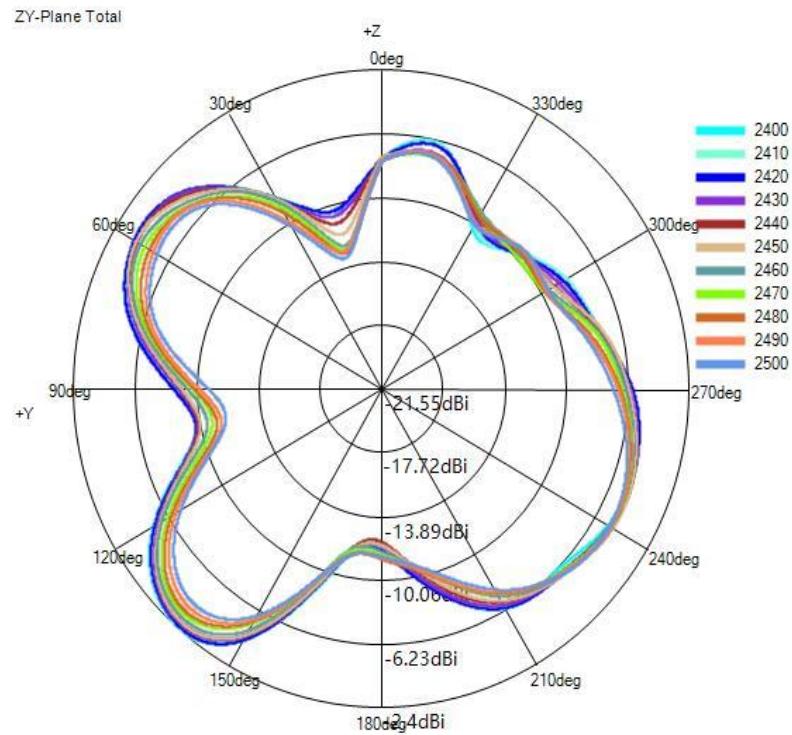
(2) Y-Z Plane(unit:dBi):
