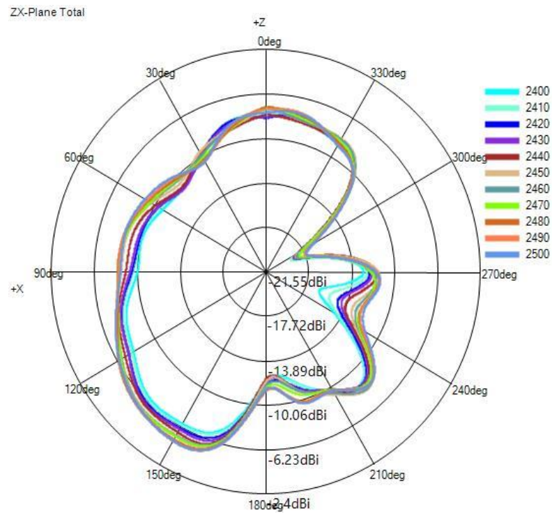
(1) X-Z Plane(unit:dBi):
