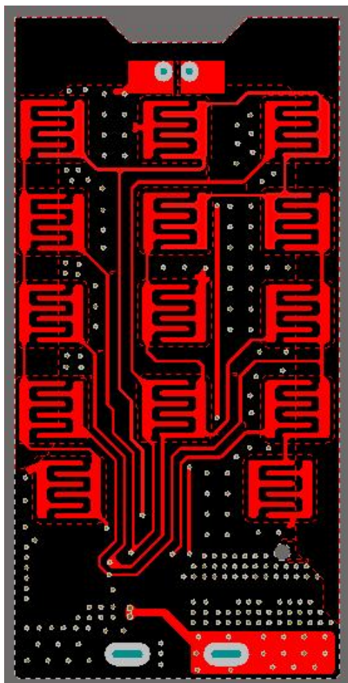
遥控器 PCB 顶层 (Top layer of remote control PCB)
