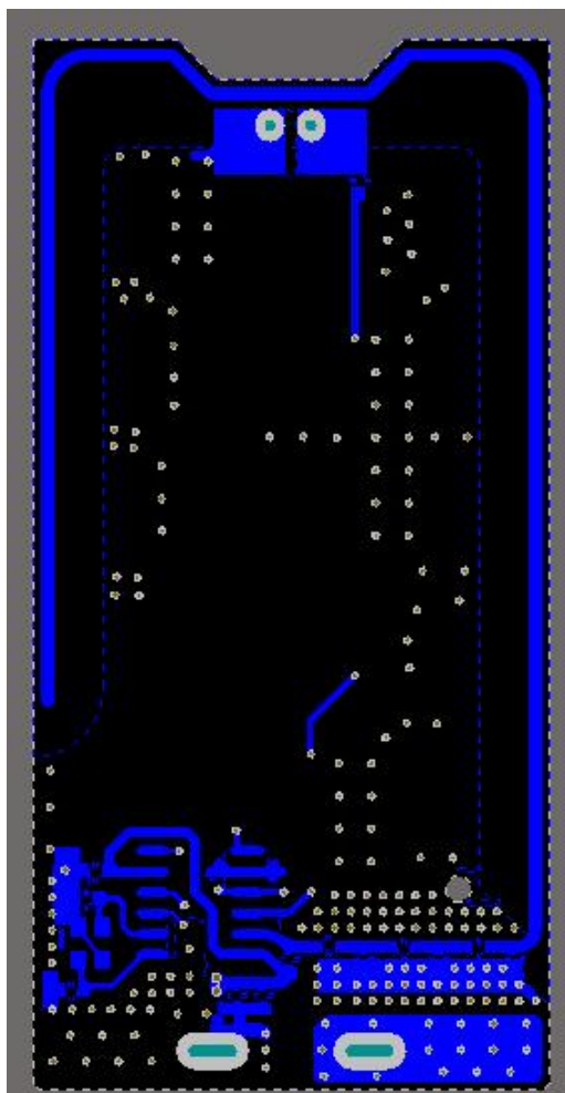
遥控器 PCB 底层 (Bottom layer of remote control PCB)
