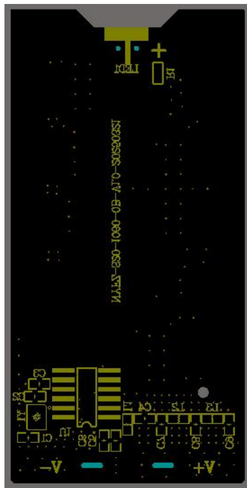
遥控器丝印层 (Remote control screen printing layer)
