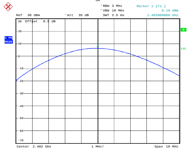
2DH1_Low
