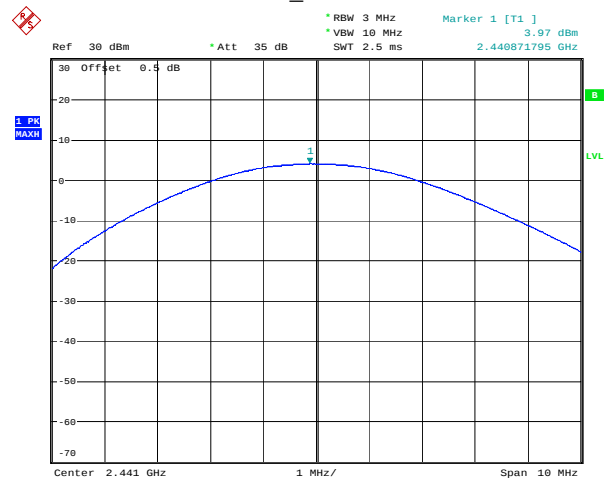
DH1_Middle
