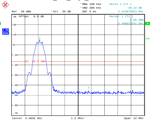
BLE_1M_High_Channel
