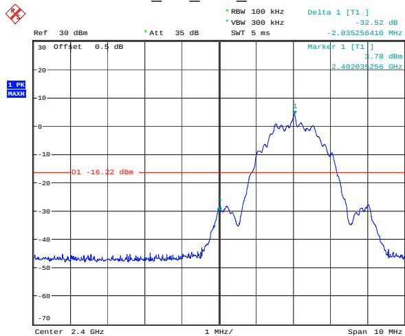
BLE_2M_Low_Channel
