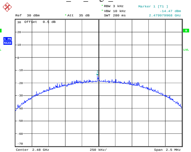
BLE_2M_High_Channel
