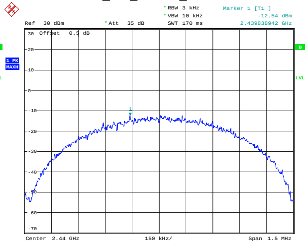
BLE_1M_Middle_Channel
