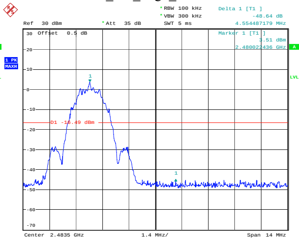
BLE_2M_High_Channel
