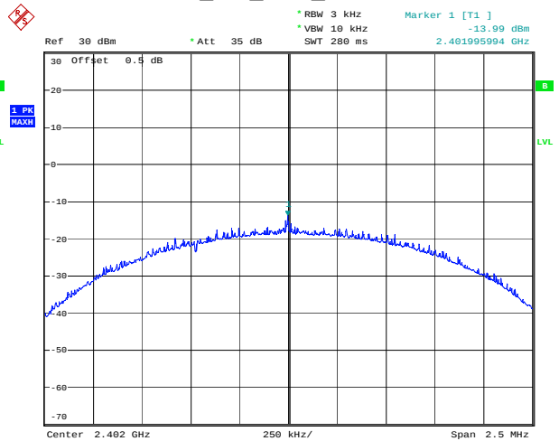
BLE_2M_Low_Channel
