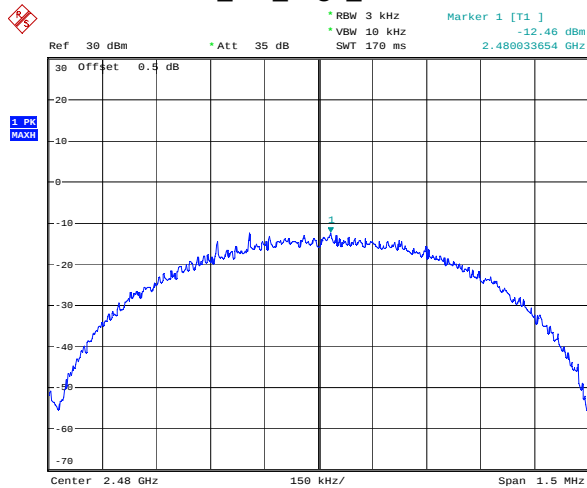
BLE_1M_High_Channel
