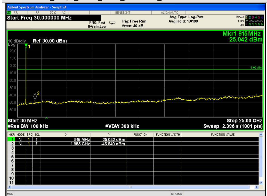
Test Graph GFSK ANT1 915.0MHz Medium Band Emissions
