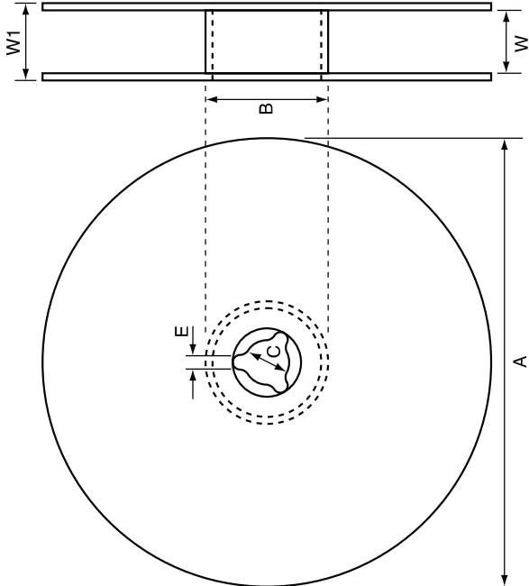
Figure 22: Reel Dimensions
