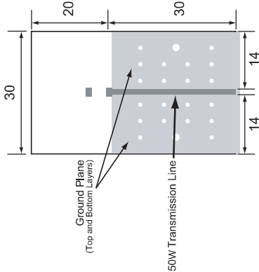
Figure 15: 2.4GHz Test Board
