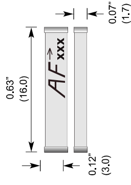
Figure 2: 868MHz and 916MHz Dimensions
