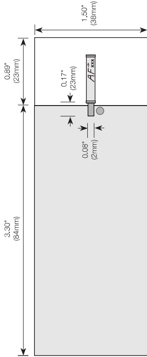
Figure 16: 868MHz and 916MHz Test Board
