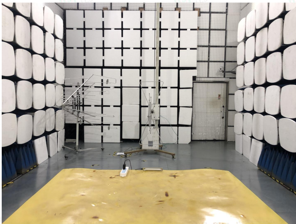
Radiated Emission from 30MHz to 1GHz
