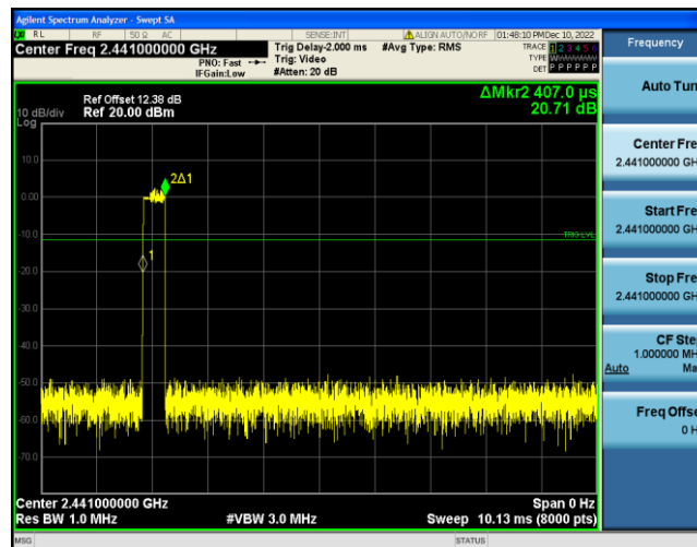
3DH3-Ant1-Hop-1.658-160
