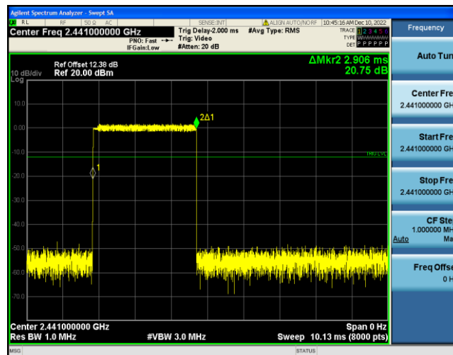
2DH1-Ant1-Hop-0.405-320
