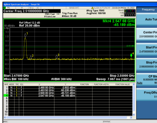
3DH5-Ant1-High-2480--2.50
