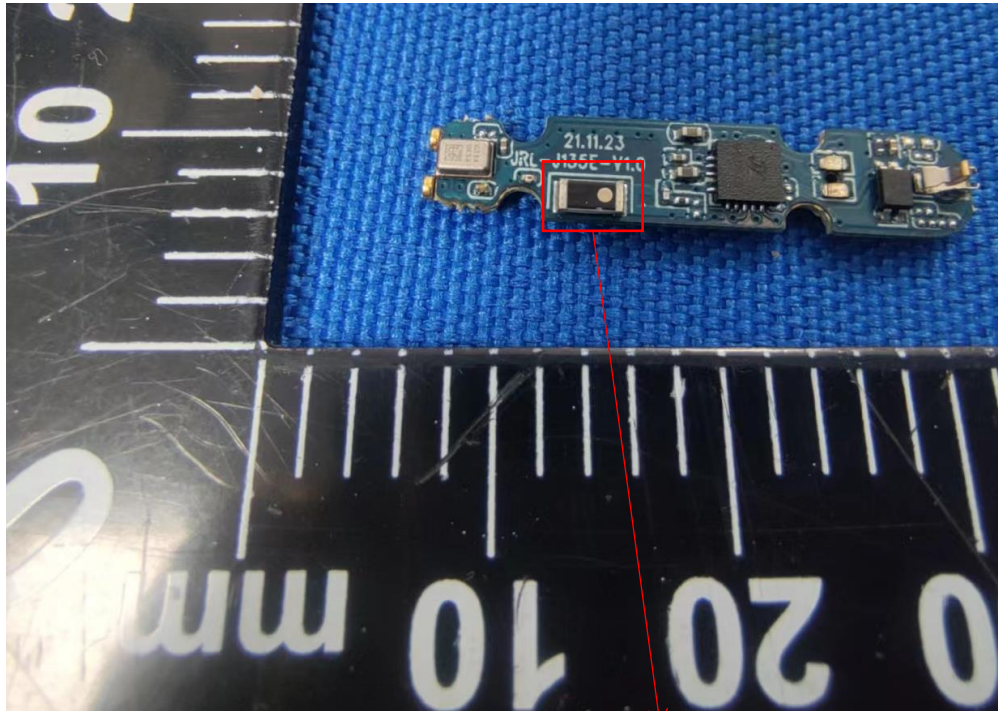
Chip antenna
