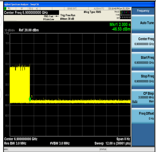
11AX160SISO-Ant2-6825-Center-6900-OFF-PASS
