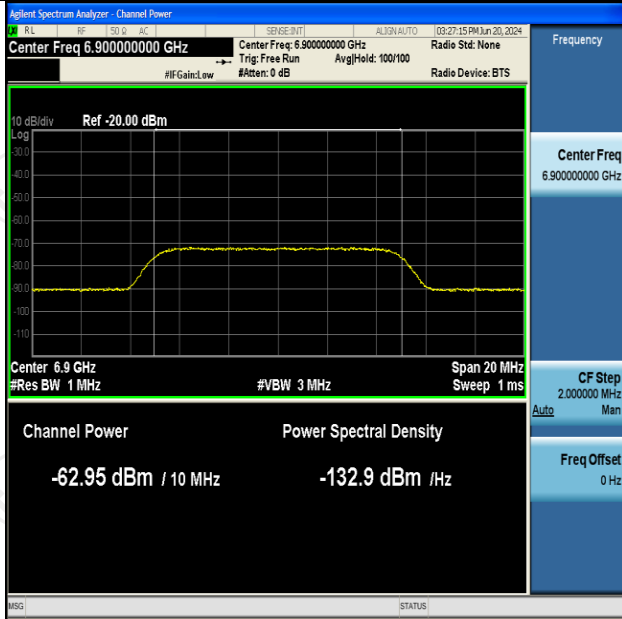
11AX160SISO-Ant2-6825-Center-6900-Minimal
