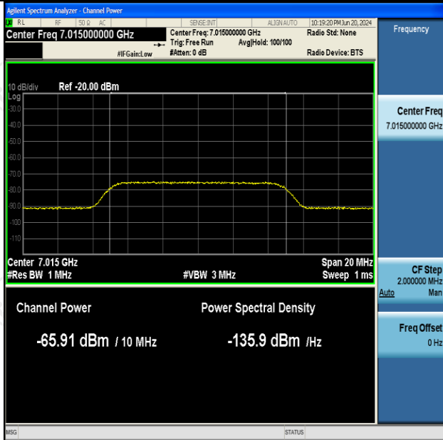
11AX20SISO-Ant2-7015-Center-7015-OFF-PASS
