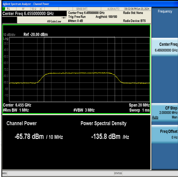
11AX20SISO-Ant2-6455-Center-6455-Minimal
