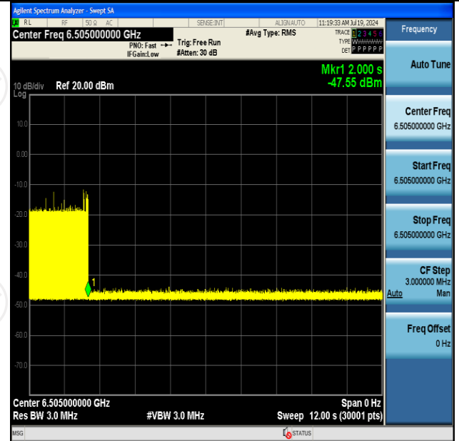
11AX160SISO-Ant2-6505-Center-6505-OFF-PASS
