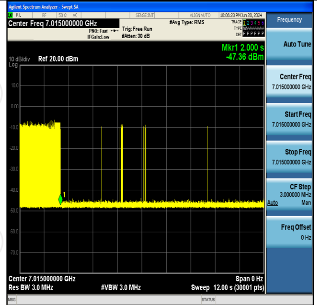
11AX20SISO-Ant2-7015-Center-7015-Minimal
