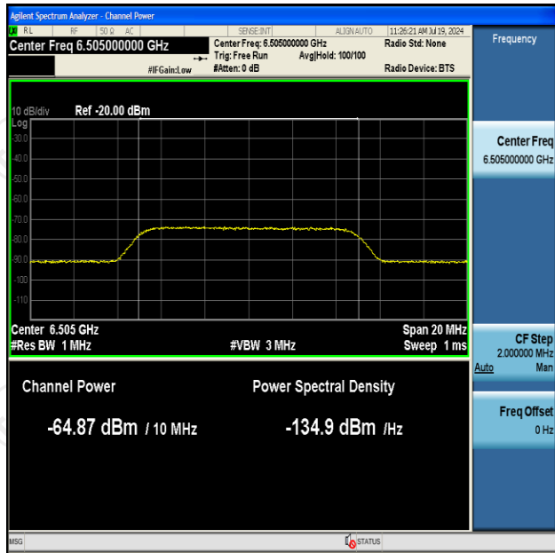
11AX160SISO-Ant2-6505-Center-6505-Minimal
