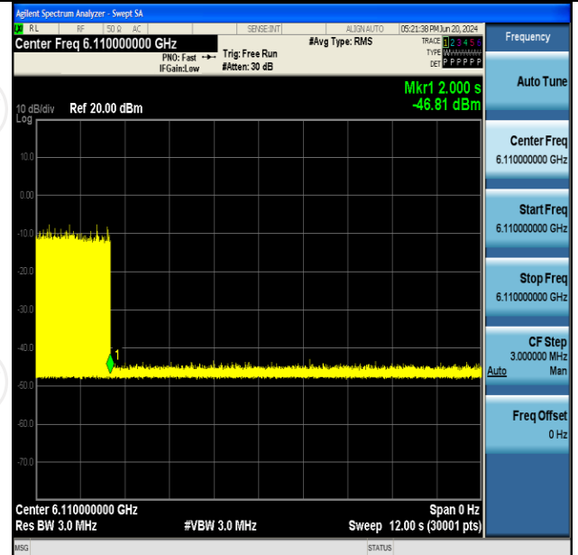
11AX160SISO-Ant2-6185-Low-6110-OFF-PASS
