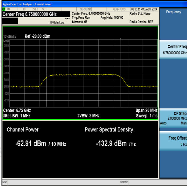
11AX160SISO-Ant2-6825-Low-6750-Minimal
