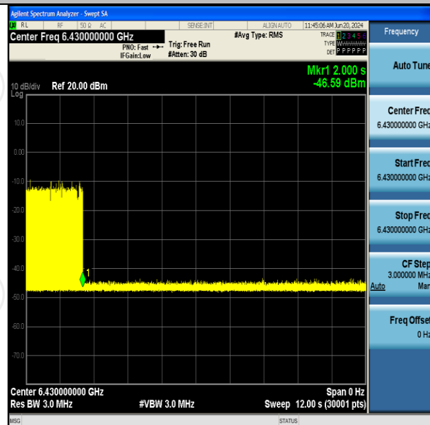
11AX160SISO-Ant2-6505-Low-6430-OFF-PASS
