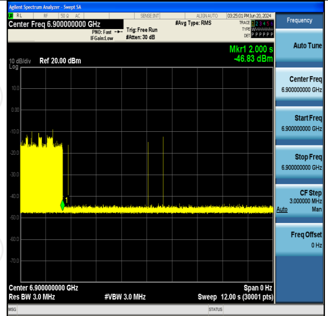
11AX160SISO-Ant2-6825-Center-6900-Minimal
