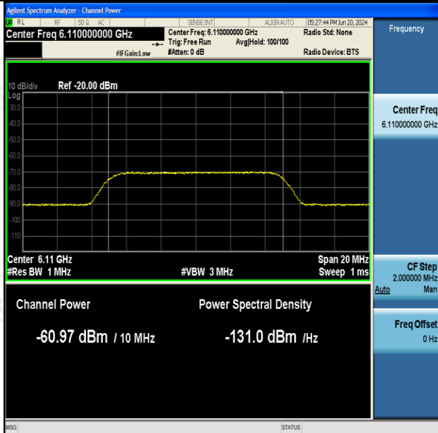
11AX160SISO-Ant2-6185-Low-6110-OFF-PASS
