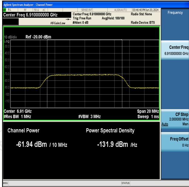
11AX160SISO-Ant2-6985-Low-6910-Minimal
