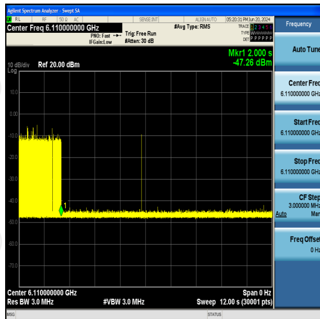
11AX160SISO-Ant2-6185-Low-6110-Minimal
