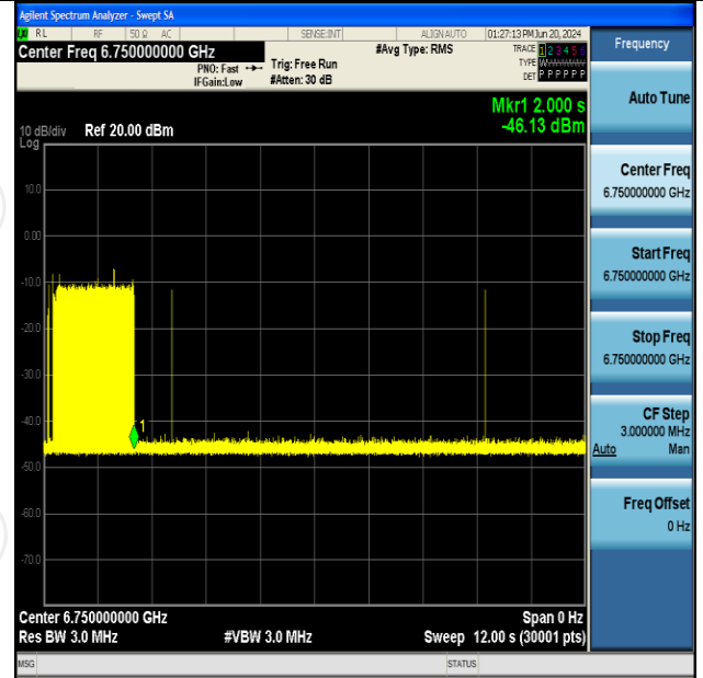
11AX160SISO-Ant2-6825-Low-6750-Minimal
