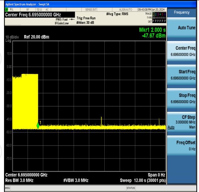
11AX20SISO-Ant2-6695-Center-6695-Minimal
