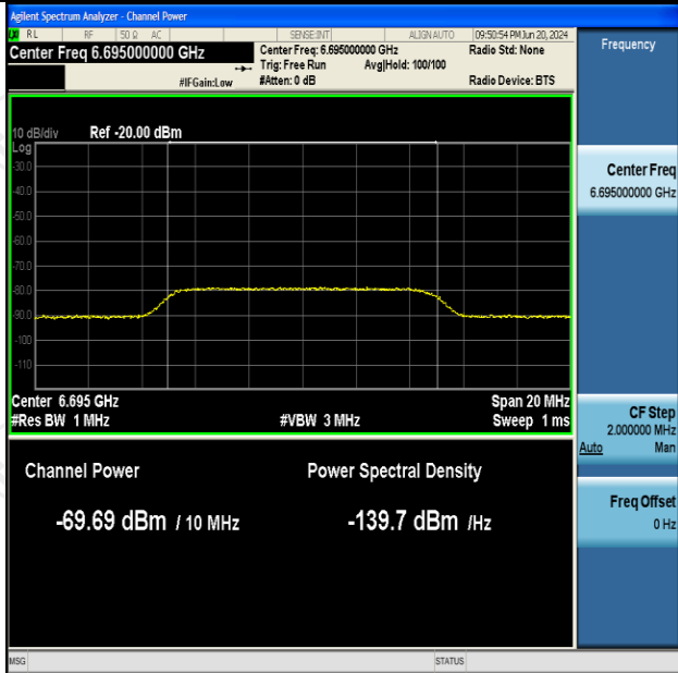
11AX20SISO-Ant2-6695-Center-6695-OFF-PASS
