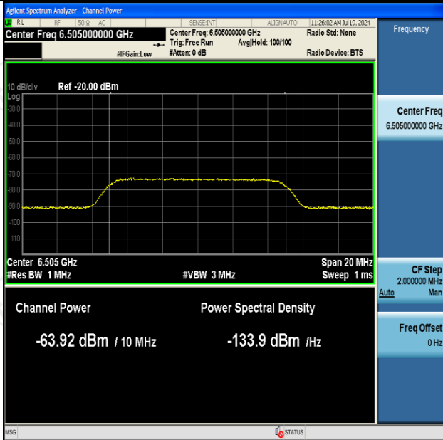
11AX160SISO-Ant2-6505-Center-6505-OFF-PASS
