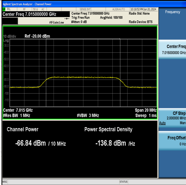
11AX20SISO-Ant2-7015-Center-7015-Minimal
