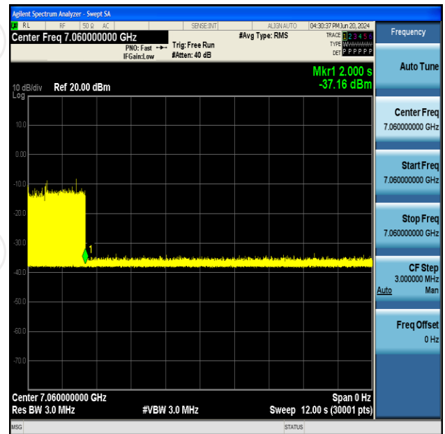
11AX160SISO-Ant2-6985-High-7060-OFF-PASS
