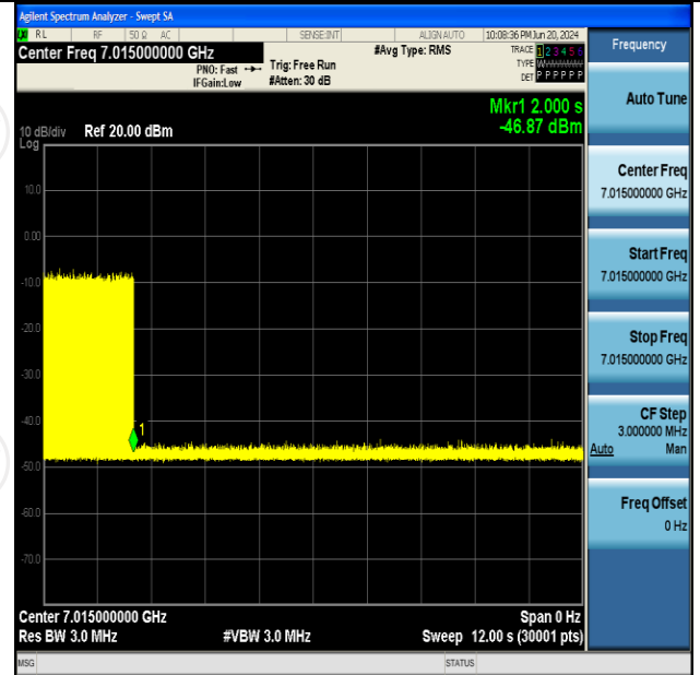
11AX20SISO-Ant2-7015-Center-7015-OFF-PASS
