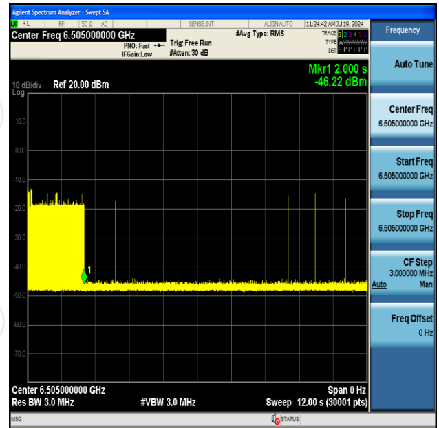
11AX160SISO-Ant2-6505-Center-6505-Minimal
