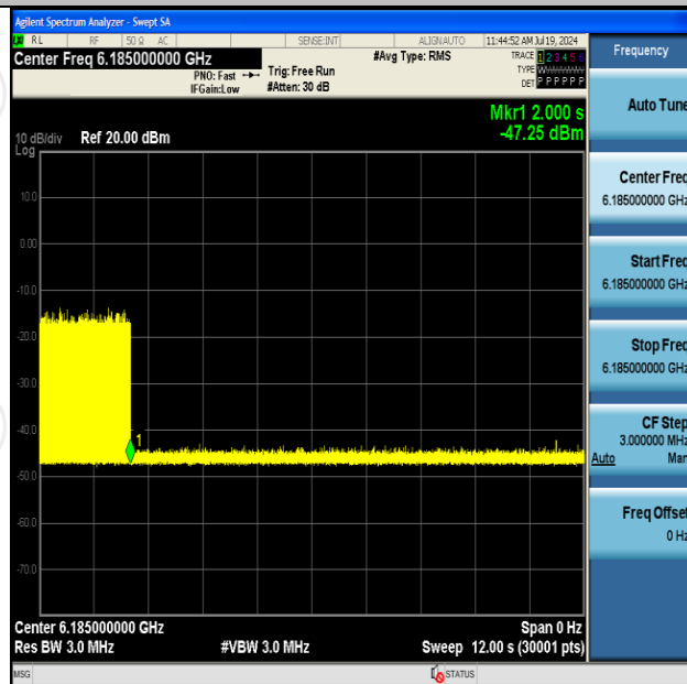
11AX160SISO-Ant2-6185-Center-6185-OFF-PASS
