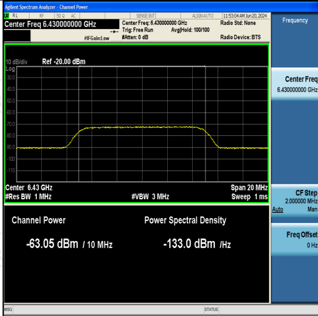
11AX160SISO-Ant2-6505-Low-6430-Minimal
