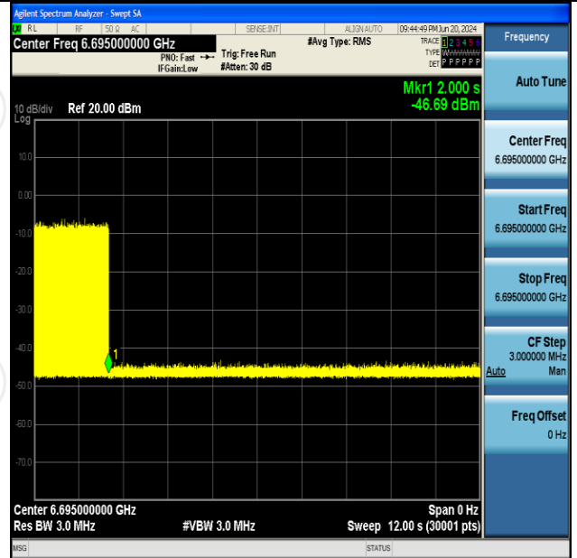
11AX20SISO-Ant2-6695-Center-6695-OFF-PASS
