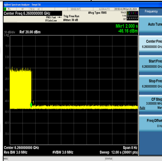
11AX160SISO-Ant2-6185-High-6260-Minimal
