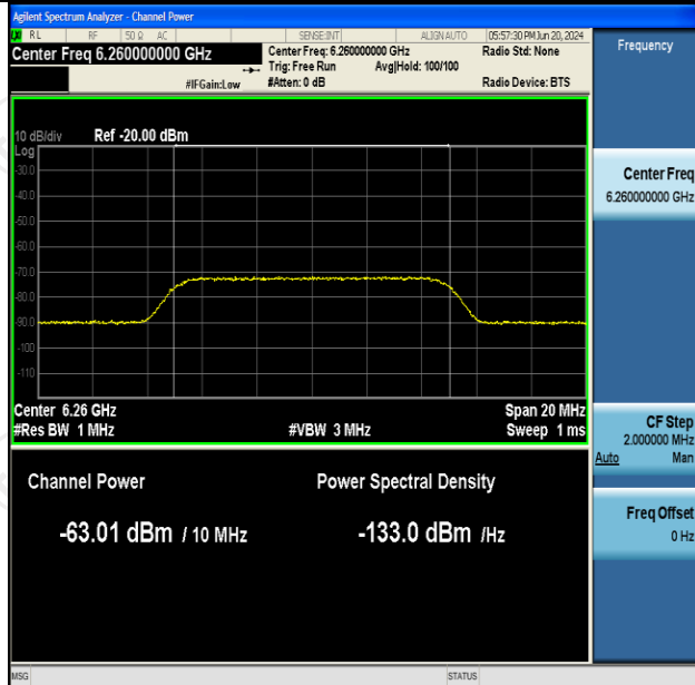
11AX160SISO-Ant2-6185-High-6260-OFF-PASS
