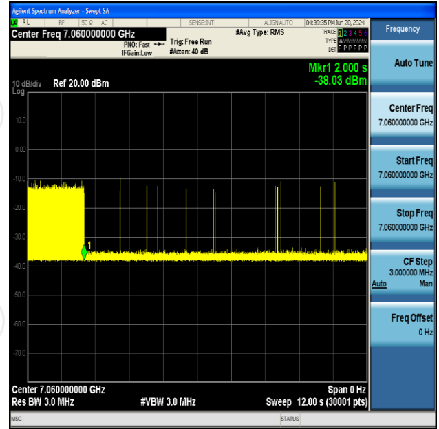
11AX160SISO-Ant2-6985-High-7060-Minimal
