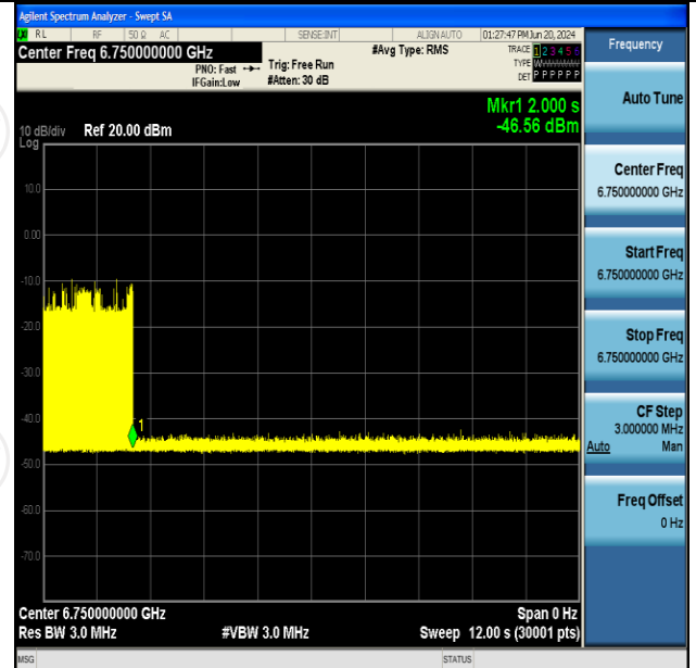
11AX160SISO-Ant2-6825-Low-6750-OFF-PASS
