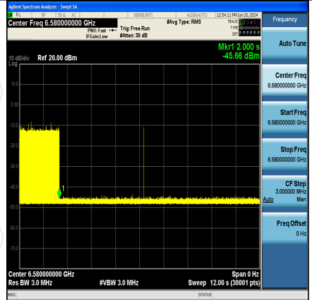
11AX160SISO-Ant2-6505-Center-6580-Minimal
