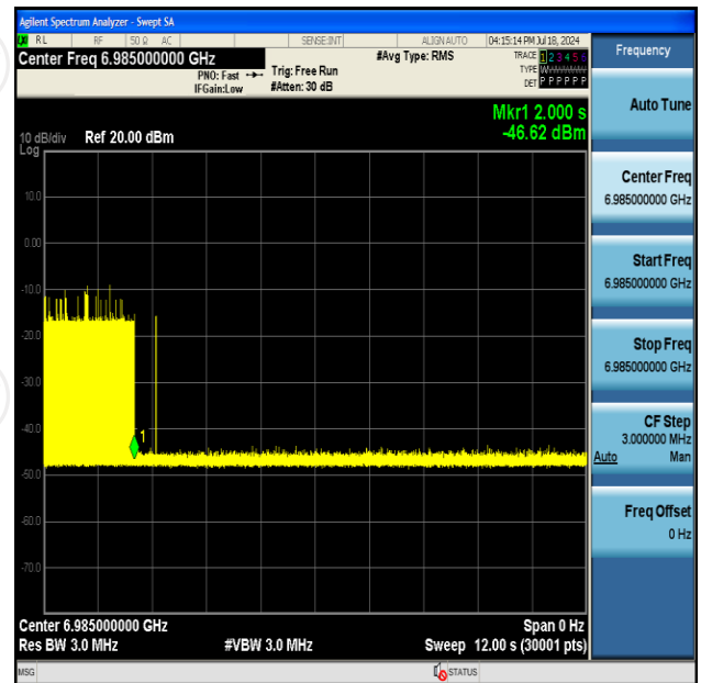
11AX160SISO-Ant2-6985-Center-6985-OFF-PASS
