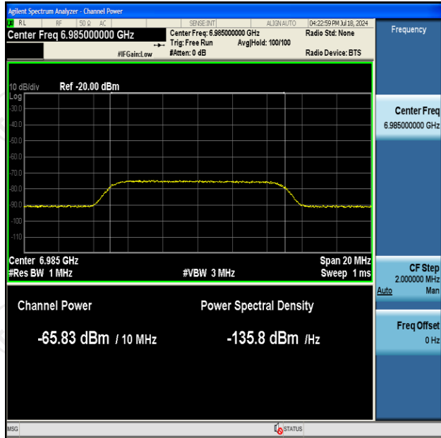
11AX160SISO-Ant2-6985-Center-6985-Minimal
