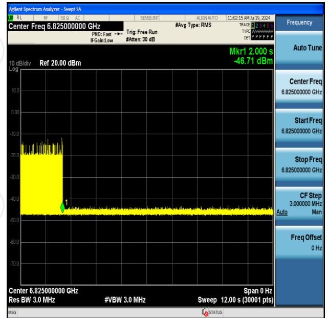
11AX160SISO-Ant2-6825-Center-6825-OFF-PASS
