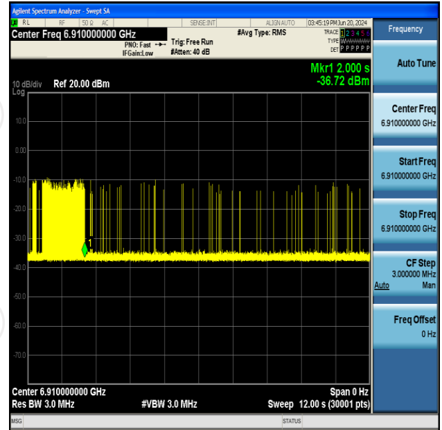
11AX160SISO-Ant2-6985-Low-6910-Minimal
