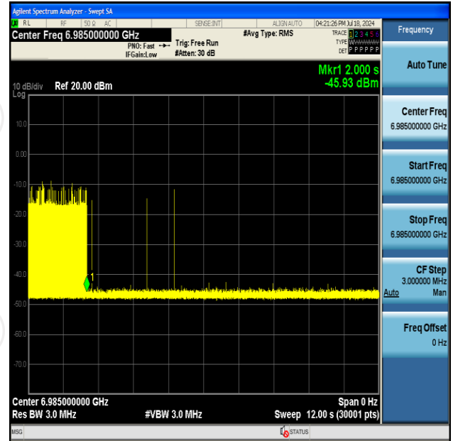
11AX160SISO-Ant2-6985-Center-6985-Minimal
