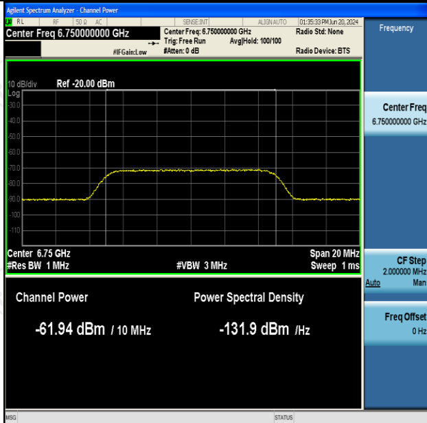
11AX160SISO-Ant2-6825-Low-6750-OFF-PASS
