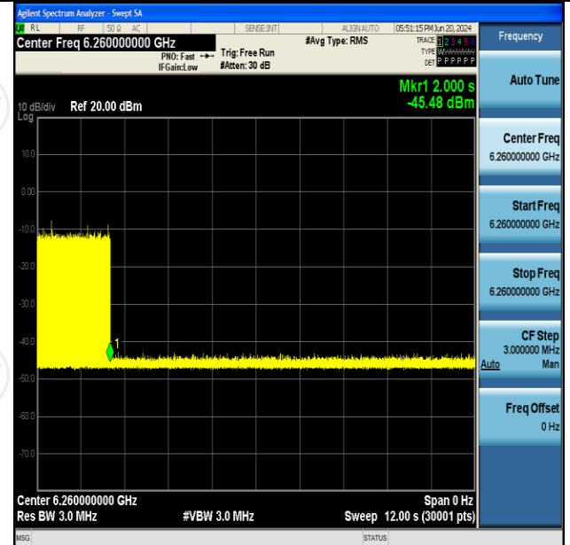
11AX160SISO-Ant2-6185-High-6260-OFF-PASS
