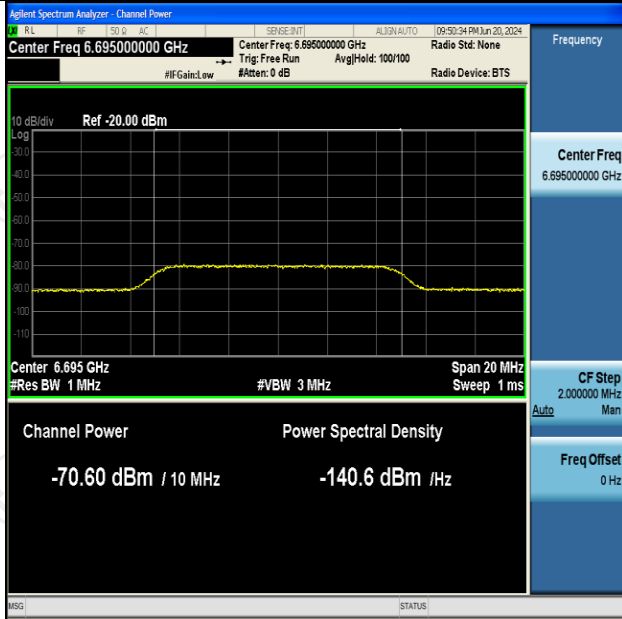
11AX20SISO-Ant2-6695-Center-6695-Minimal
