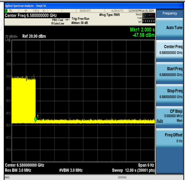
11AX160SISO-Ant2-6505-Center-6580-OFF-PASS
