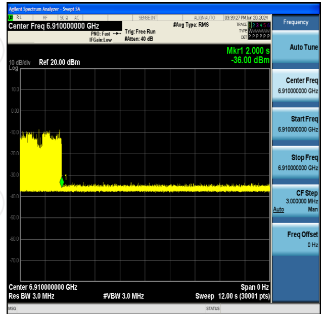
11AX160SISO-Ant2-6985-Low-6910-OFF-PASS
