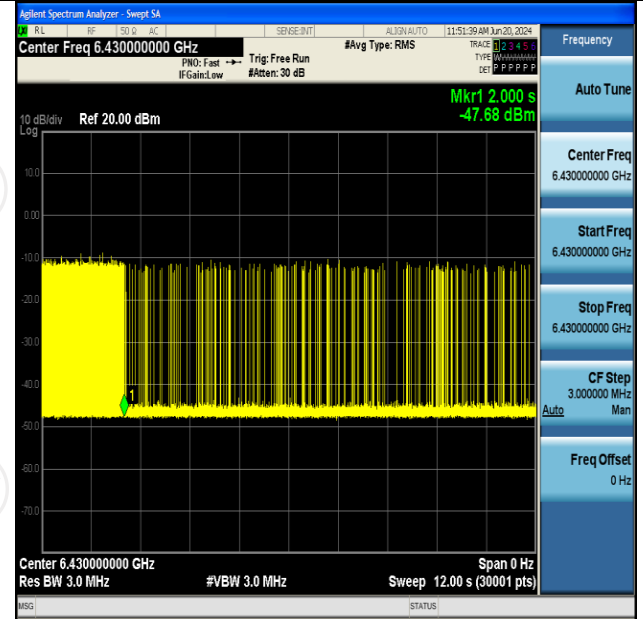
11AX160SISO-Ant2-6505-Low-6430-Minimal
