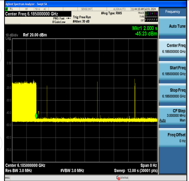
11AX160SISO-Ant2-6185-Center-6185-Minimal
