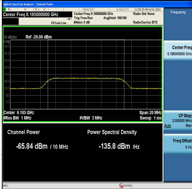
11AX160SISO-Ant2-6185-Center-6185-Minimal
